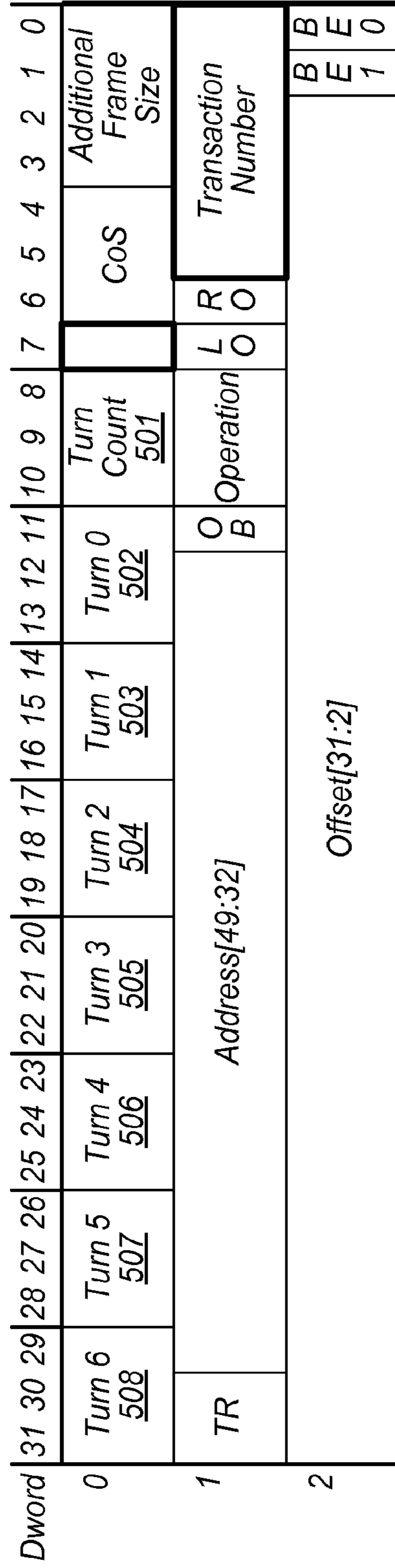
Address Routed Write Frame Format
