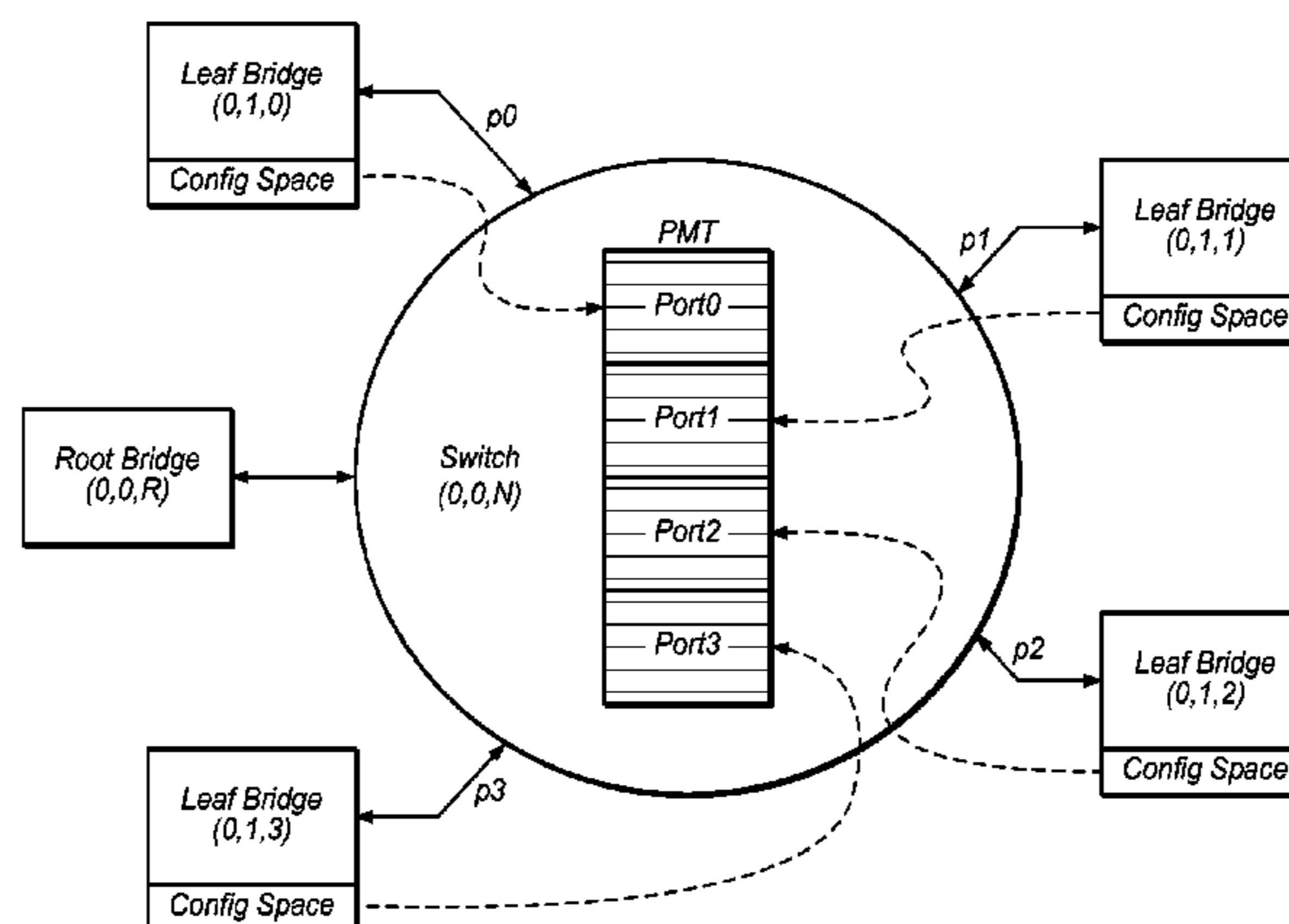
Configuration Space Snooping Into Port Map Table
