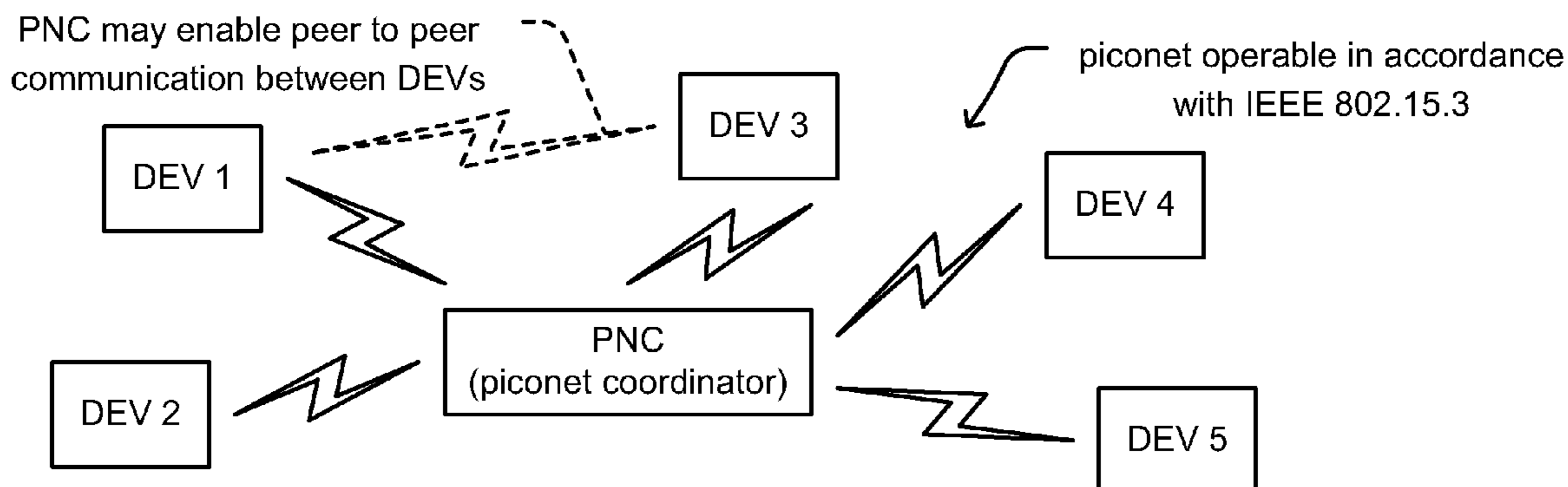
piconet (shown in wireless communication system embodiment)
