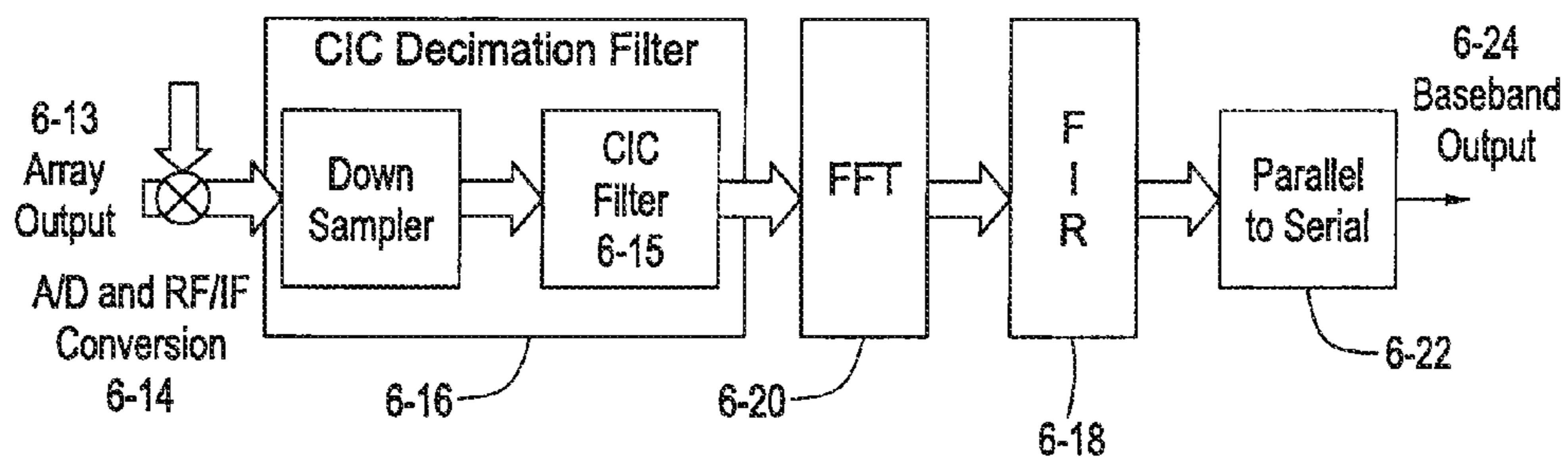
RX Configuration
