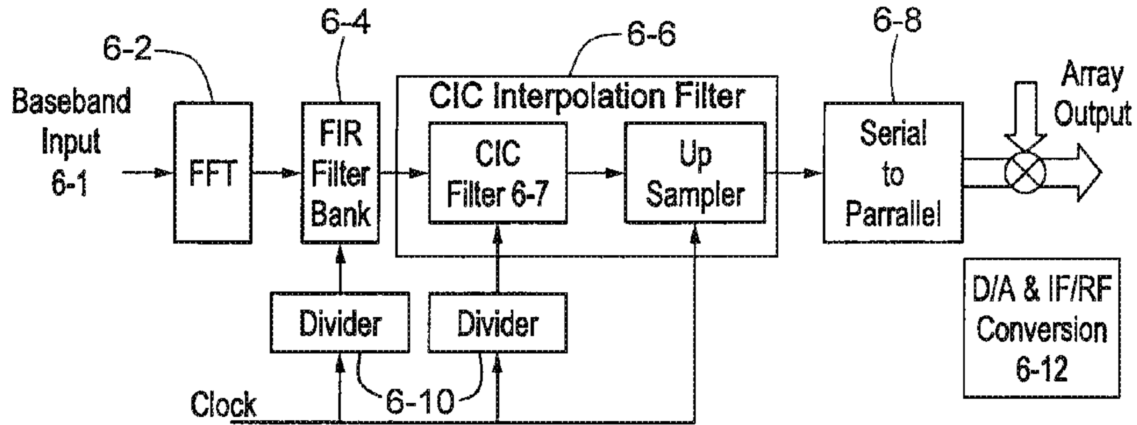
TX Configuration
