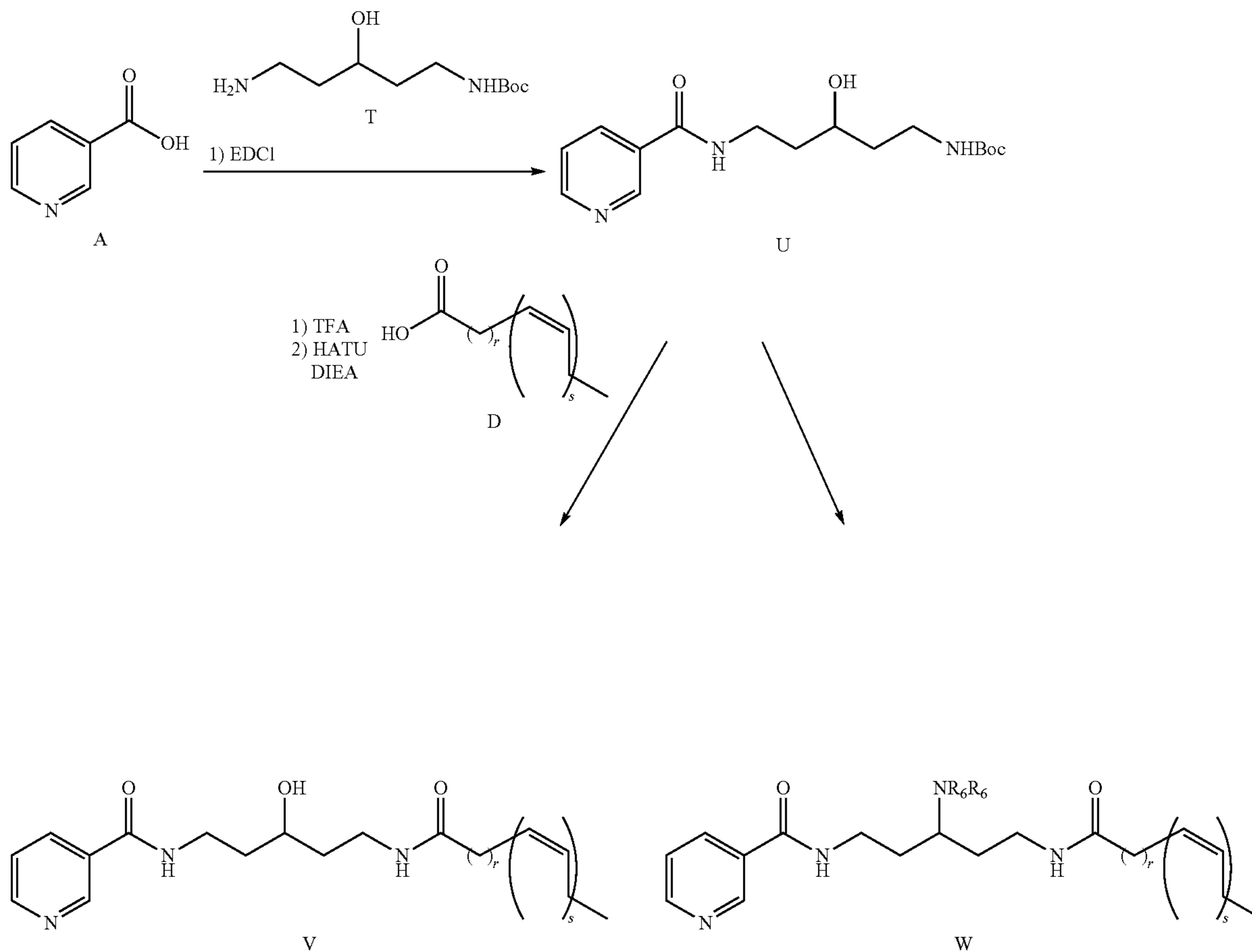
Scheme 6
