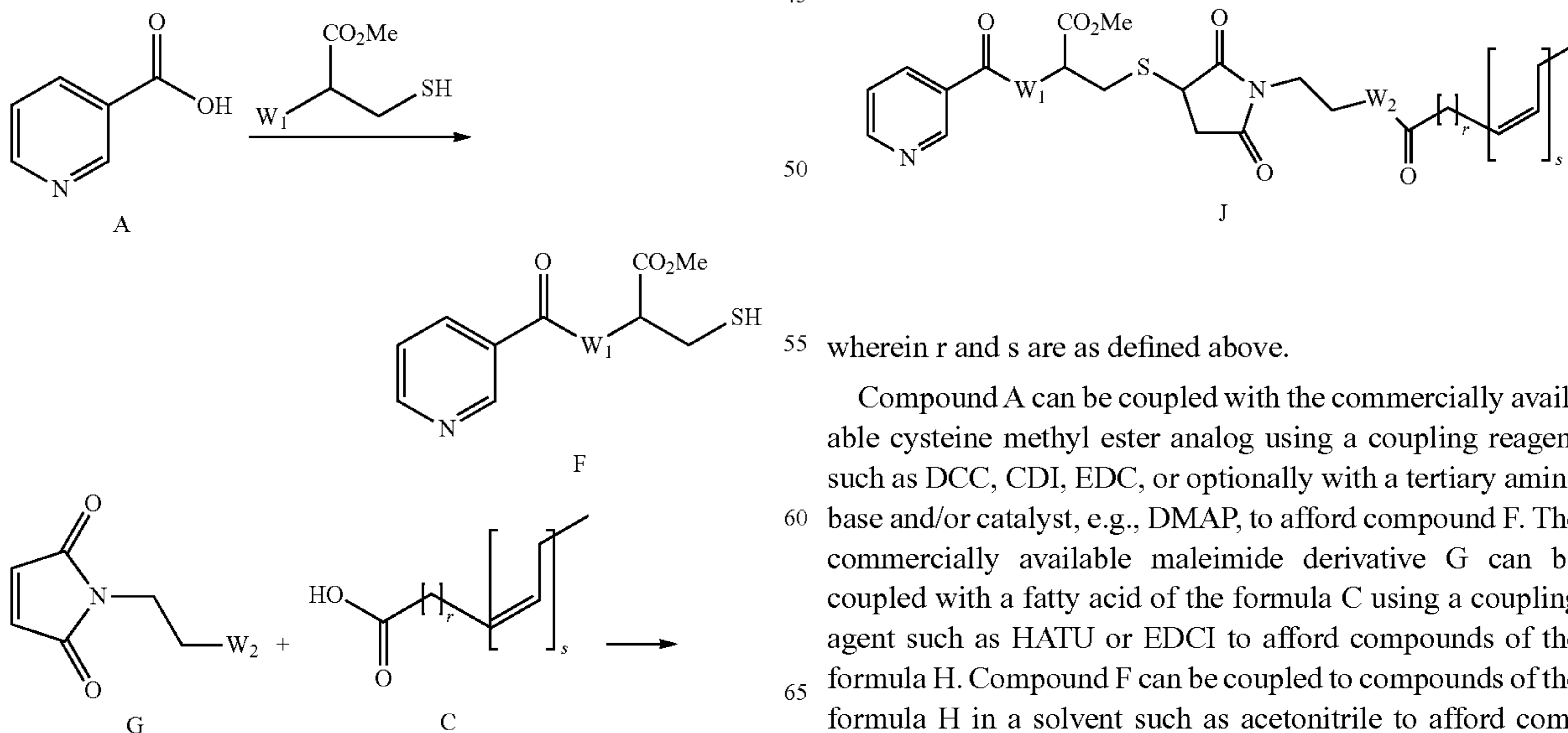
Scheme 12
