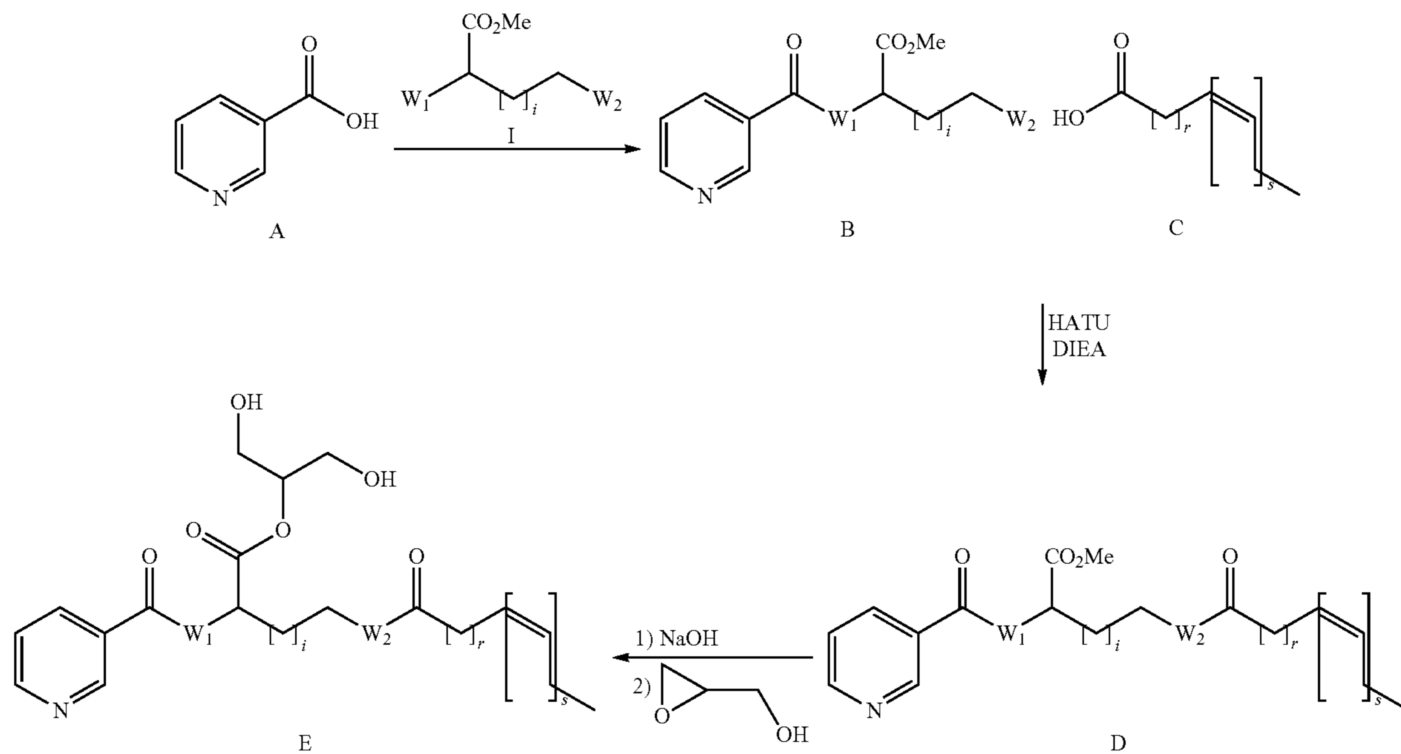
Scheme 11
