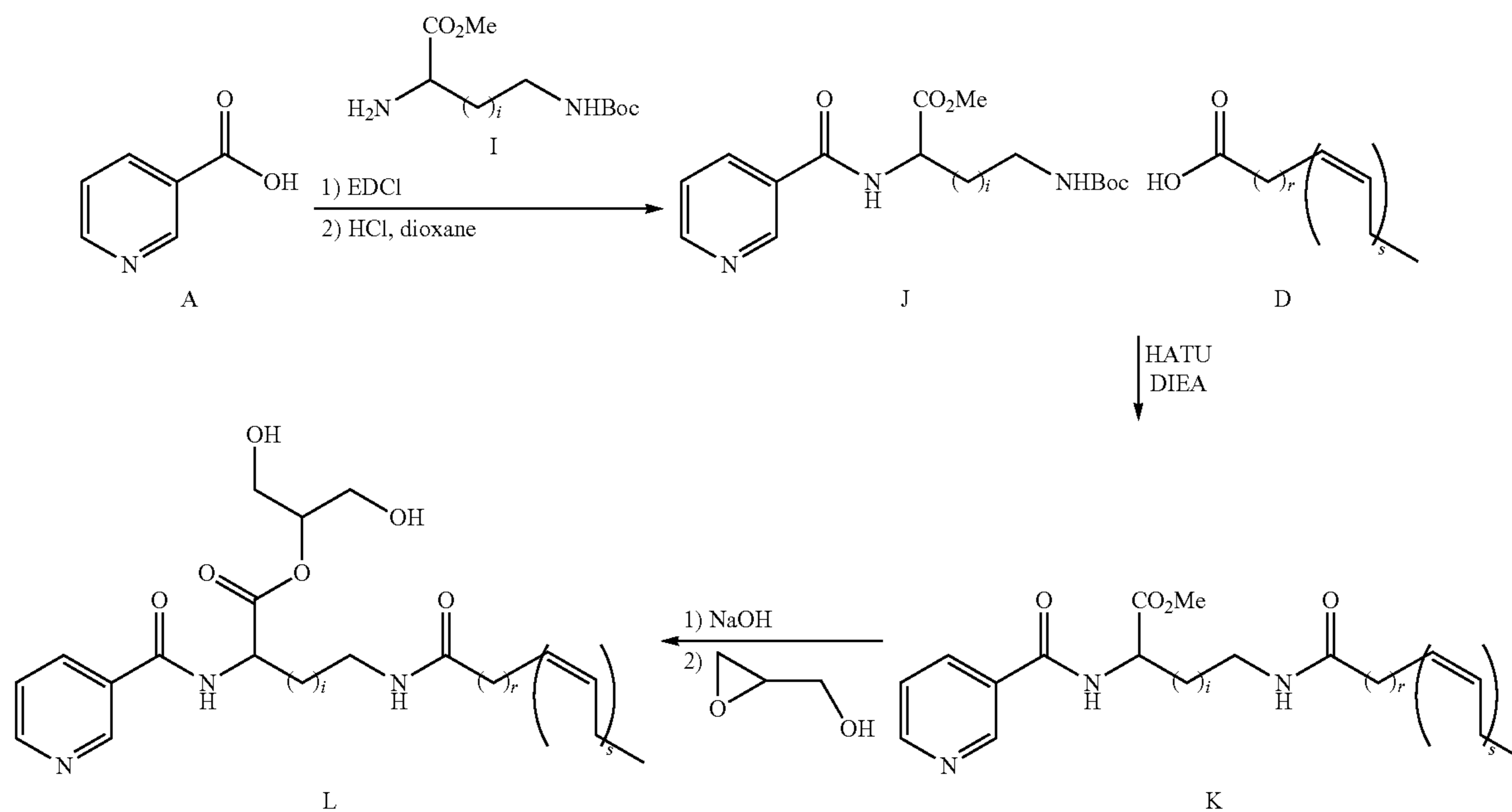
Scheme 3
