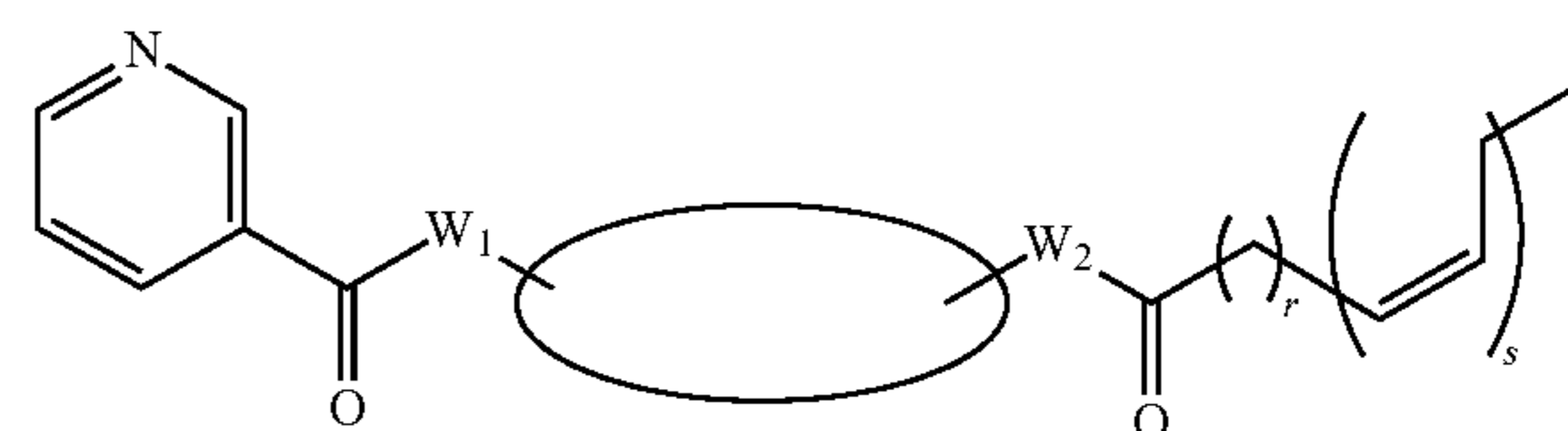
Scheme 10
