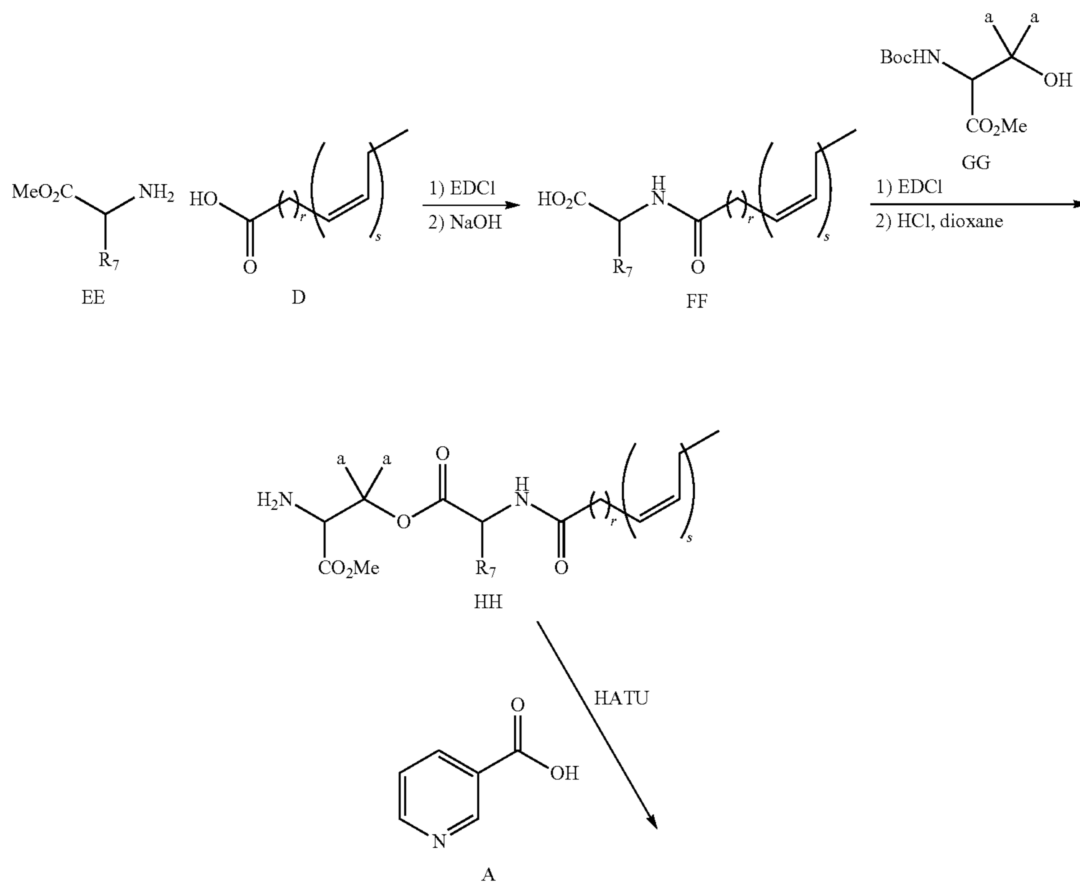
Scheme 9
