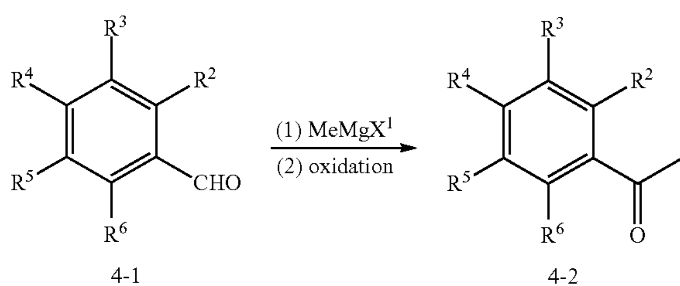
Scheme 4
