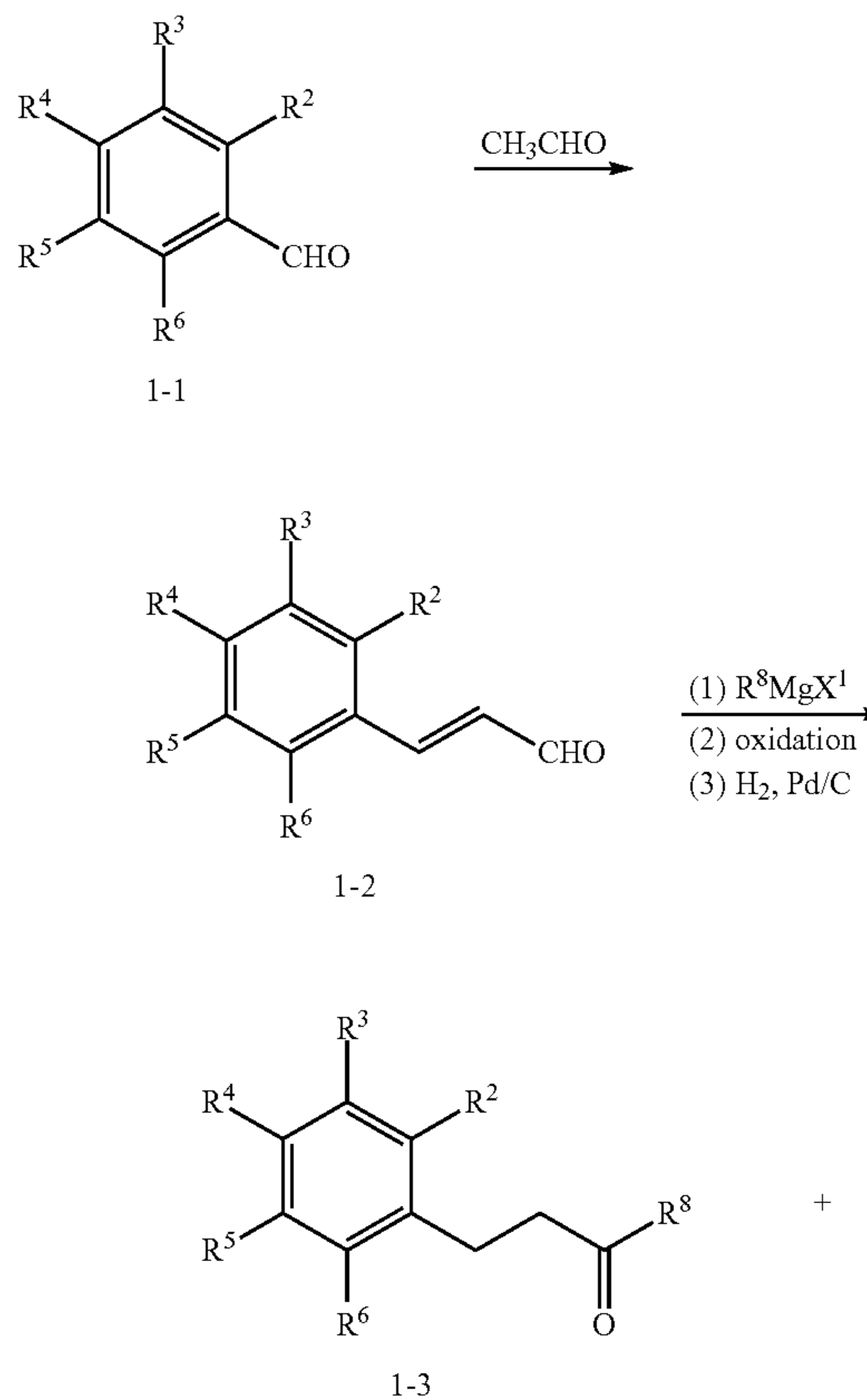
Scheme 1
