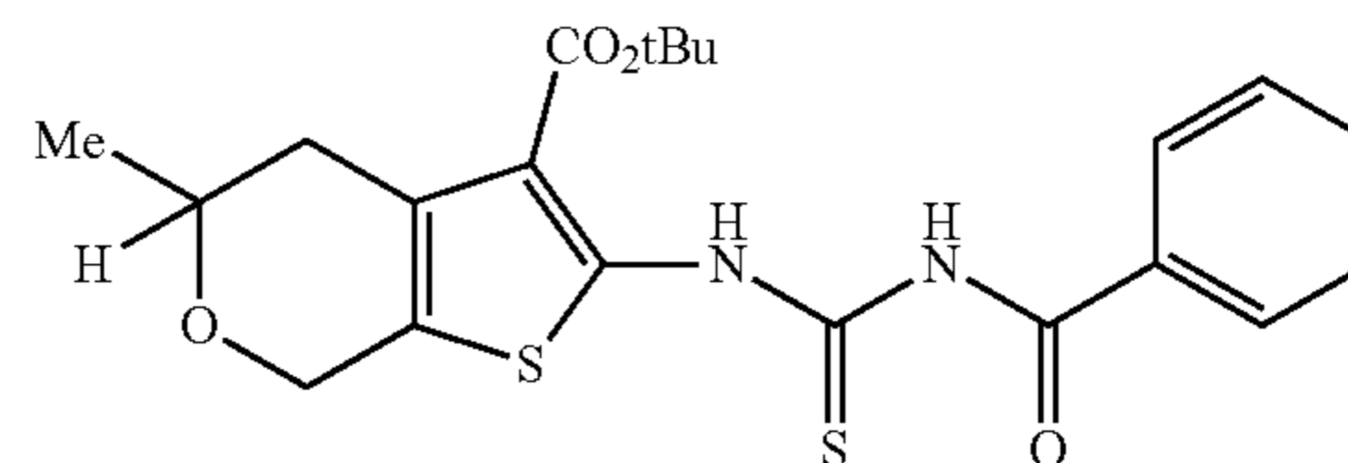
tert-butyl 2-(3-benzoylthioureido)-5-methyl-5,7-dihydro-4H-thieno[2,3-c]pyran-3-carboxylate
