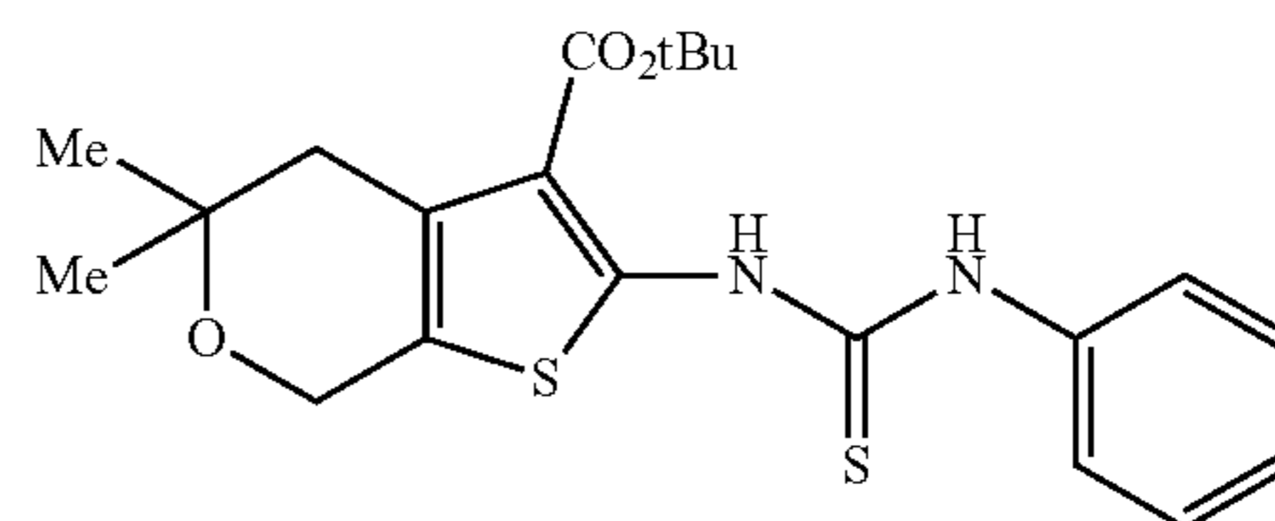
tert-butyl 5,5-dimethyl-2-(3-phenylthioureido)-5,7-dihydro-4H-thieno[2,3-c]pyran-3-carboxylate
