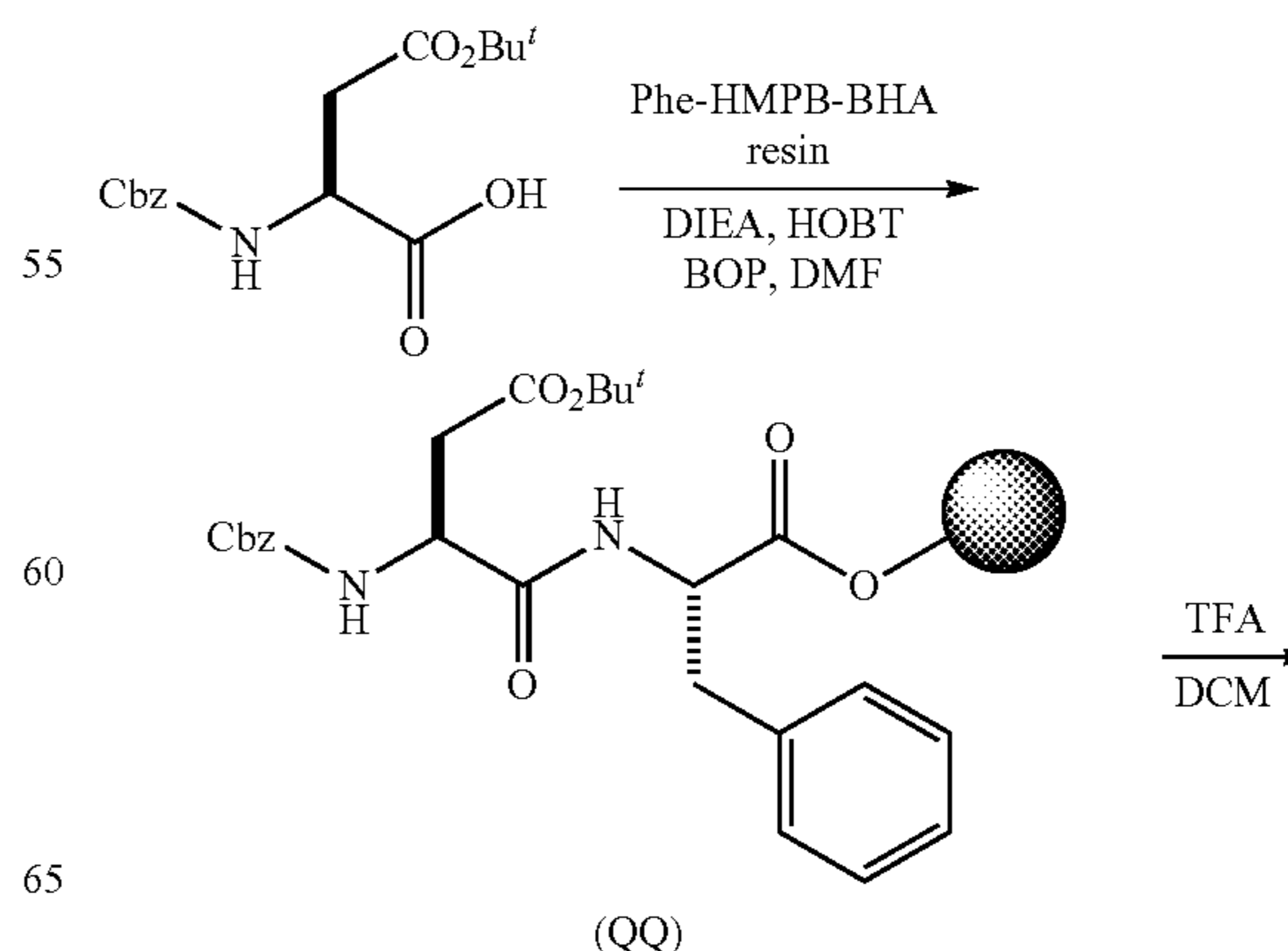
Scheme 10: Synthesis of Example 10
