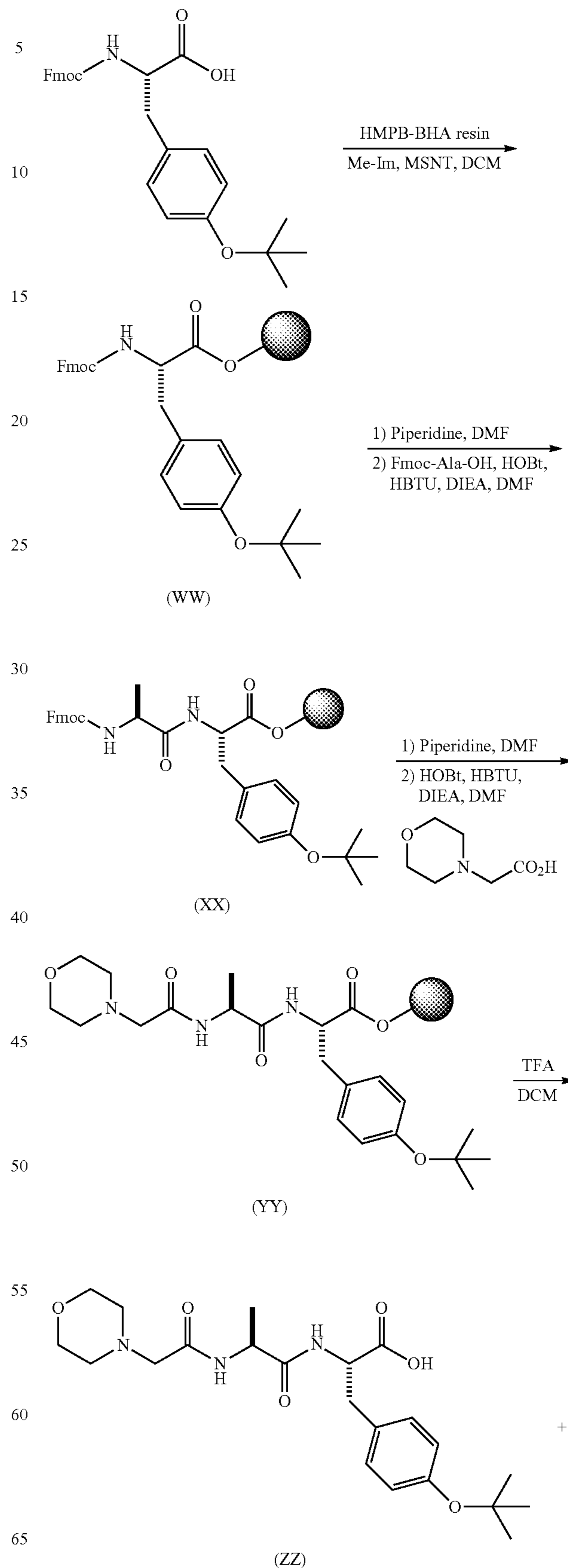
Scheme 13: Synthesis of Example 13
