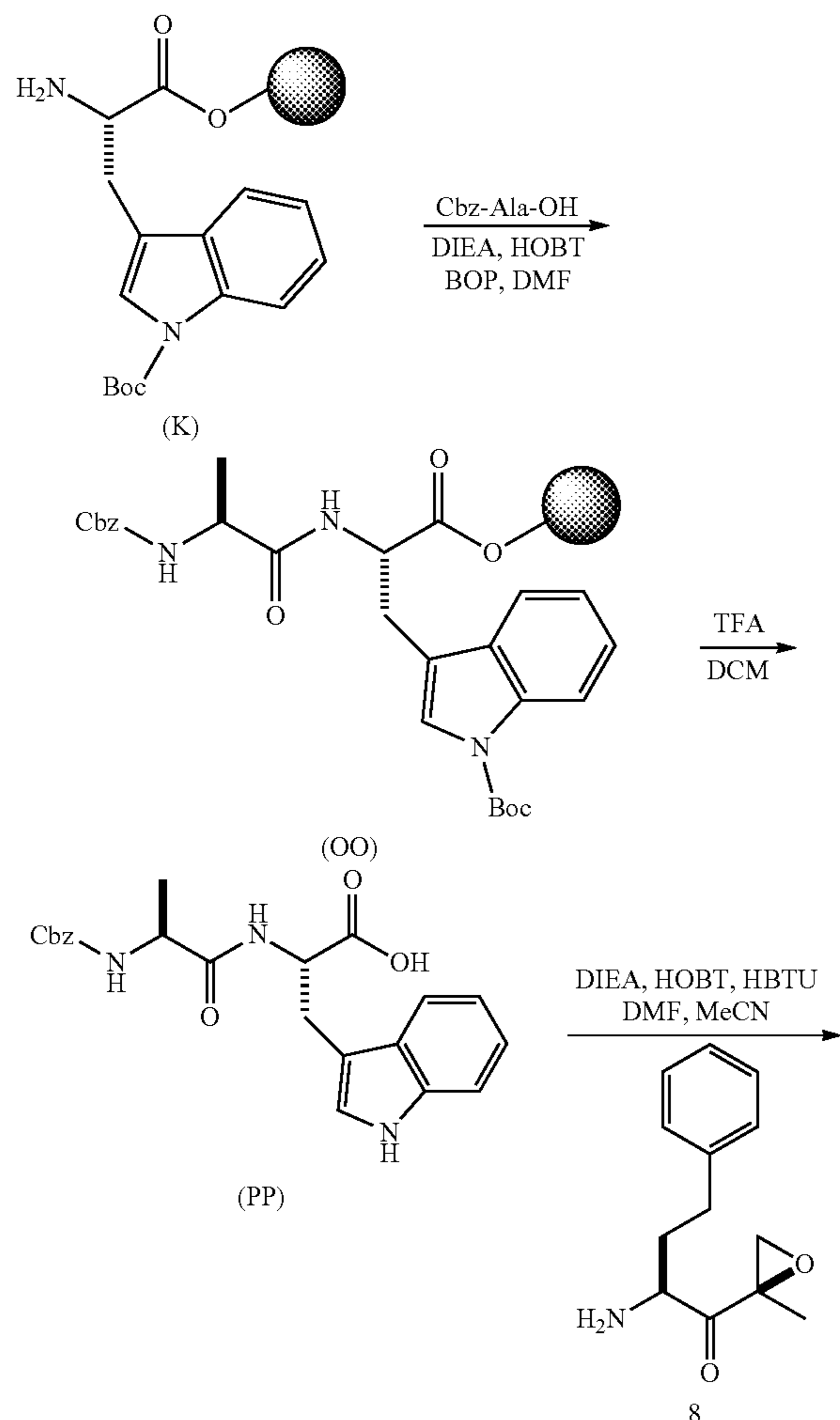
Scheme 9: Synthesis of Example 9
