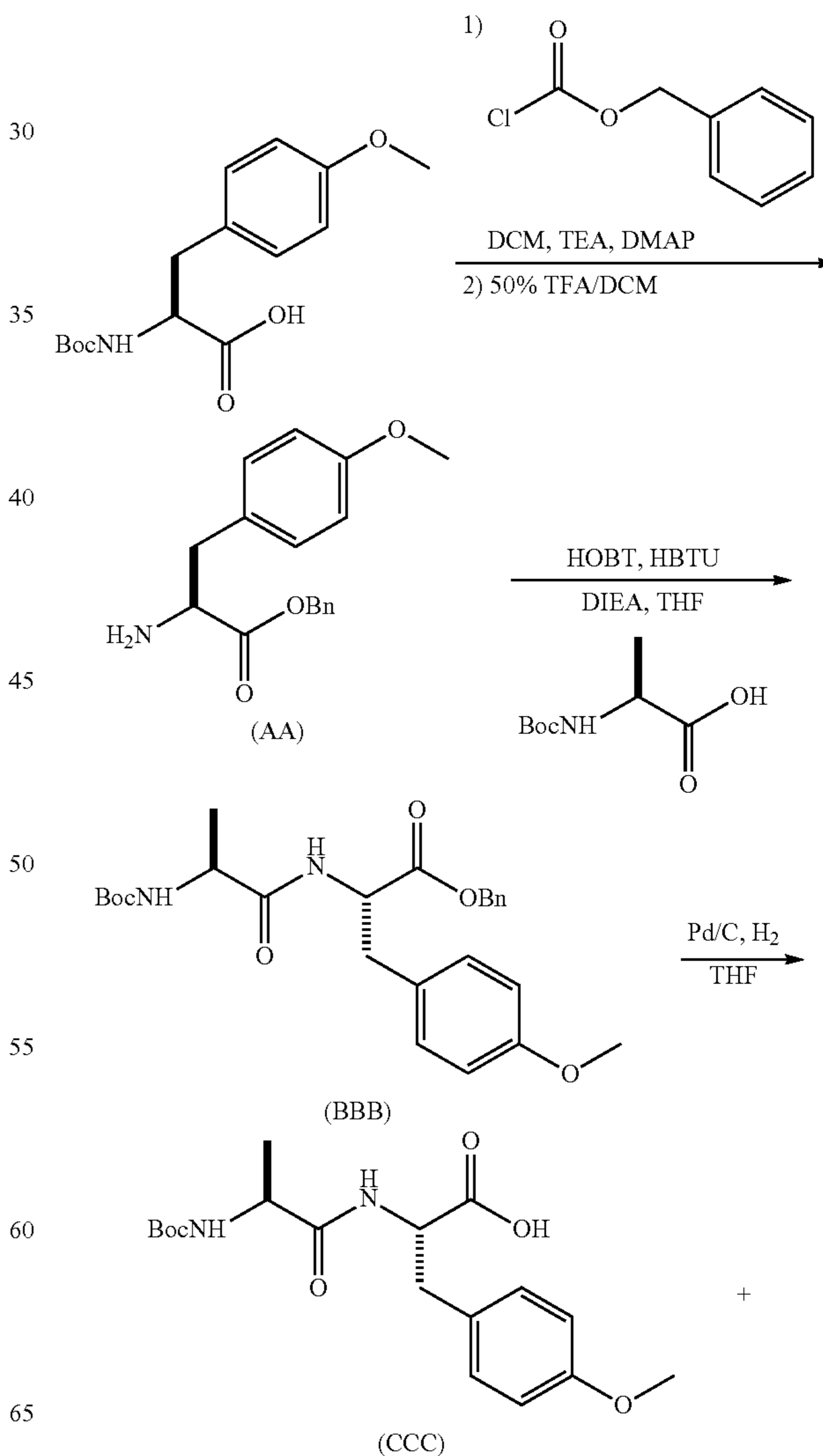
Scheme 14: Synthesis of Example 14
