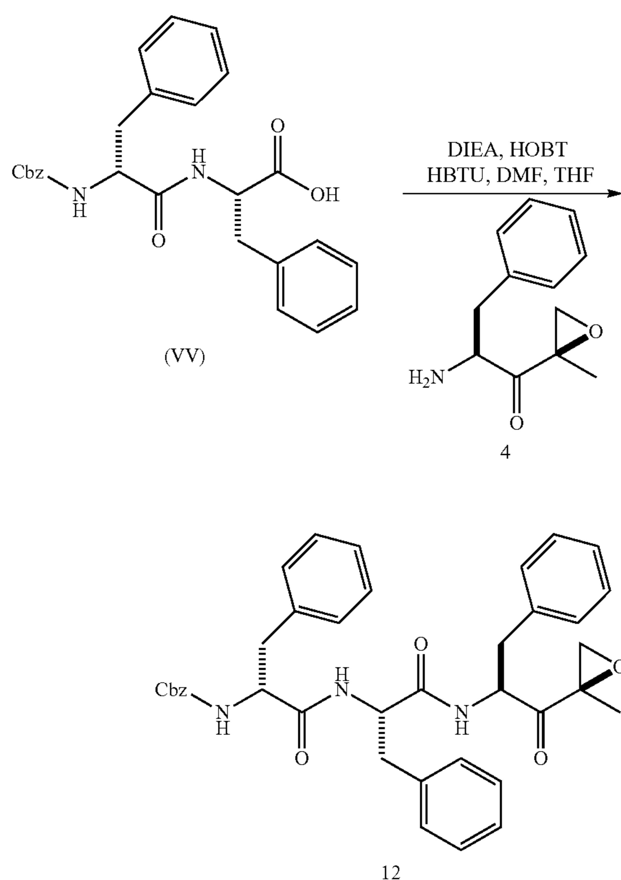
Scheme 12: Synthesis of Example 12
