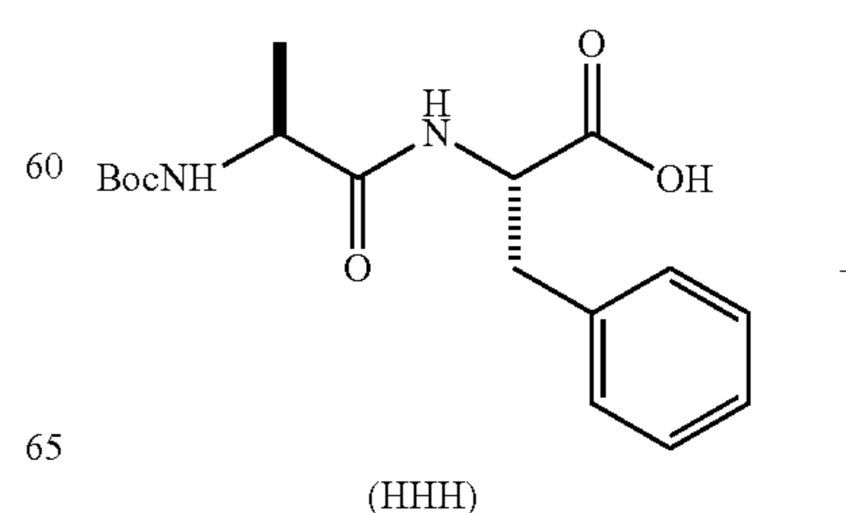
Scheme 17: Synthesis of Example 17
