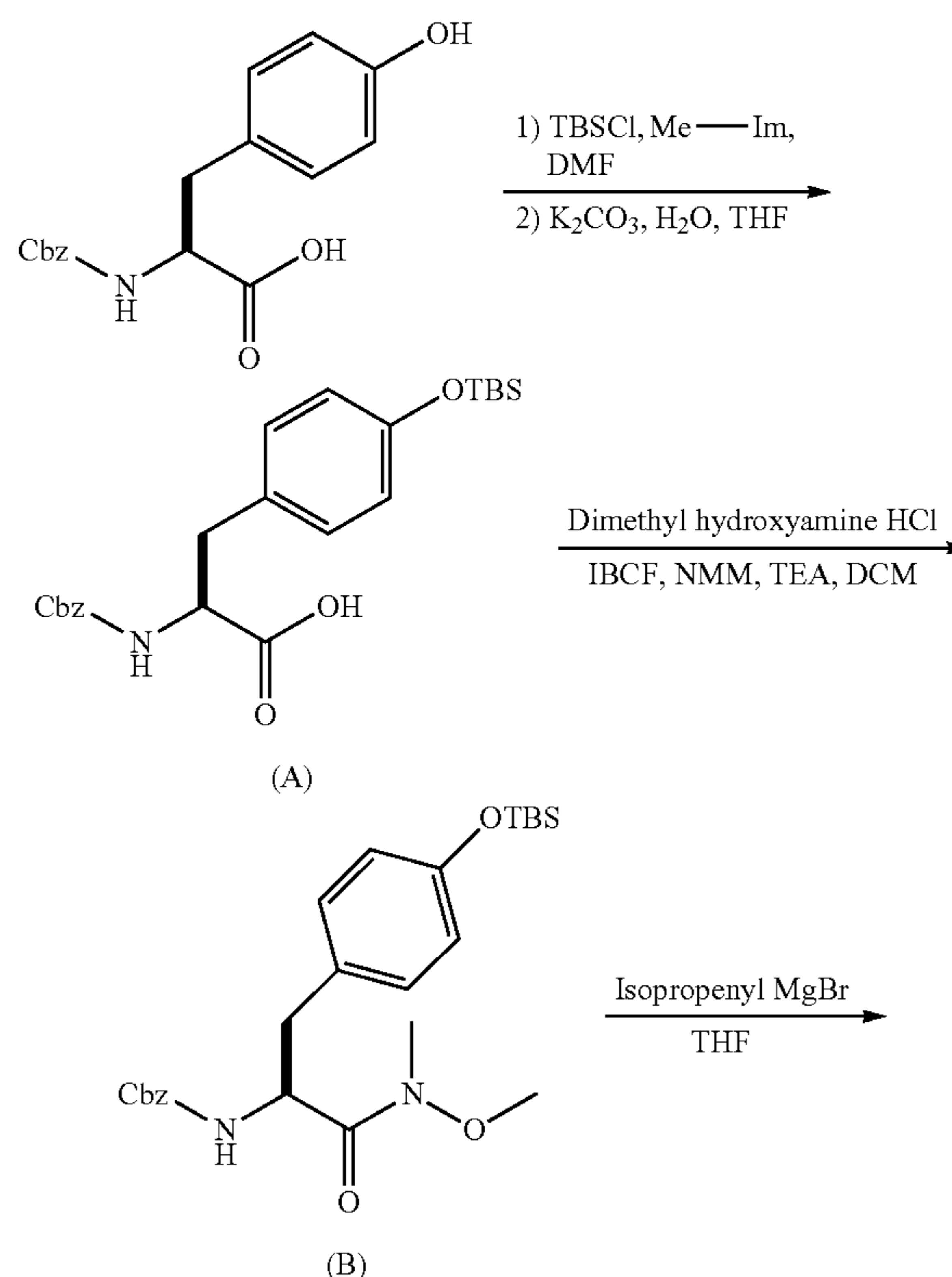
Scheme 1: Synthesis of Example 1
