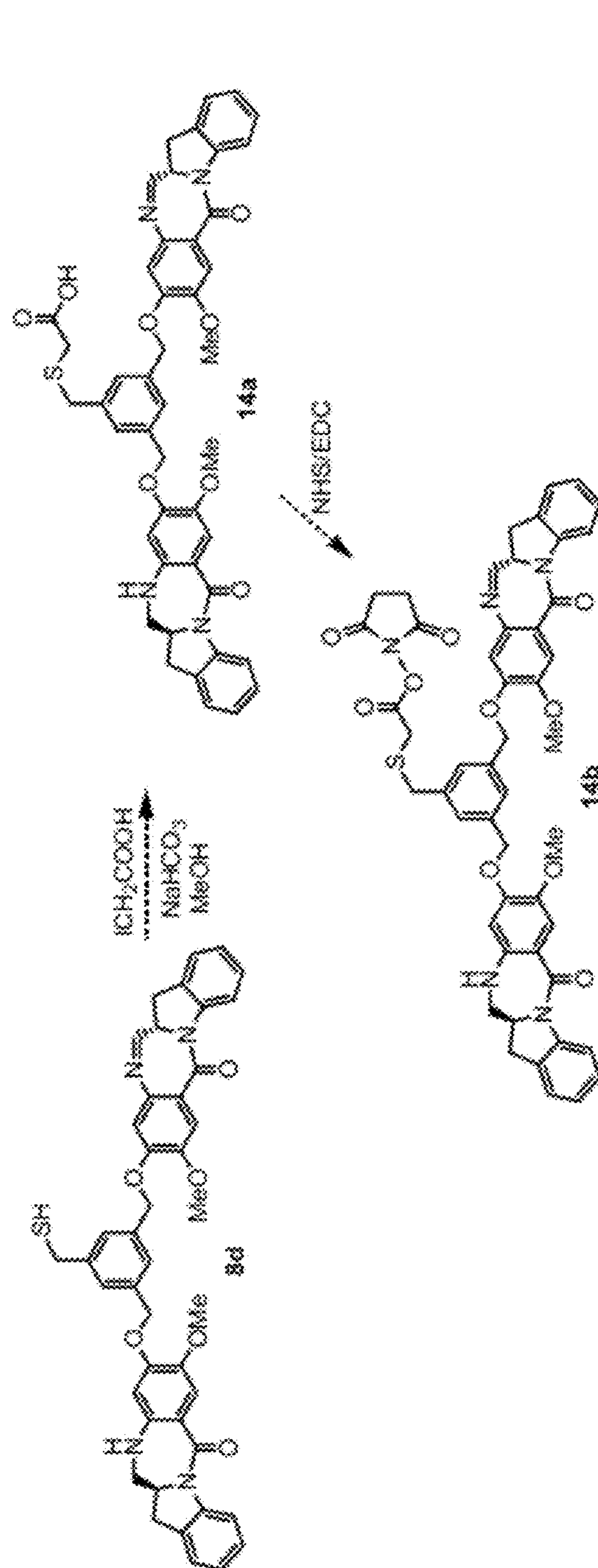
Figure 17. Synthetic Scheme of the One-step Thioncetyl Linkable Dimers 14a-b
