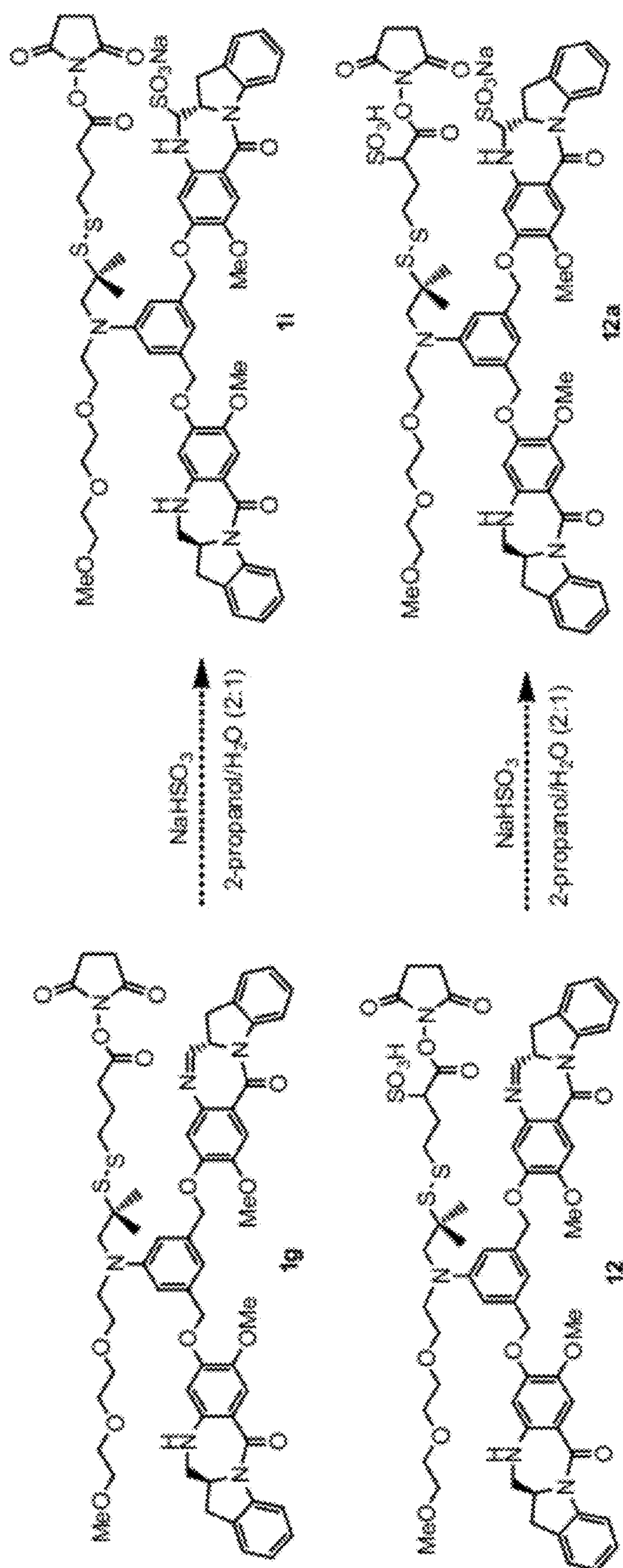
Figure 43. Synthetic Scheme of Compounds 11 and 12a
