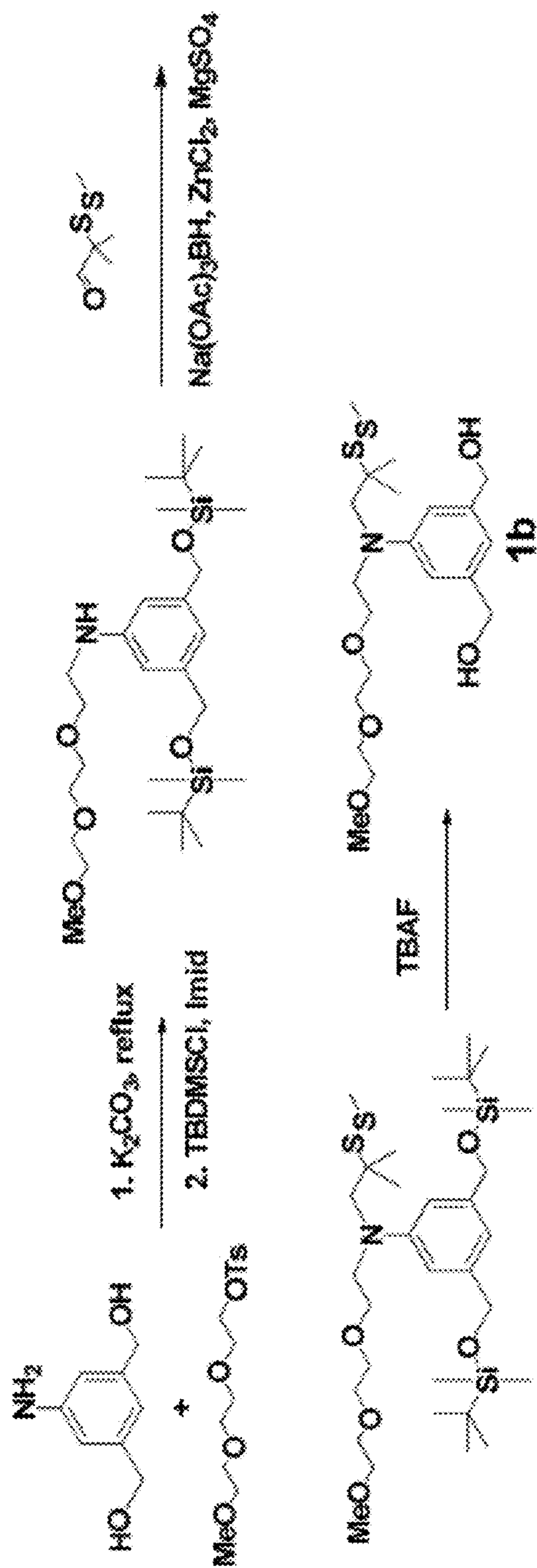
Figure 46. Alternate Synthesis of (5-(2-(2-(2-methoxyethoxy)ethoxy)ethyl)(2-methyl-2-(methylidisulfonyl)propyl)amino)-1,3-phenylene)dimethanol (1b)
