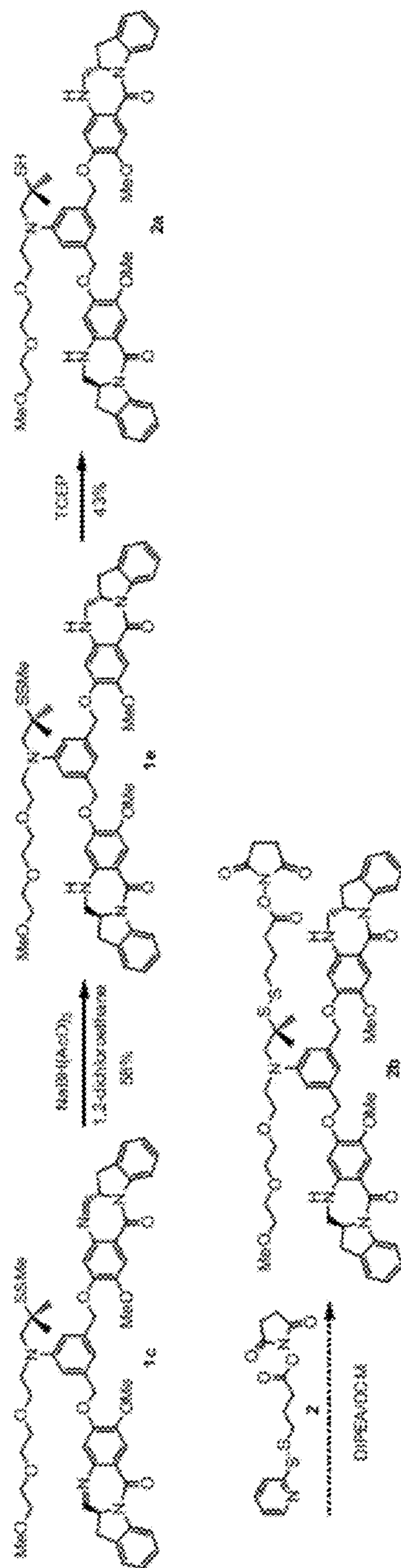
Figure 2. Synthetic Scheme of Dimers 2a-h
