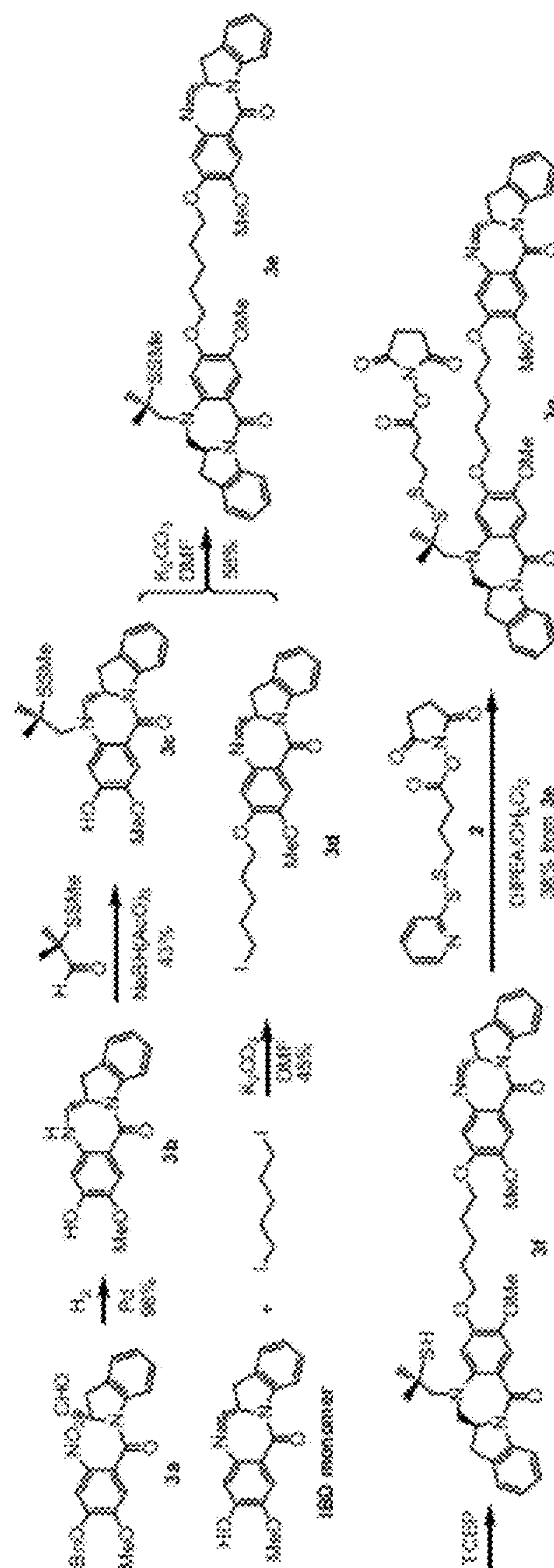
Figure 3. Synthetic Scheme of Dimers 3e-g
