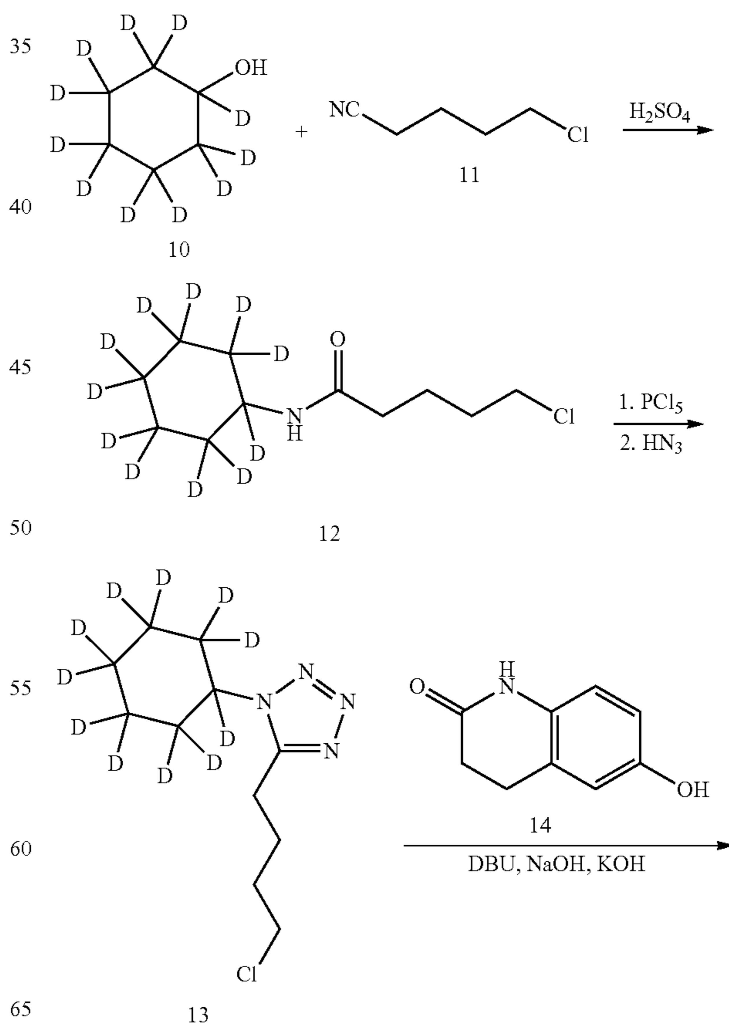
Scheme 1. Preparation of Compound 106
