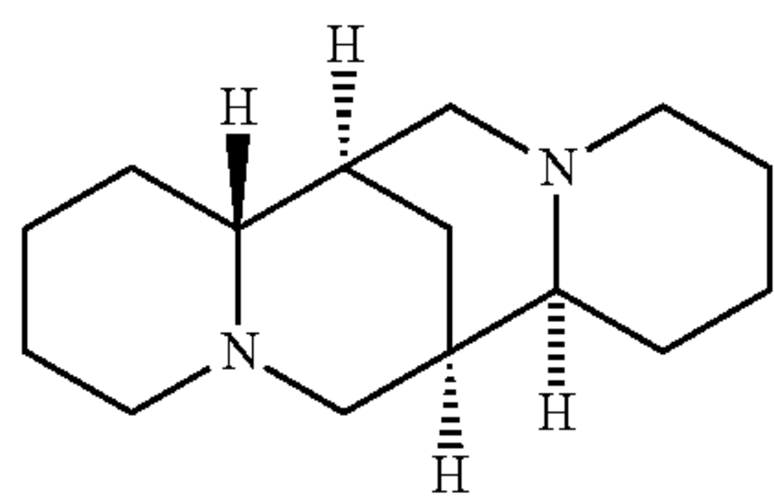
(-)-Sparteine (Sp)
