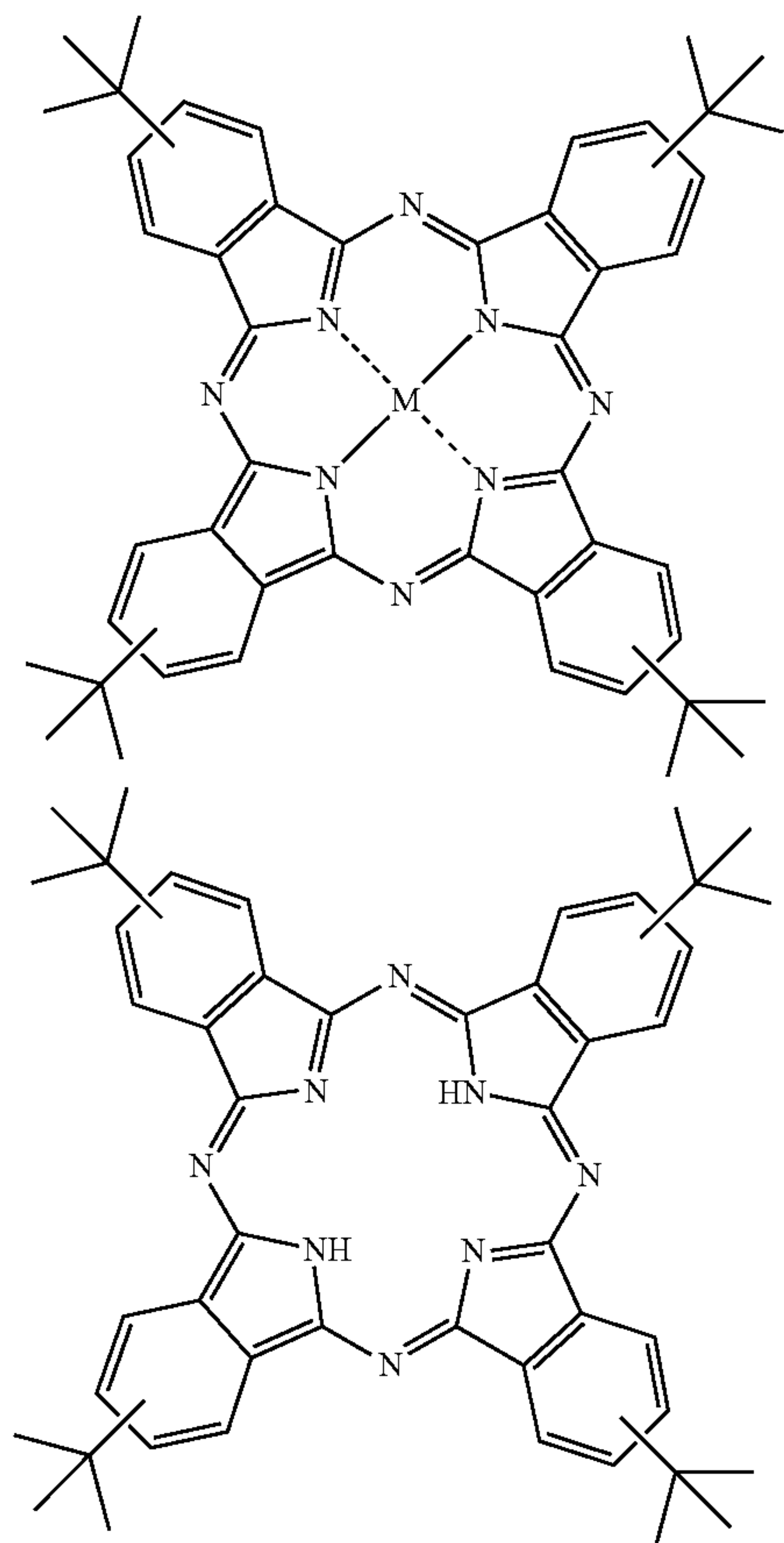
(TBP)
