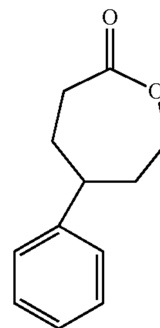
5-Phenyloxepan-2-one (PXO)
