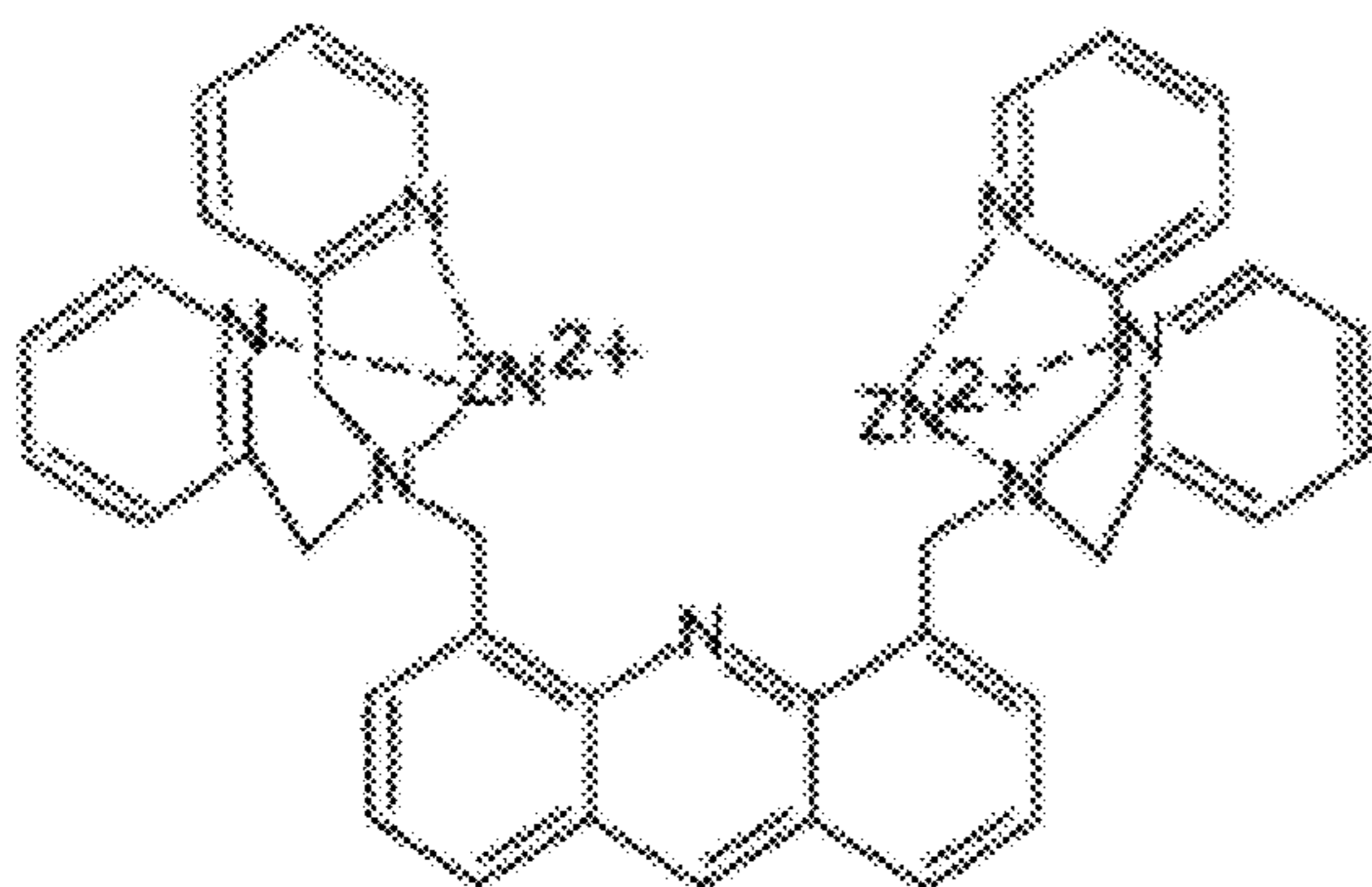
Compound 3
