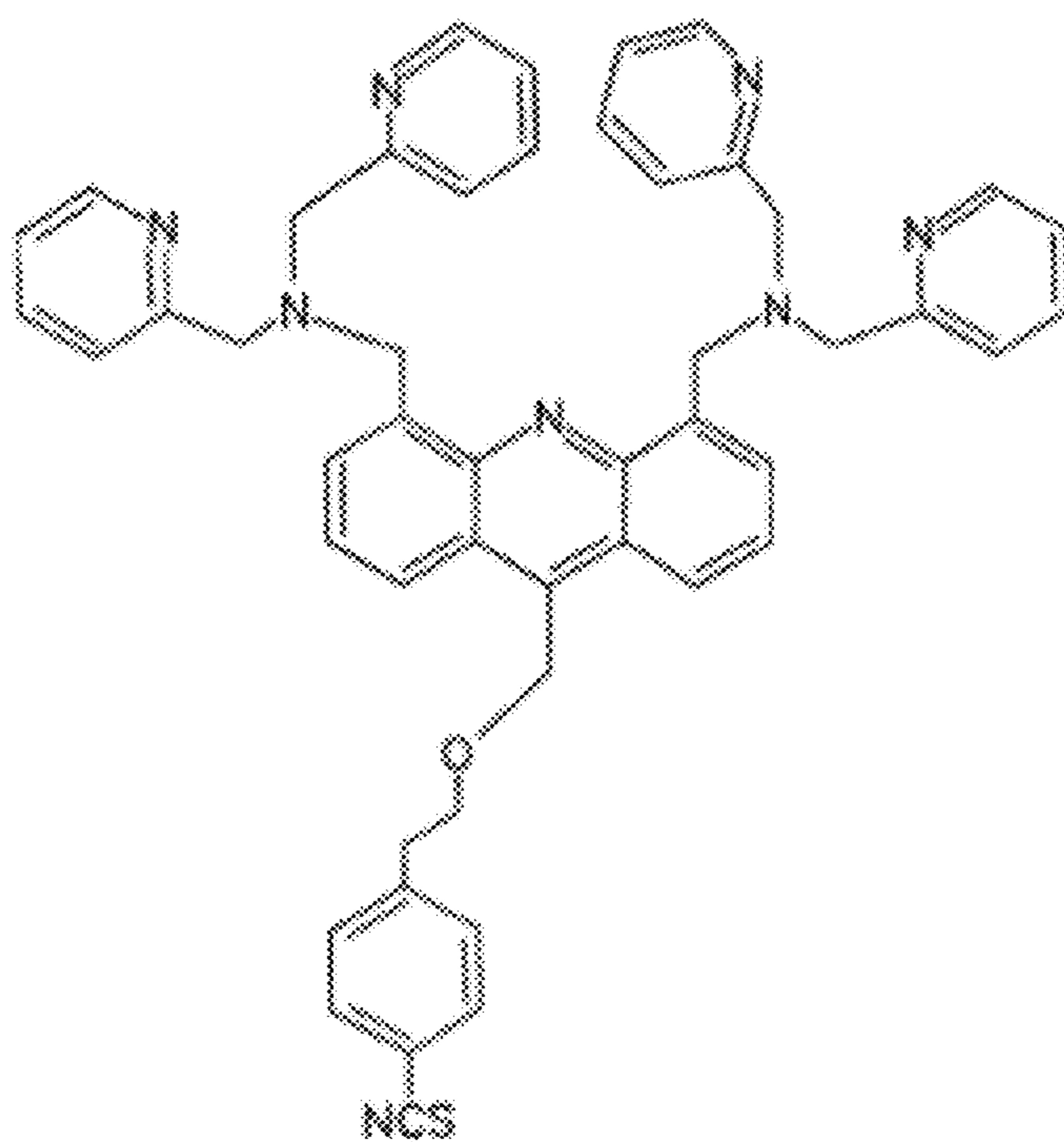
Compound 10
