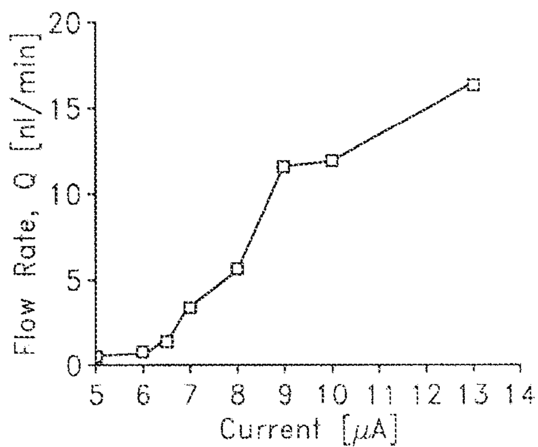
Ultra low flow rate FIG. 21B
