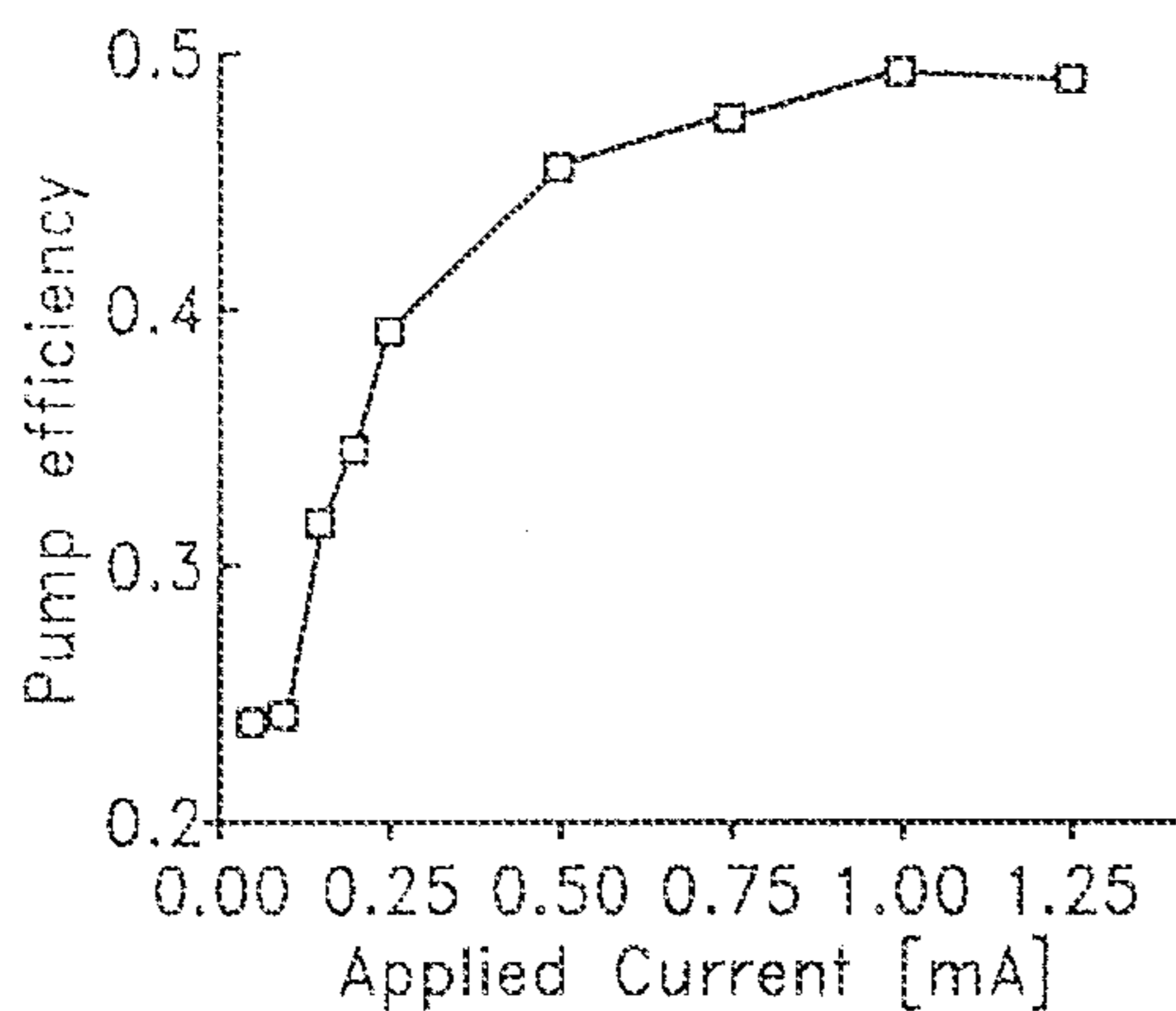
Pump efficiency FIG. 21C
