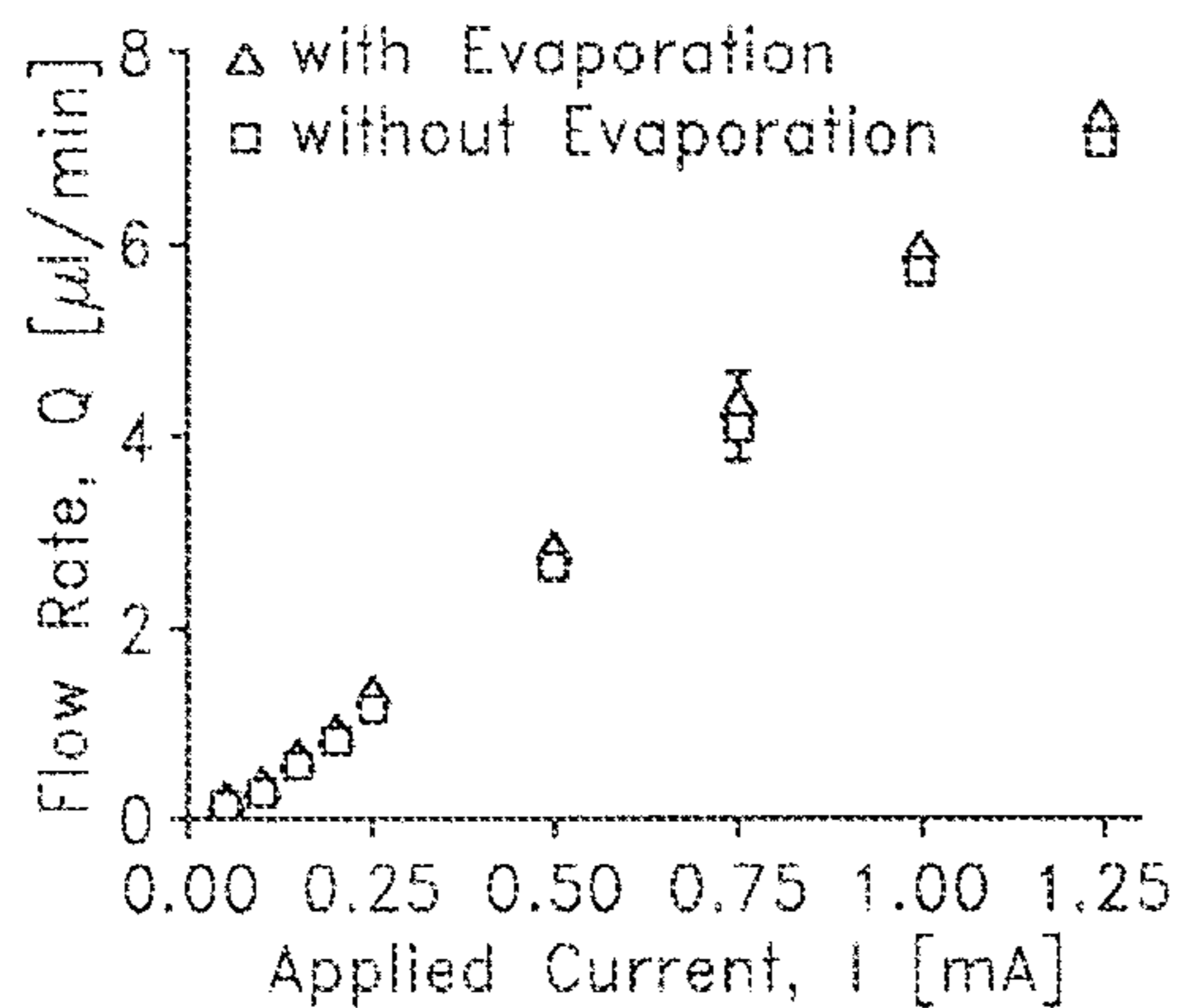
Flow rate testing FIG. 21A
