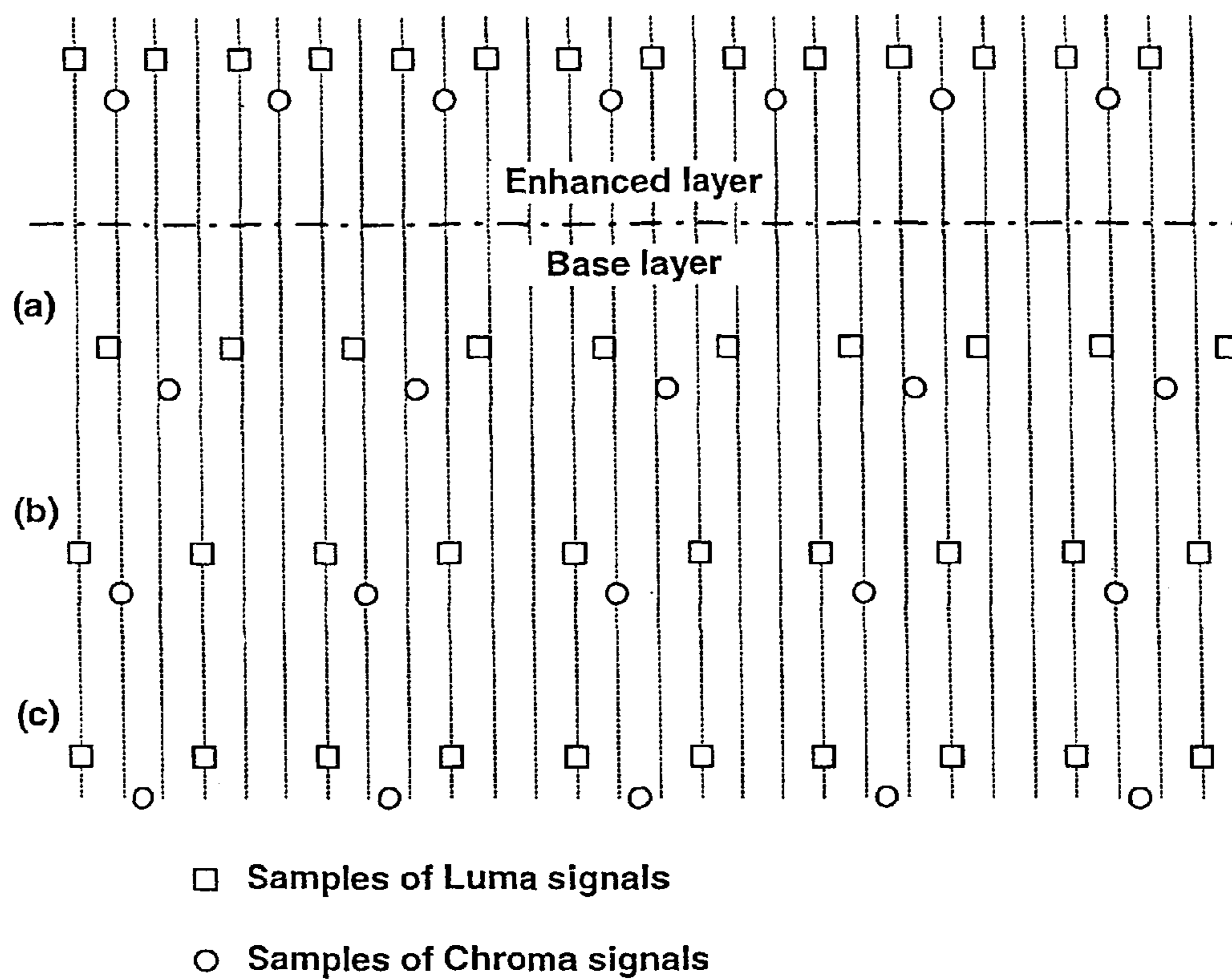
FIG. 12 (PRIOR ART)
