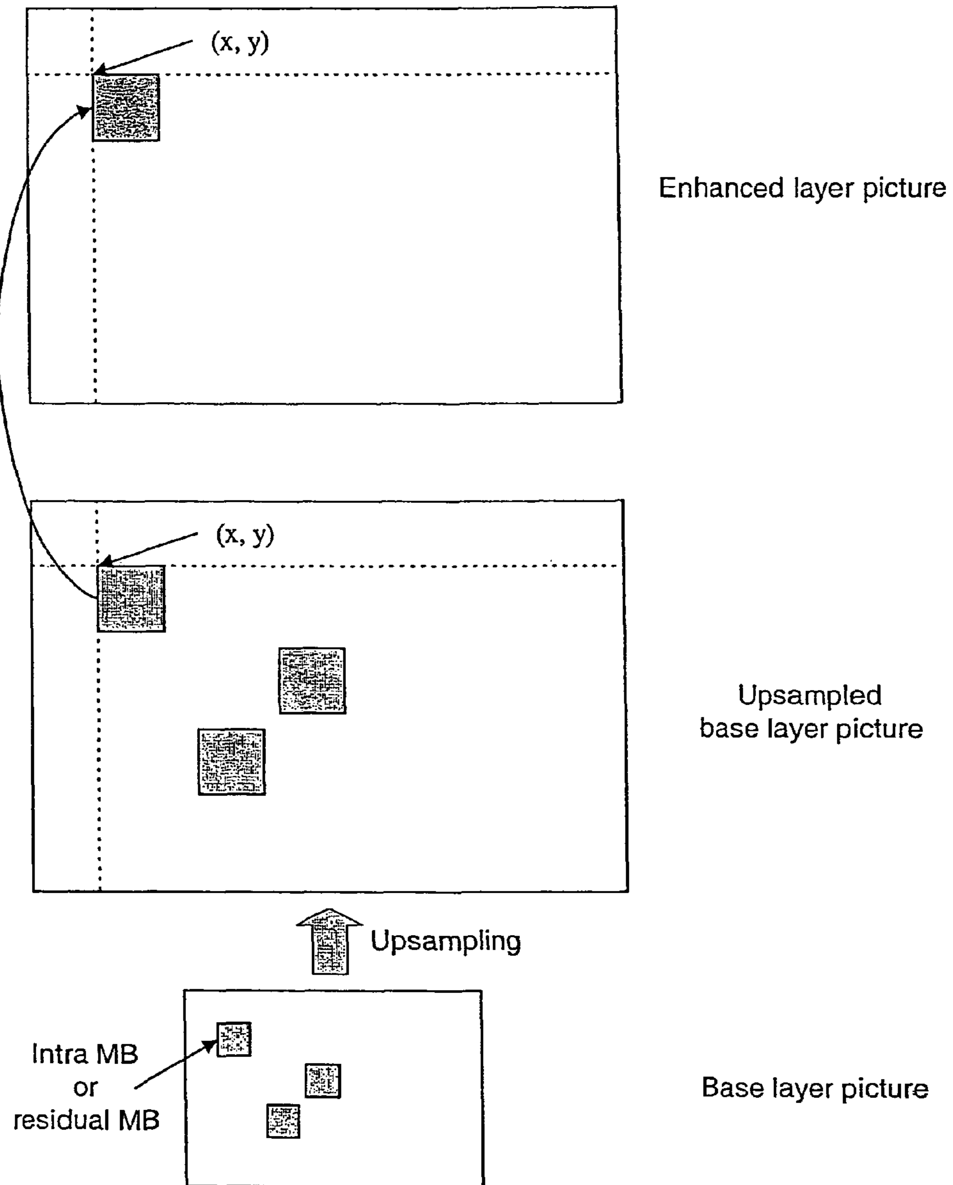
FIG. 11 (PRIOR ART)
