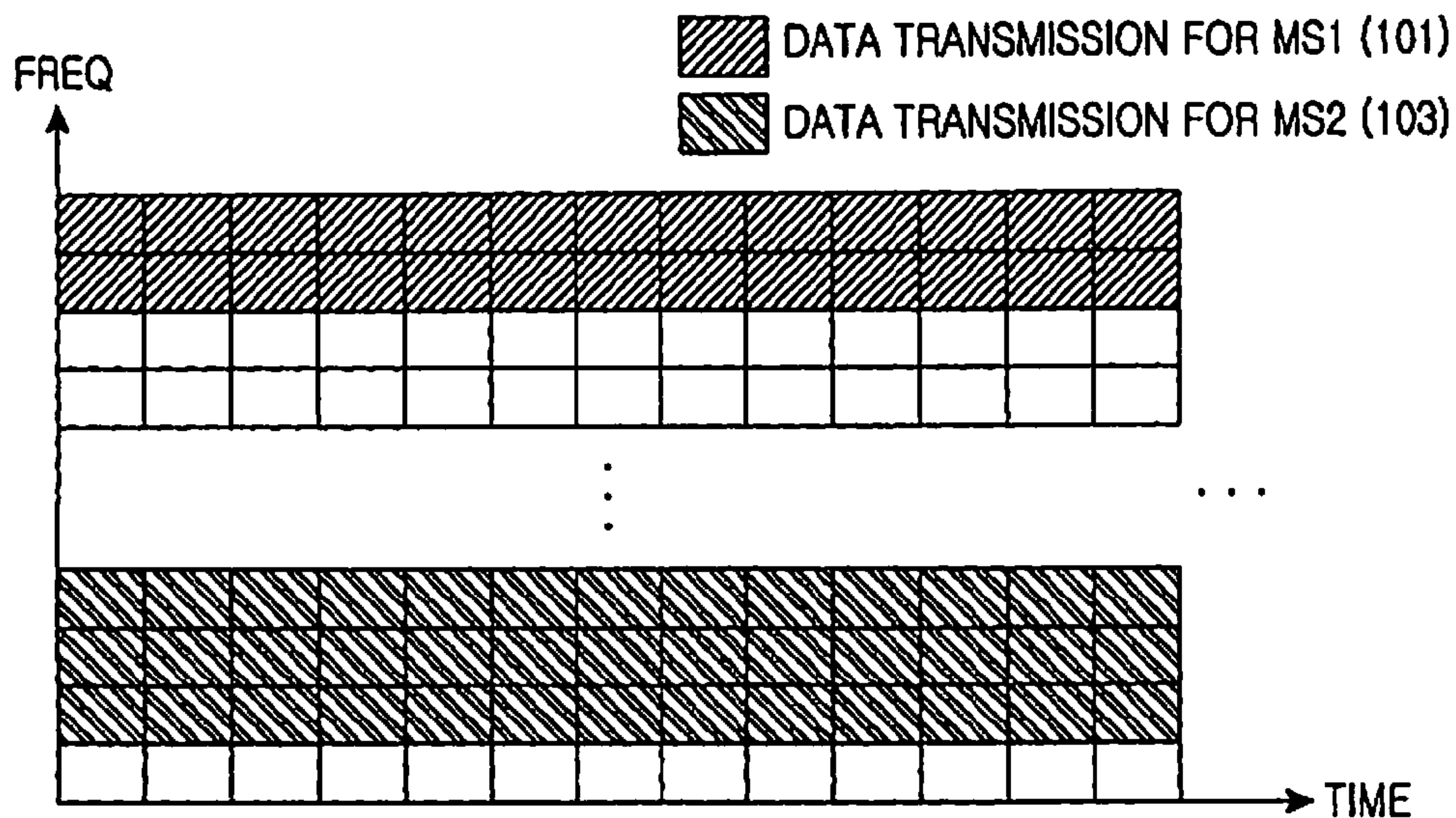
FIG. 1 (PRIOR ART)
