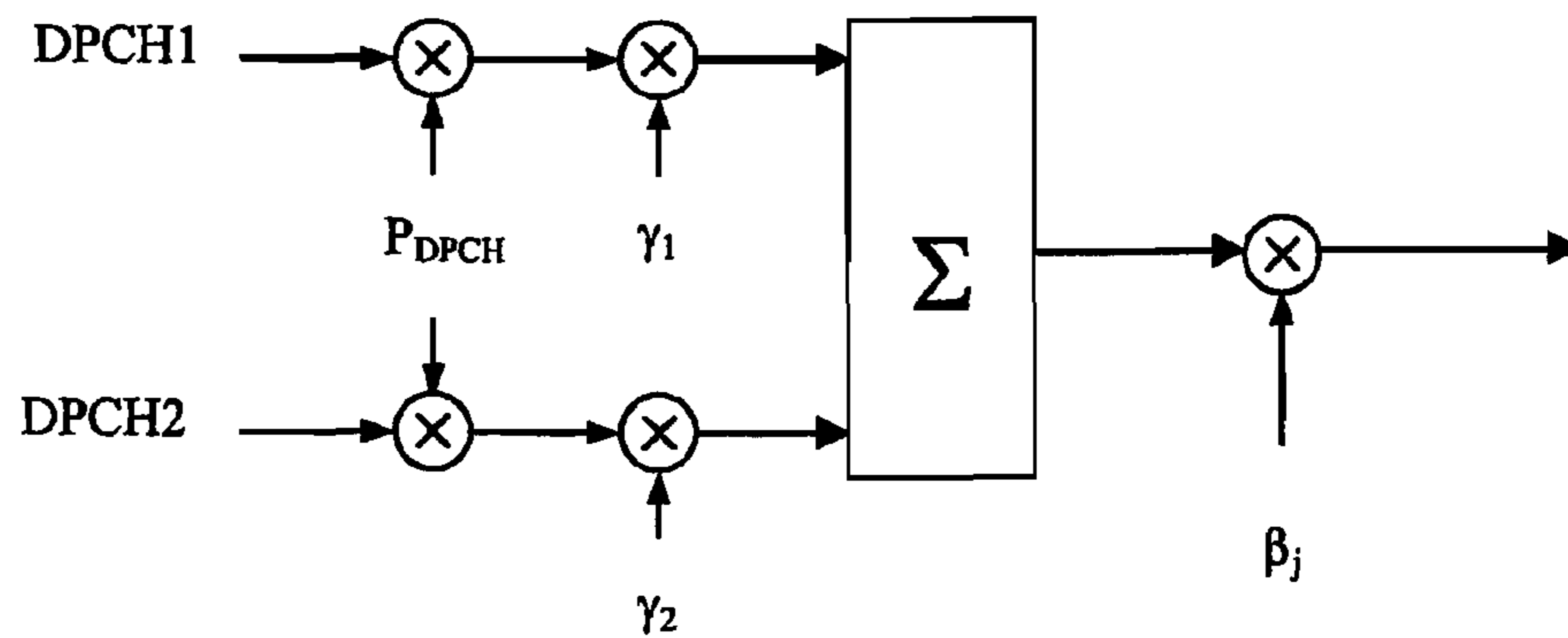
Figure 3 (Prior Art)
