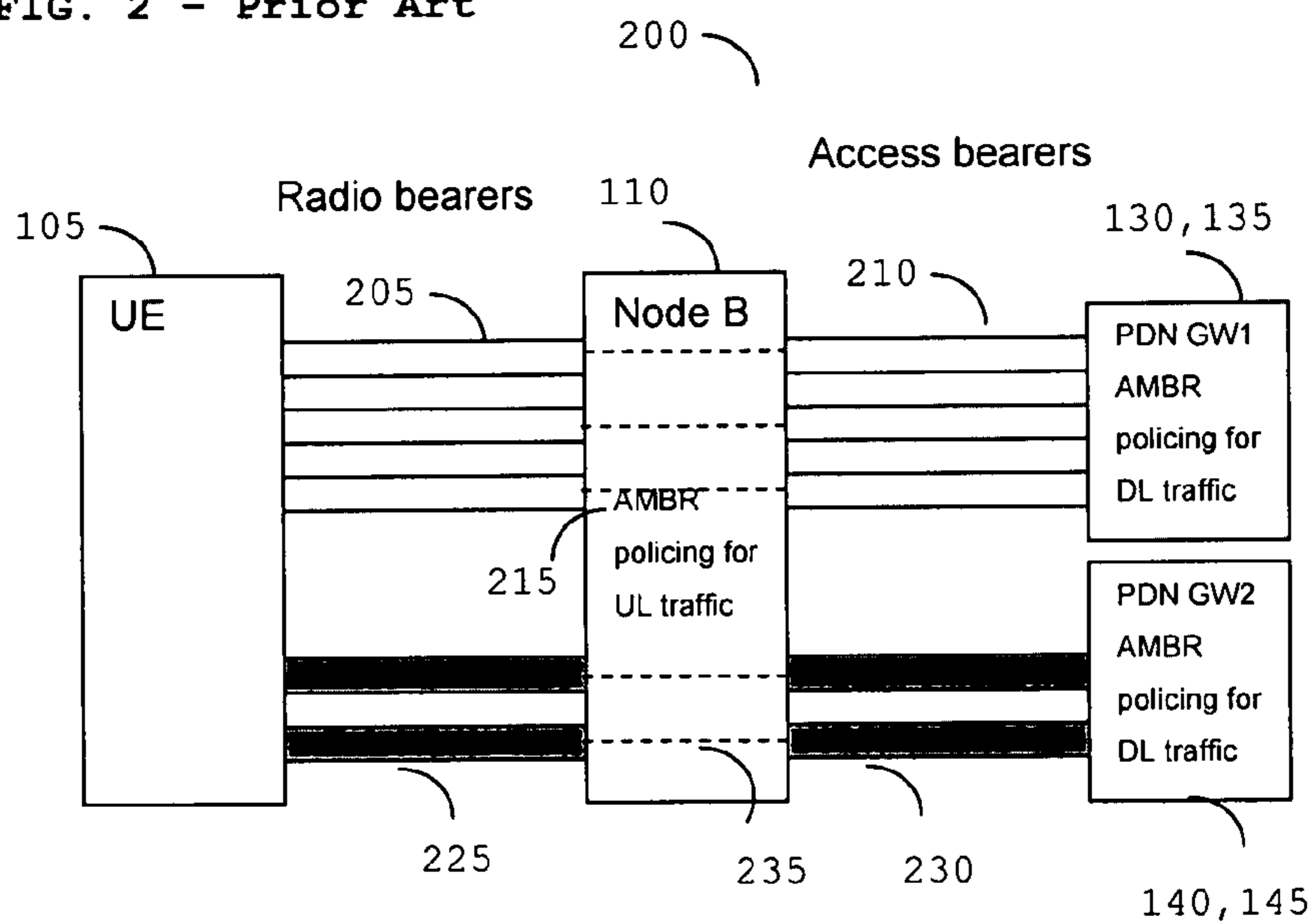
FIG. 2 - Prior Art
