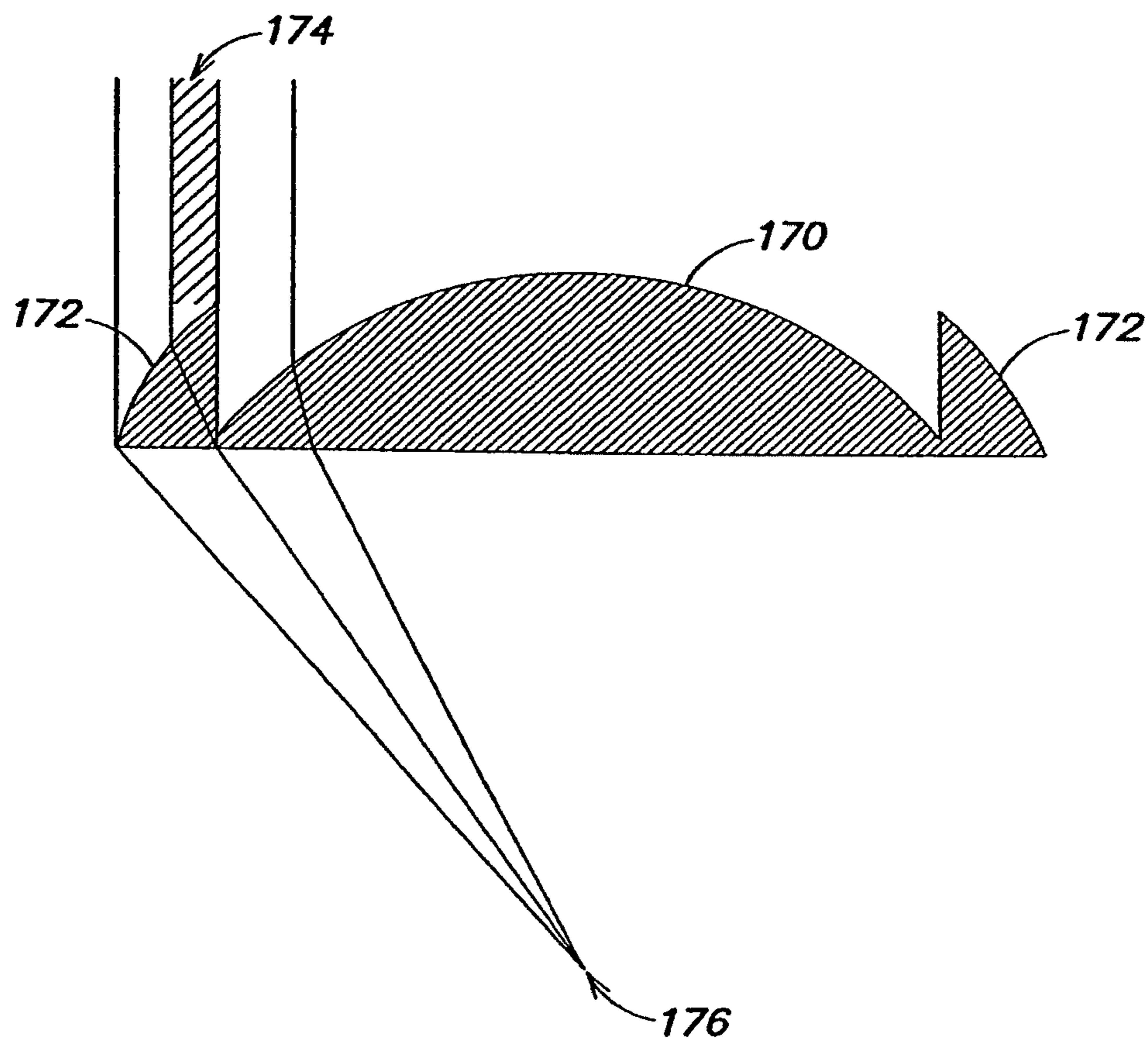
FIG. 9 (RELATED ART)
