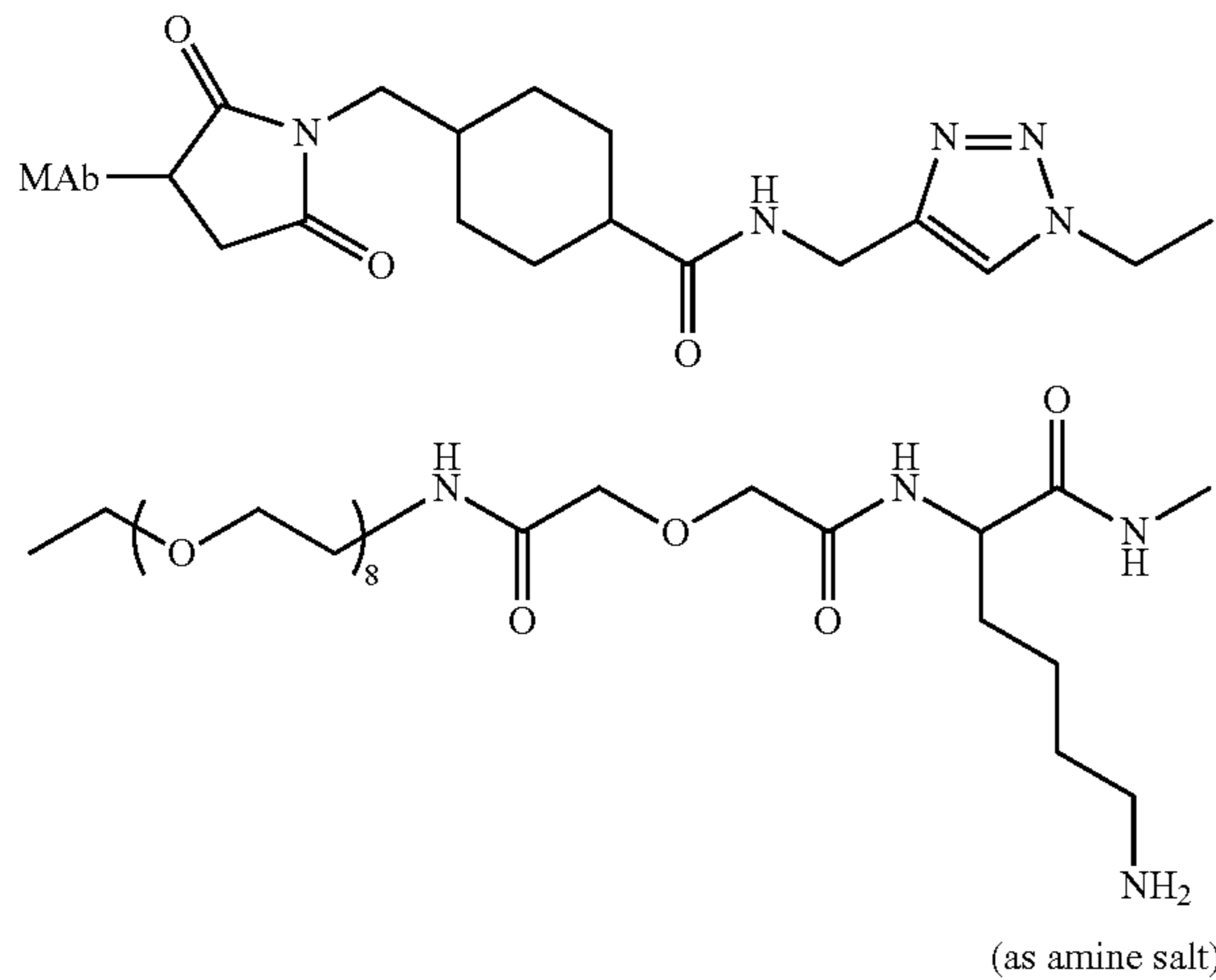
MAb-CL2A-SN-38
