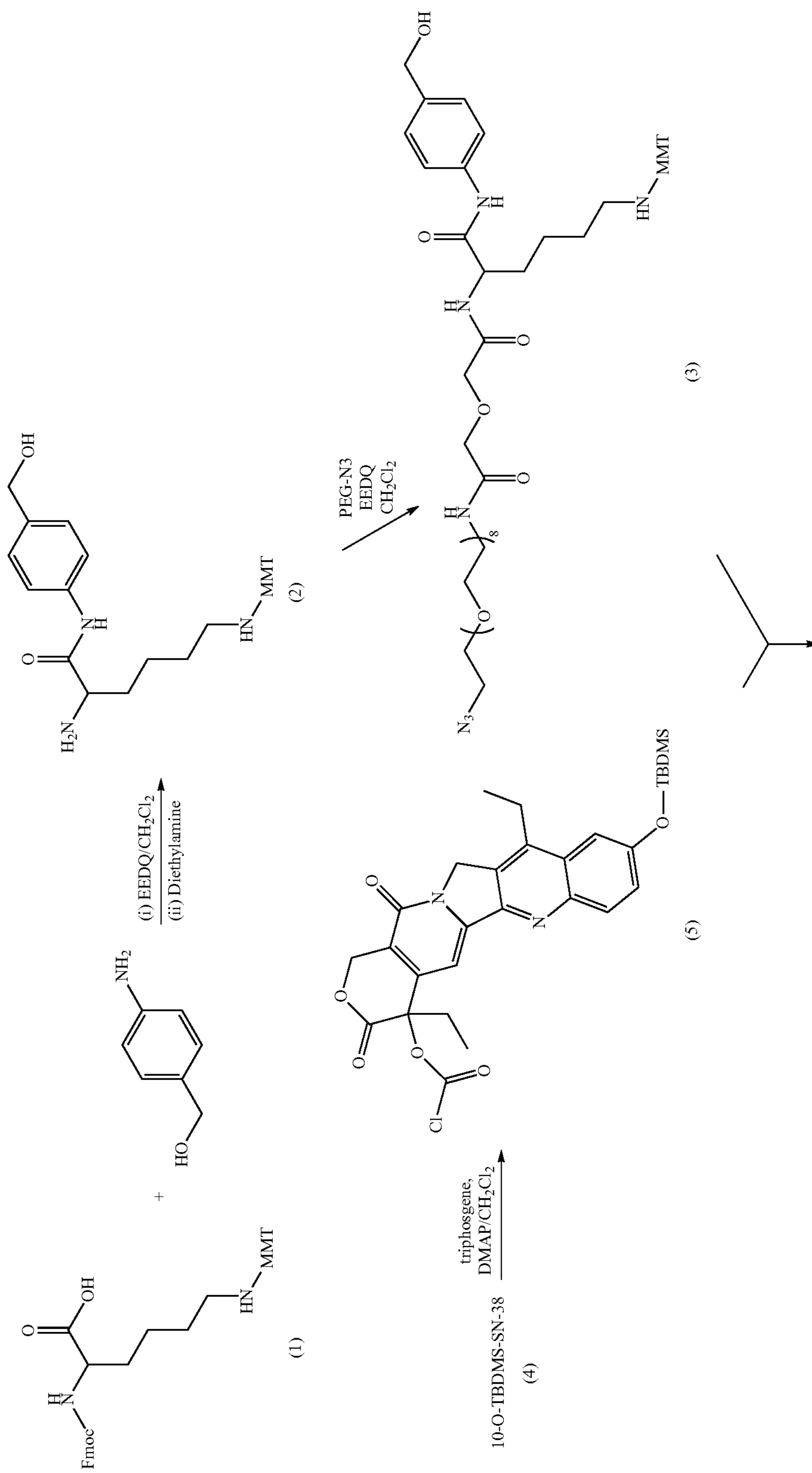
Scheme-3: Preparation of CL2A-SN-38
