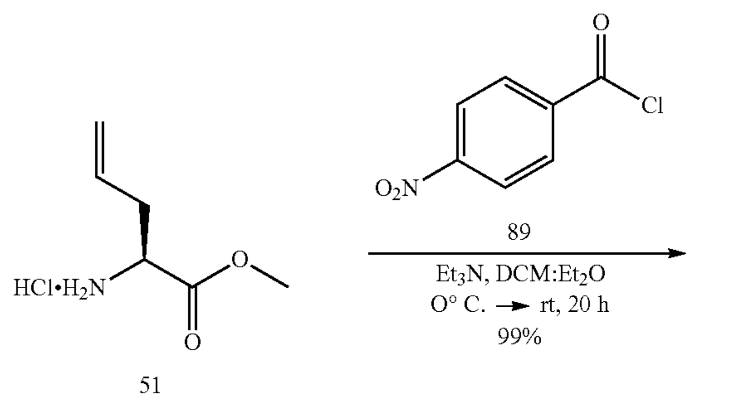
Scheme 5.5
