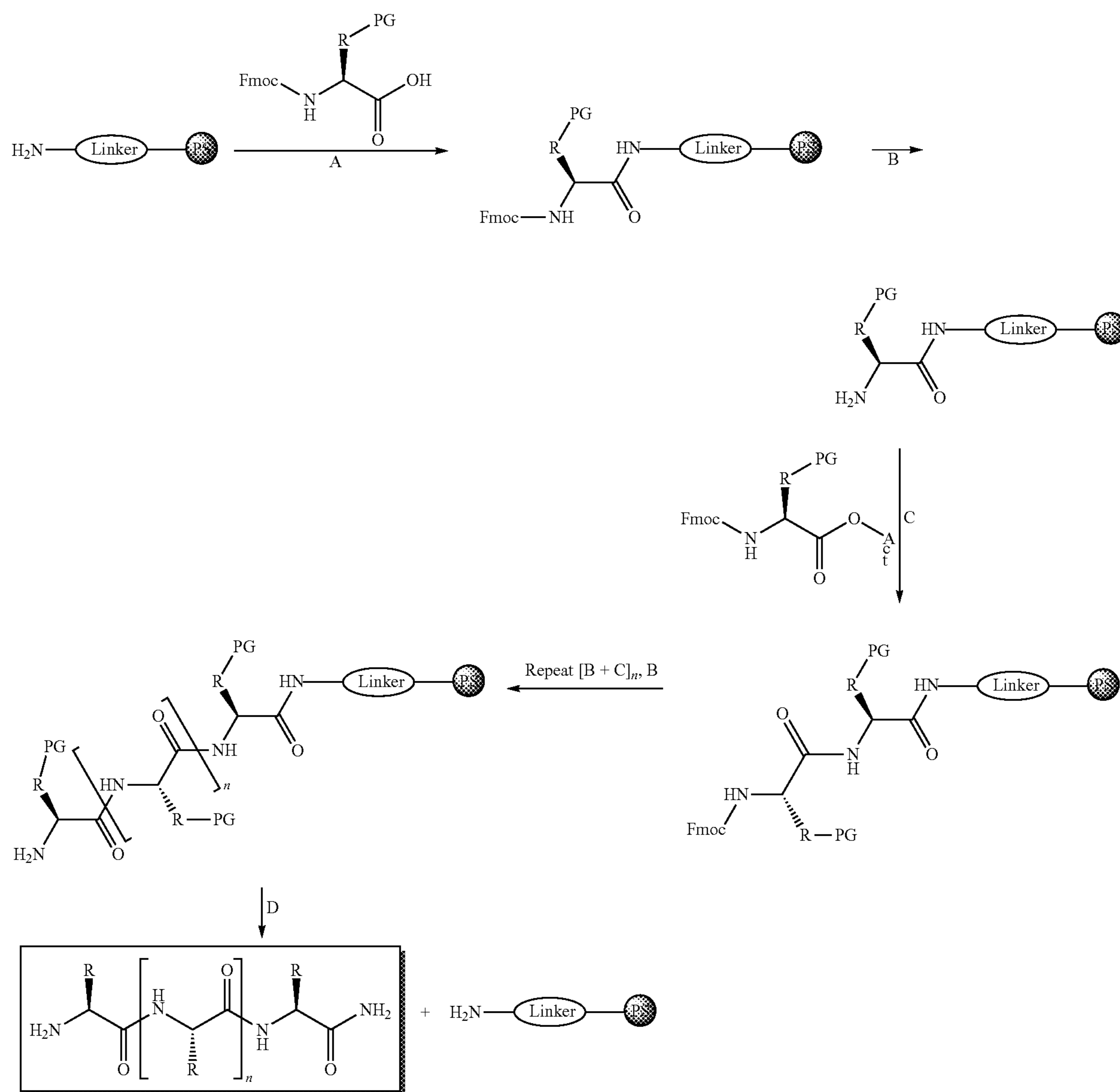
Scheme 6.1
