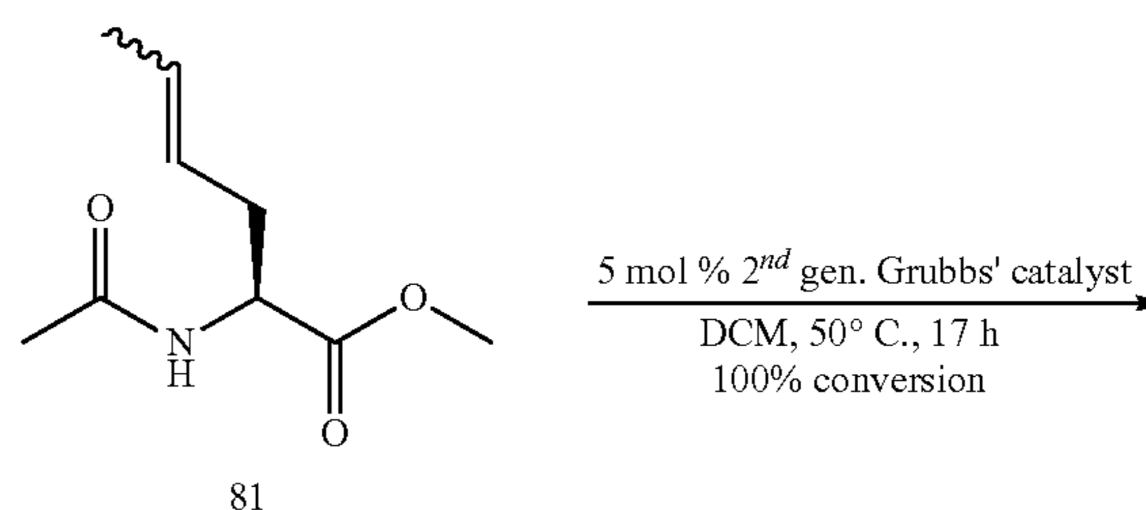
Scheme 4.34
