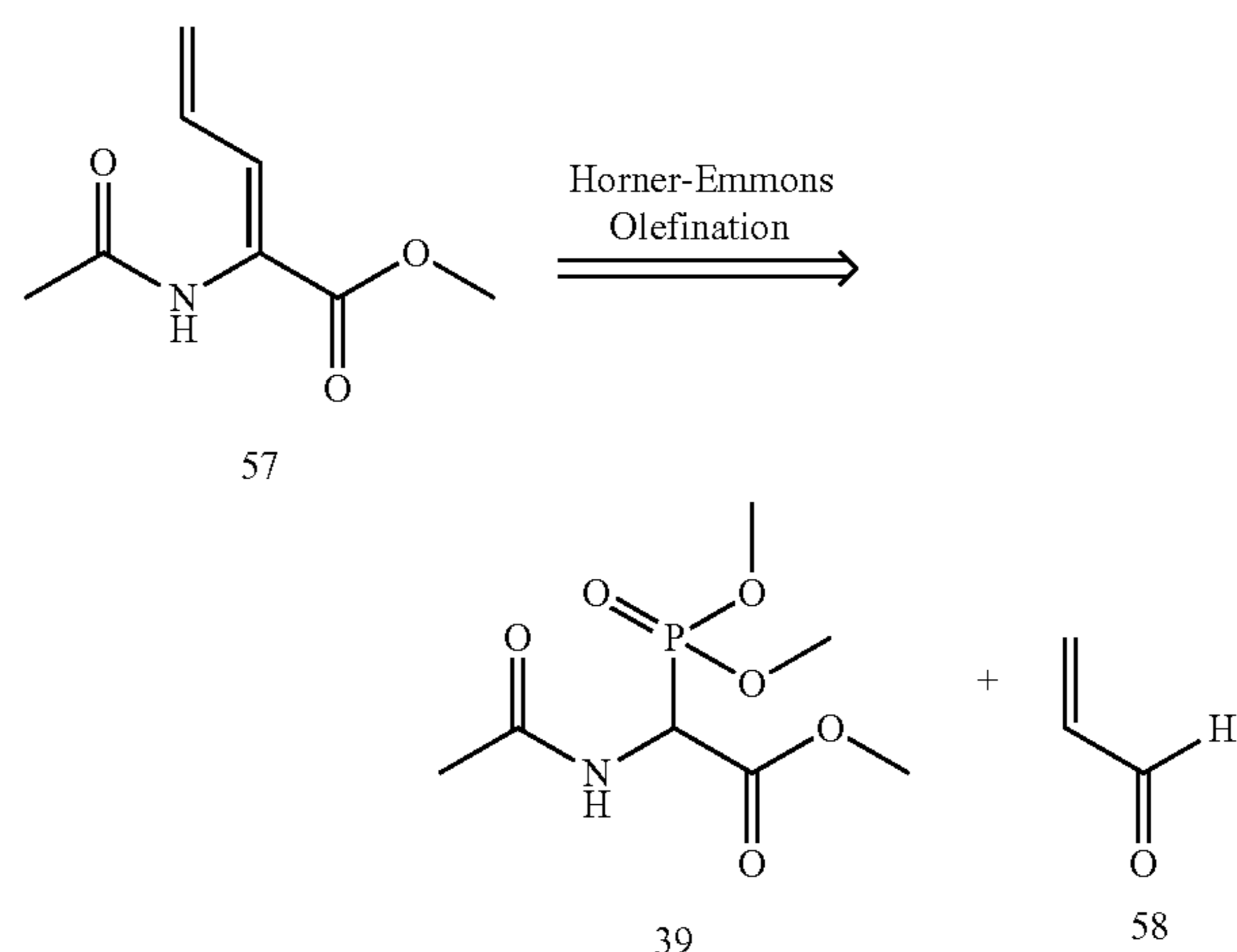
Scheme 4.2
