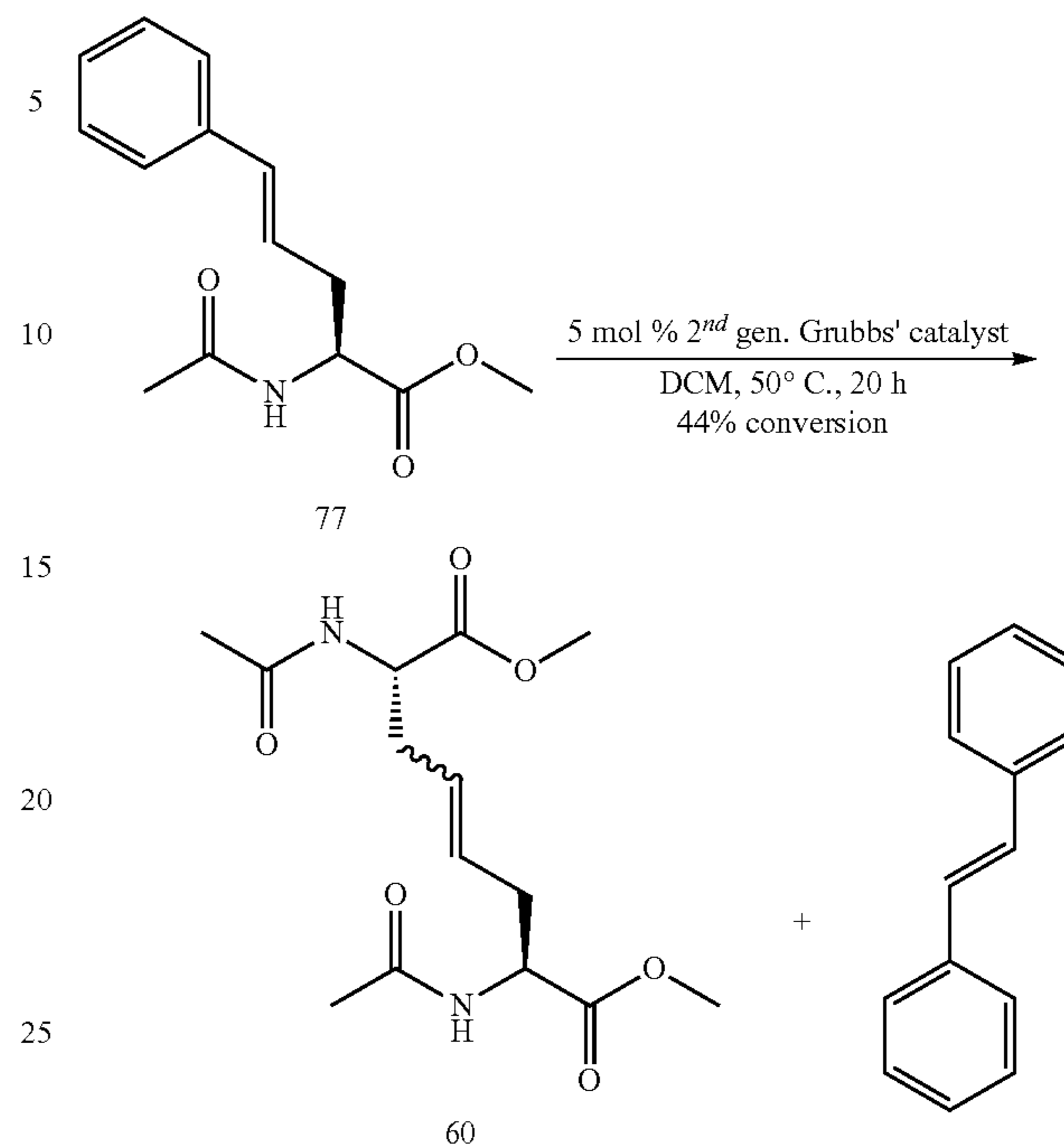
Scheme 4.26
