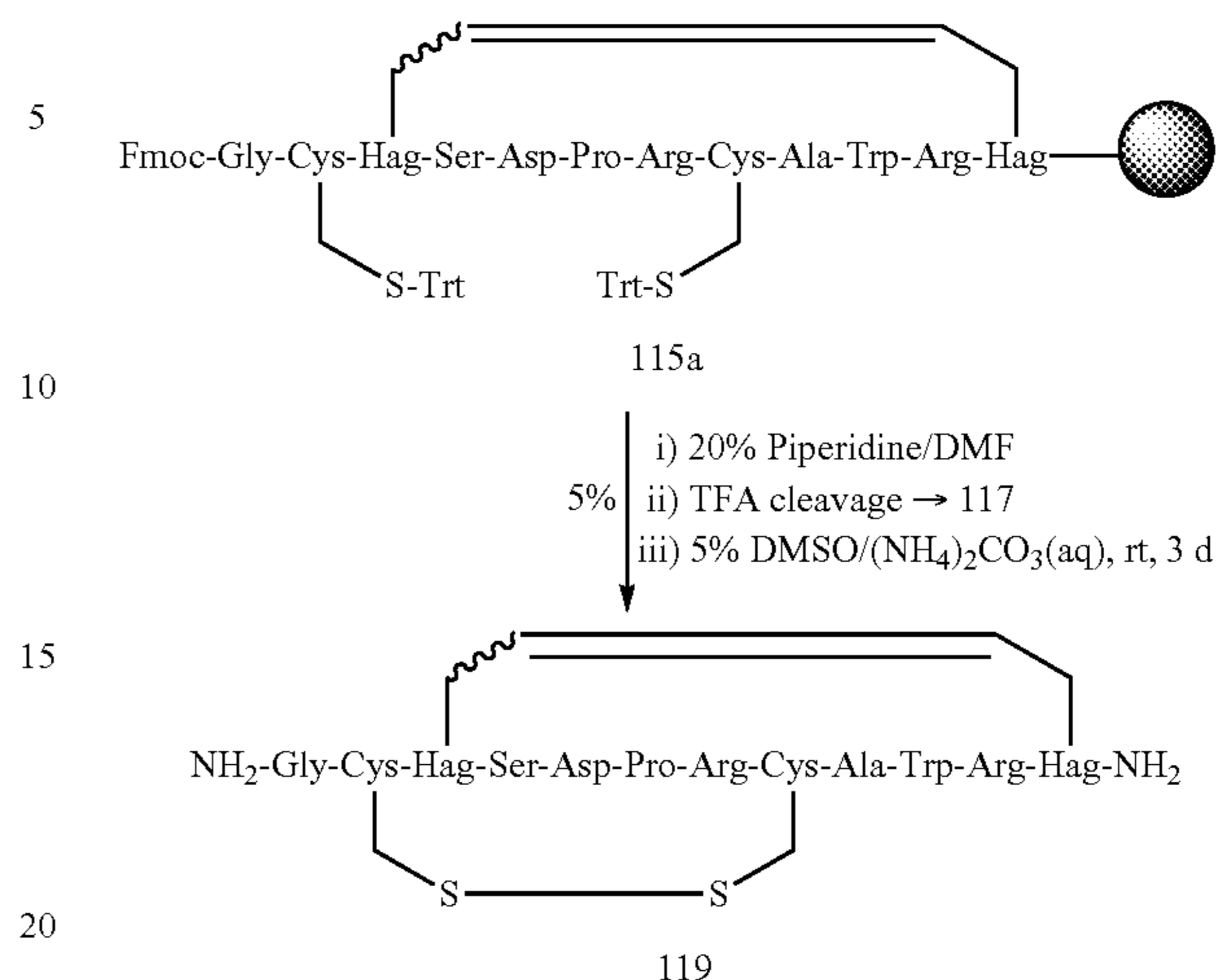
Scheme 6.19
