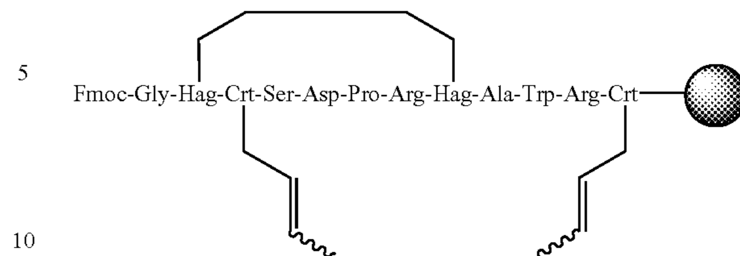
Scheme 6.30
