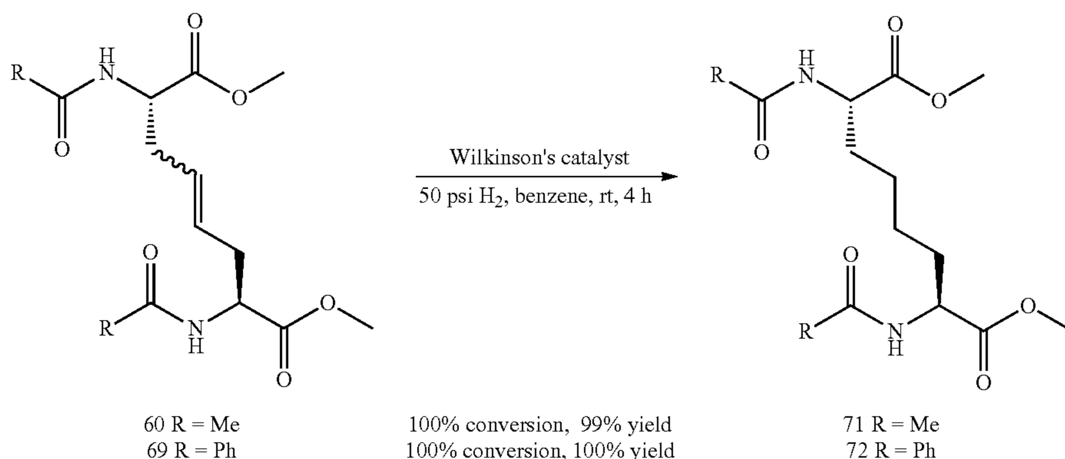
Scheme 4.19
