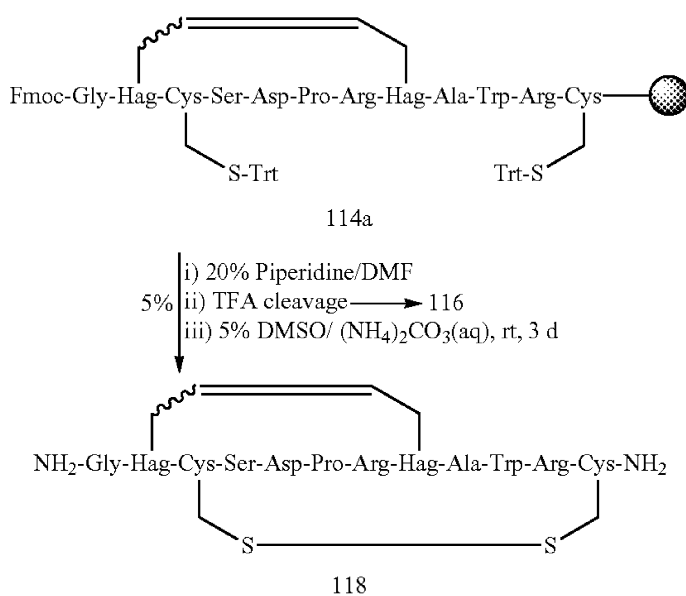
Scheme 6.18
