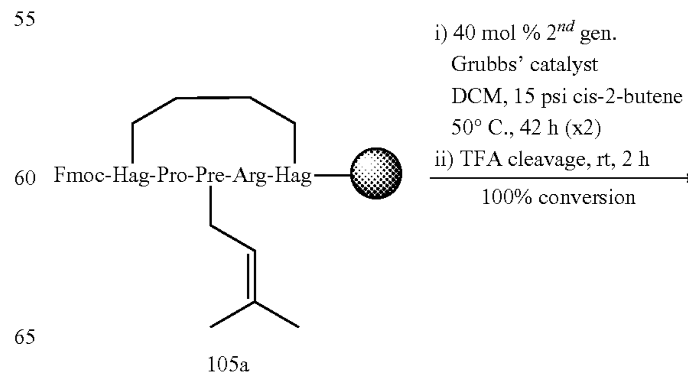
Scheme 6.11
