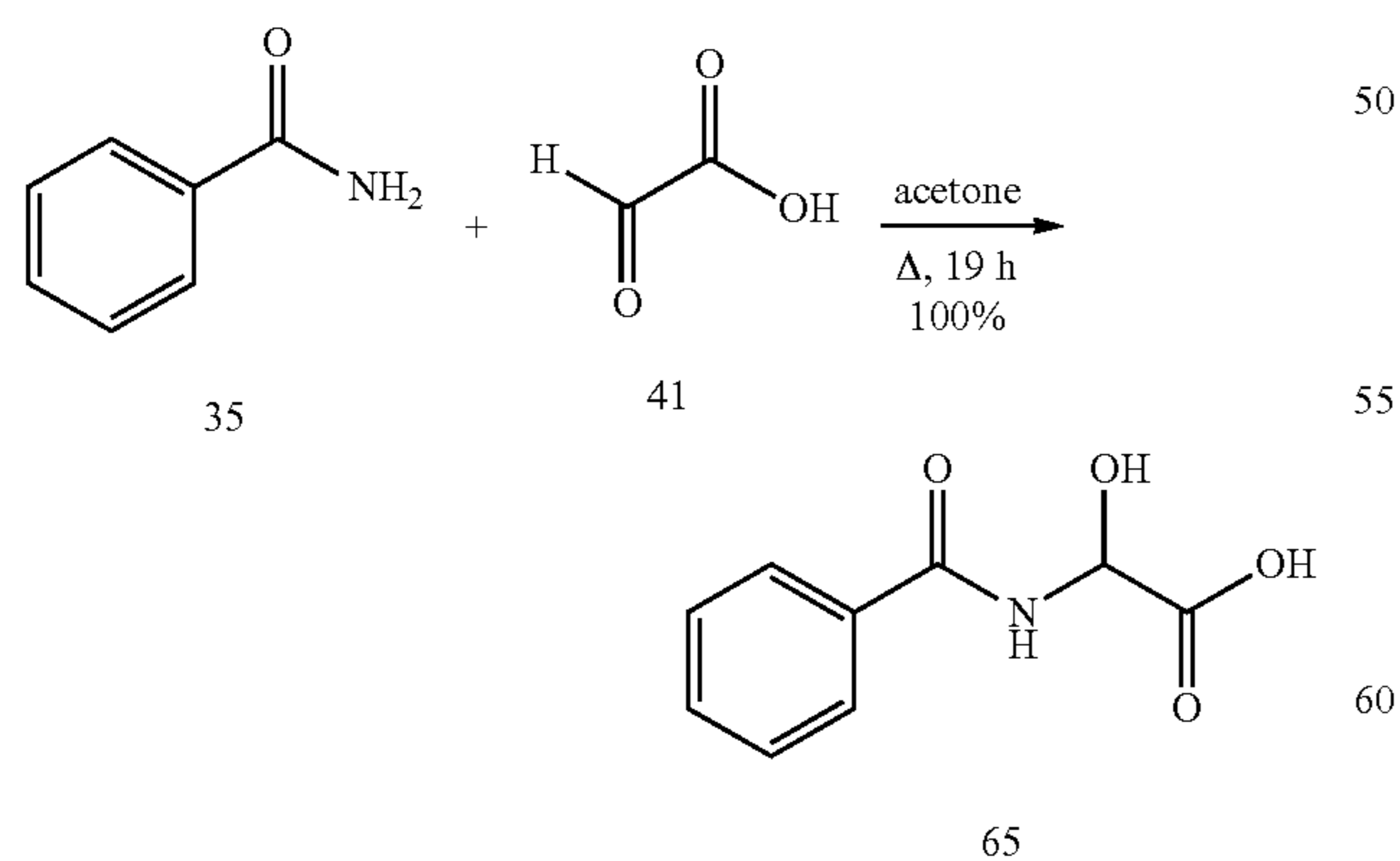
Scheme 4.12
