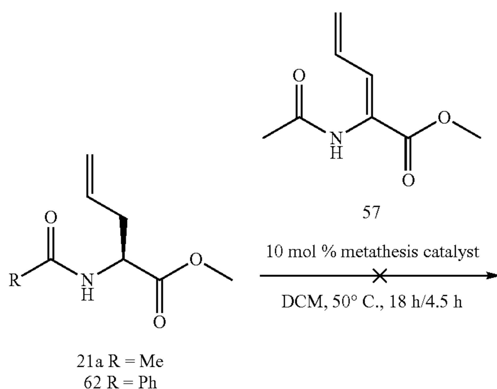
Scheme 4.20
