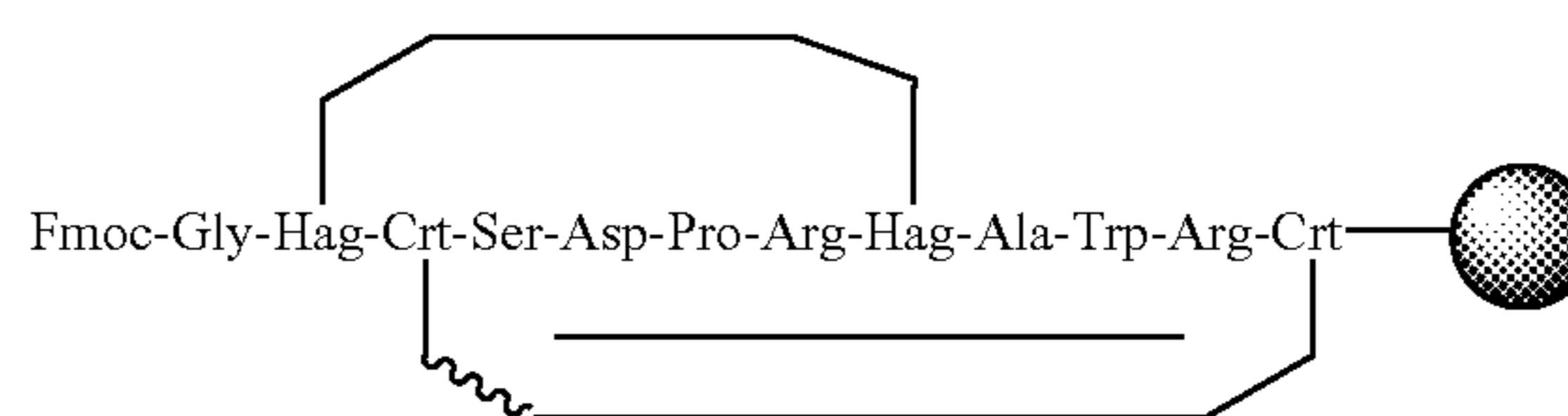
Scheme 6.31
