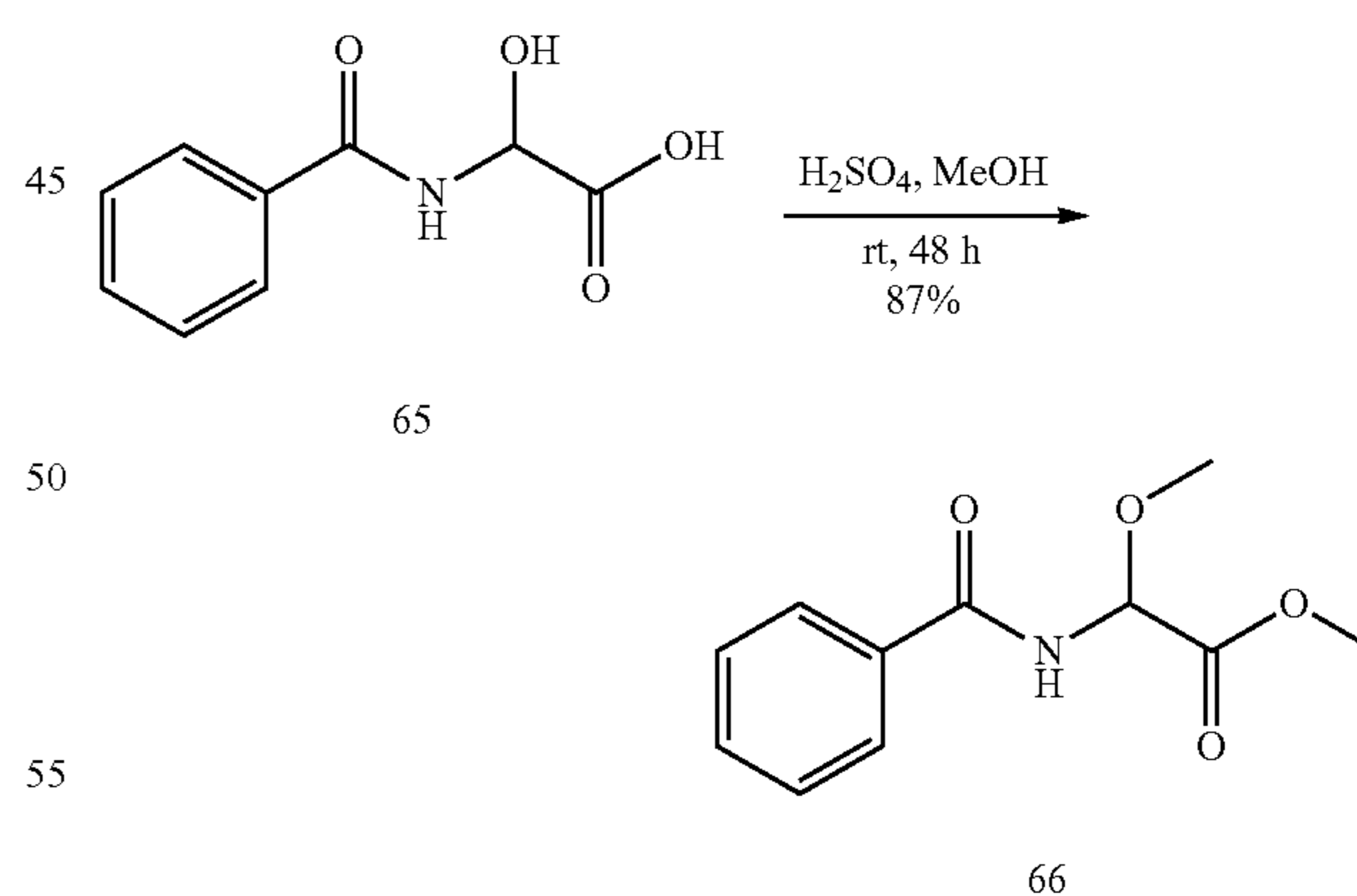
Scheme 4.13
