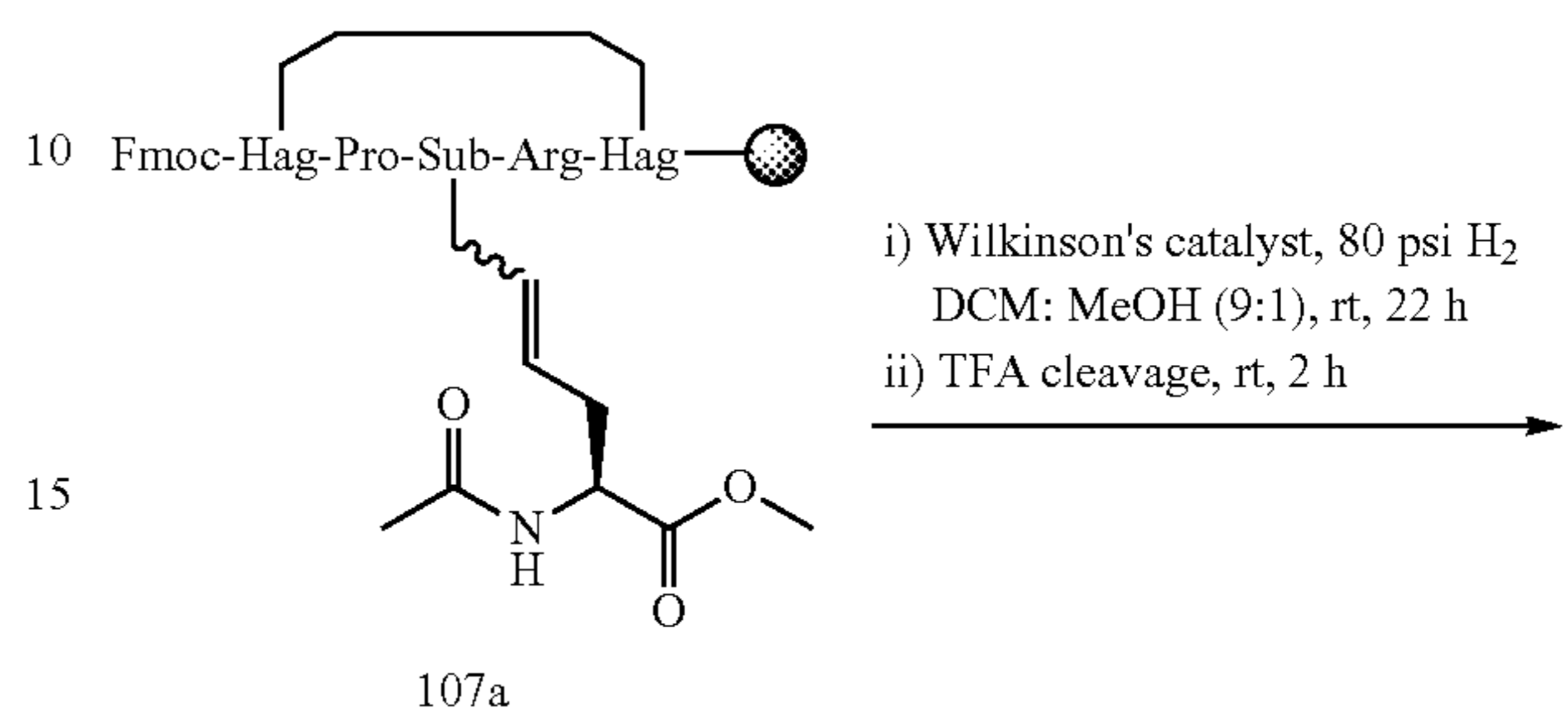
Scheme 6.13
