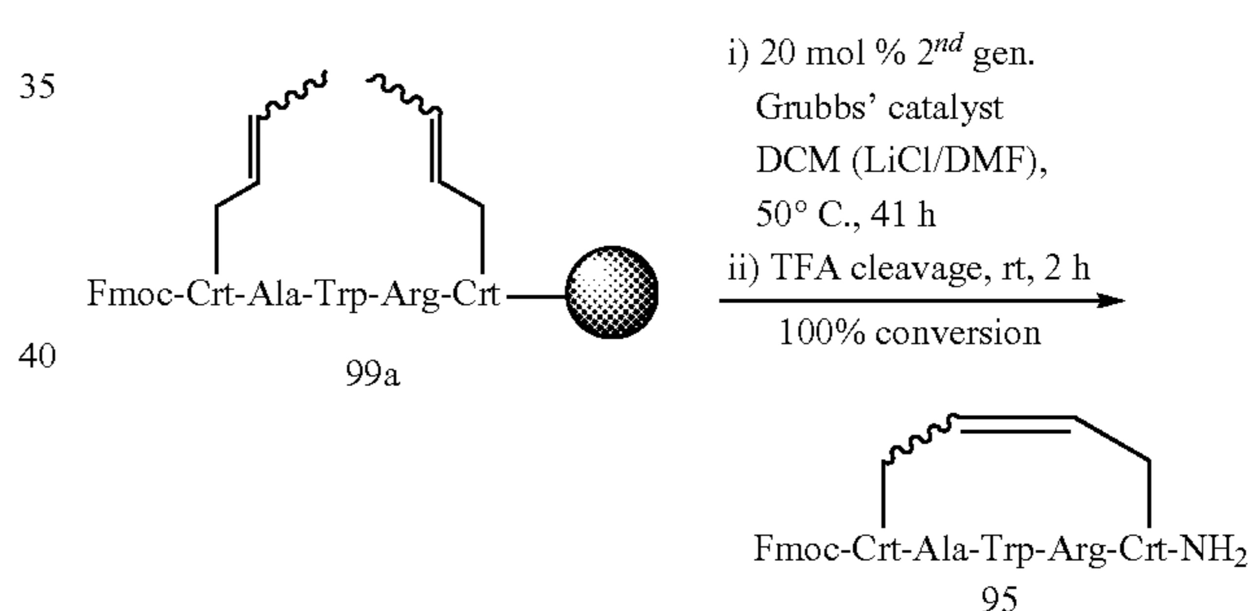
Scheme 6.6
