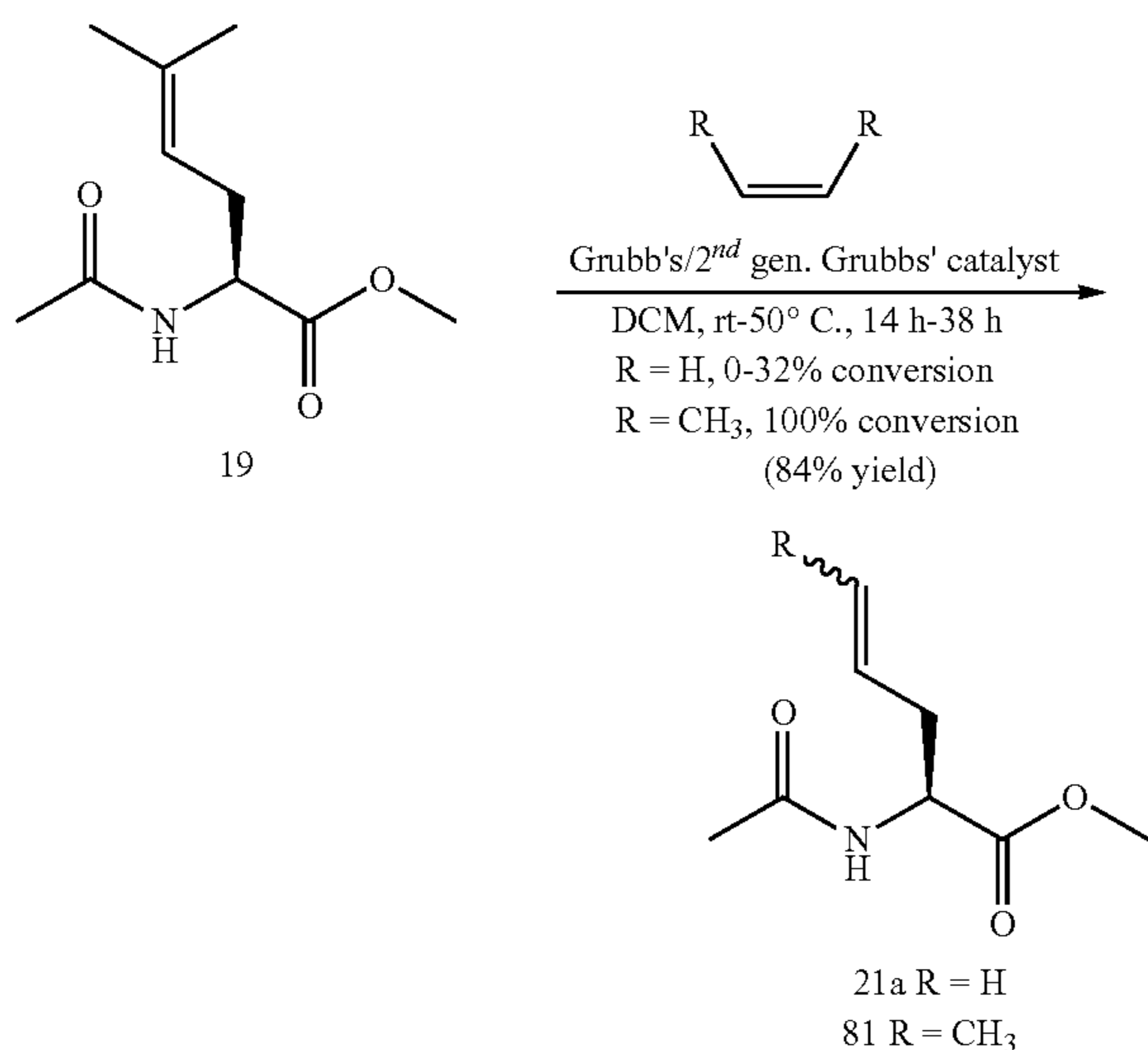
Scheme 4.33
