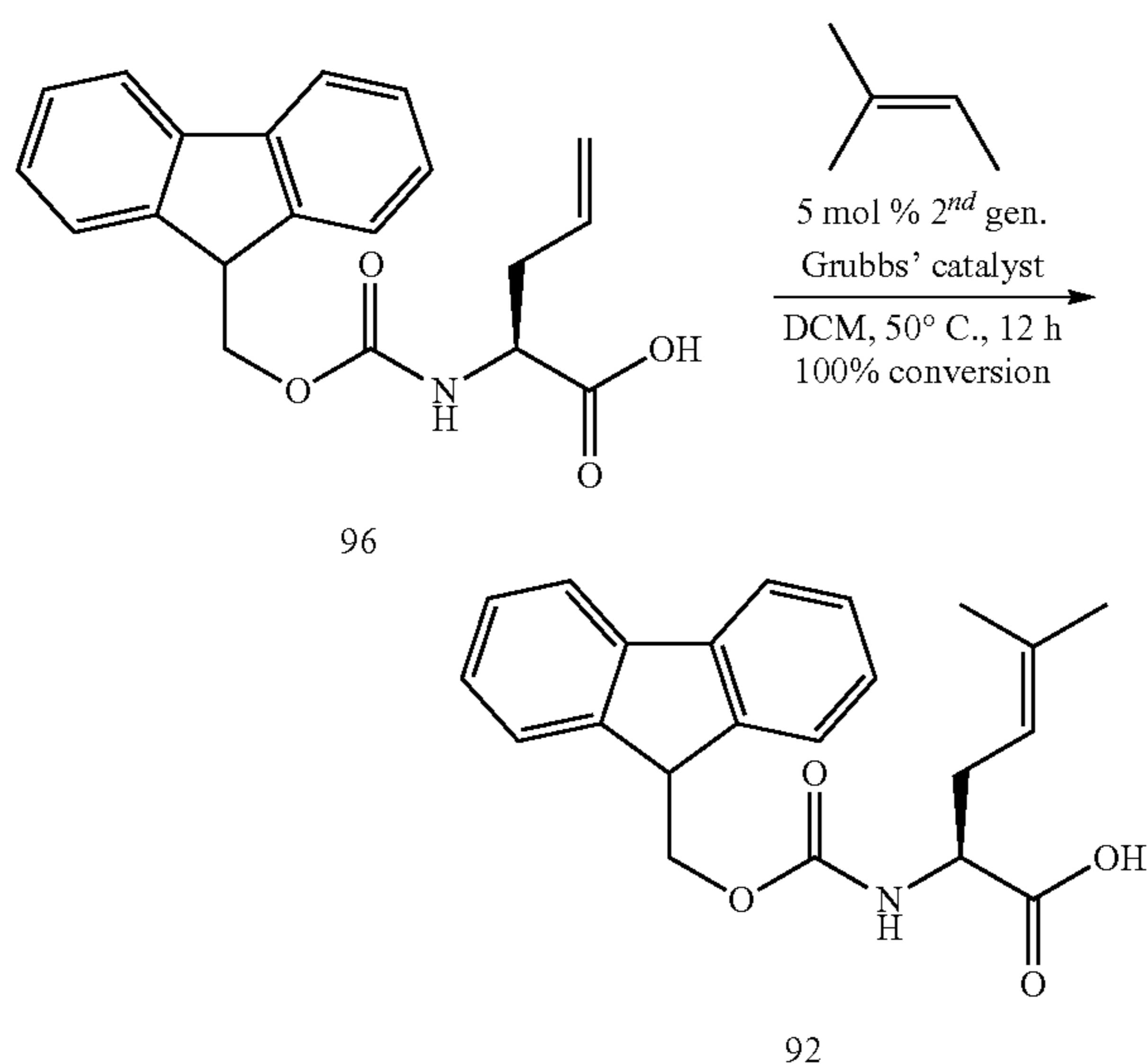
Scheme 6.8
