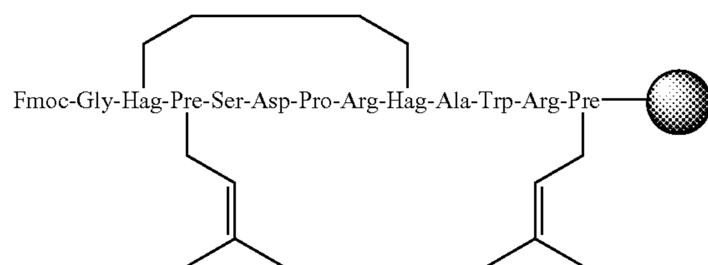
Scheme 6.28
