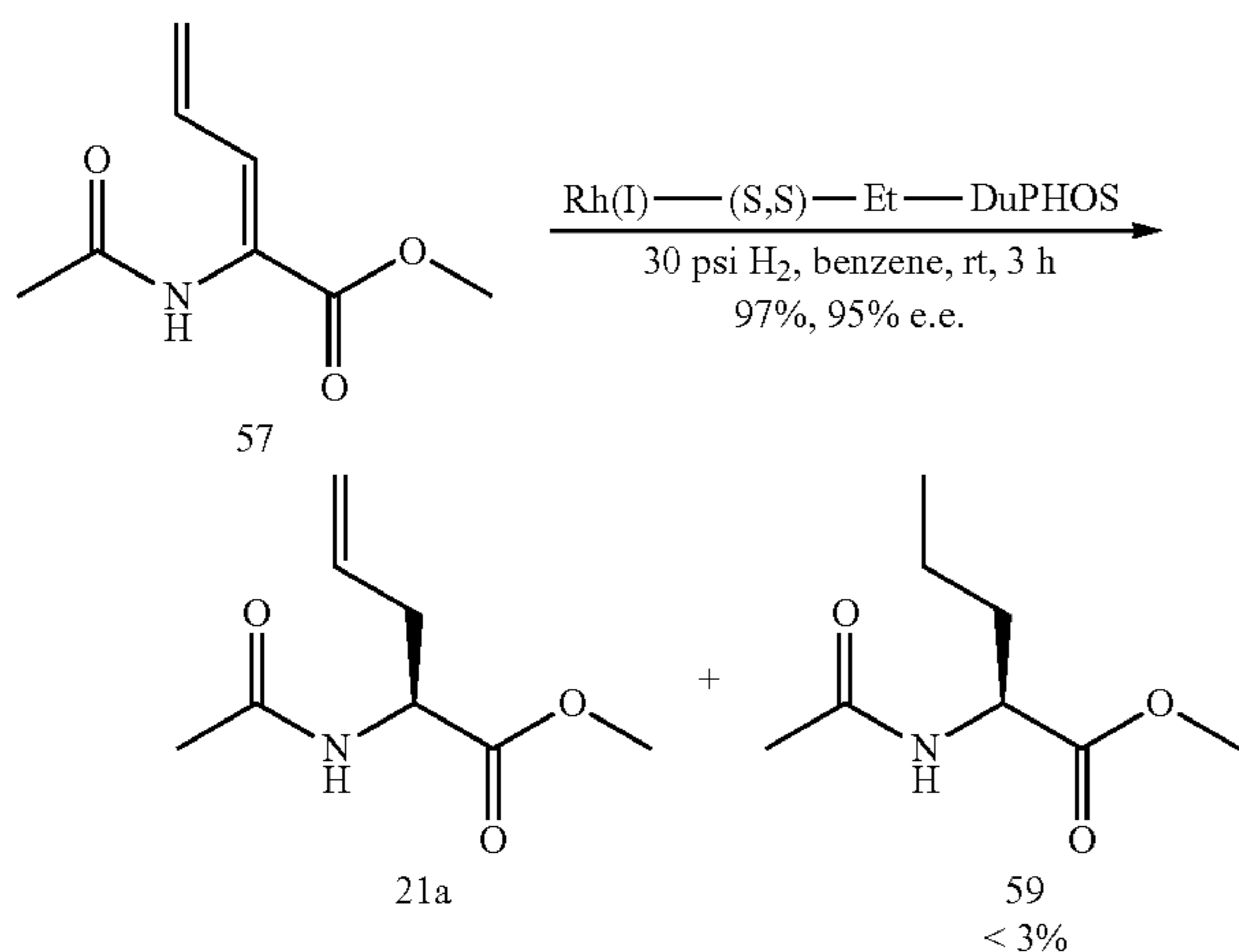
Scheme 4.5
