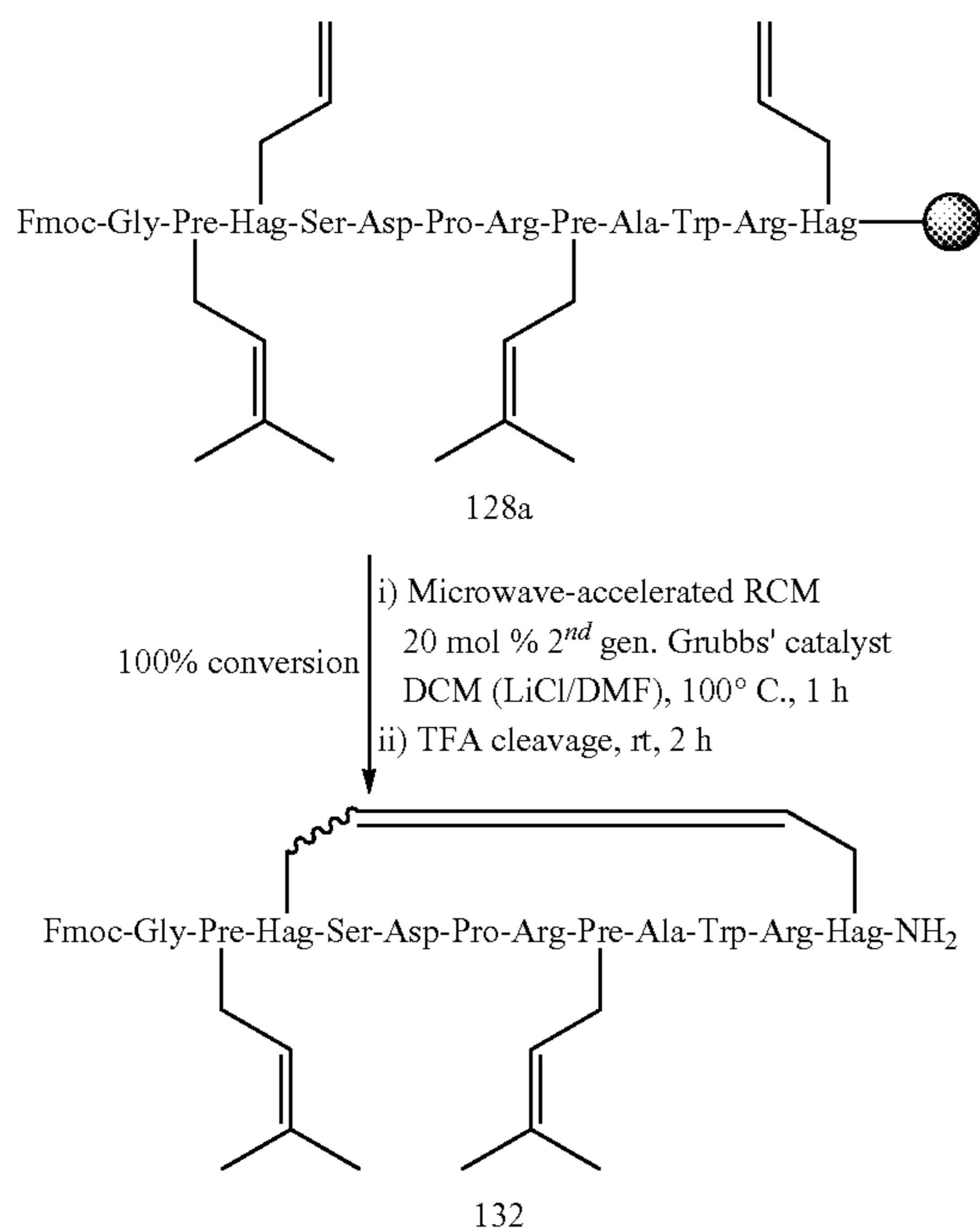
Scheme 6.25
