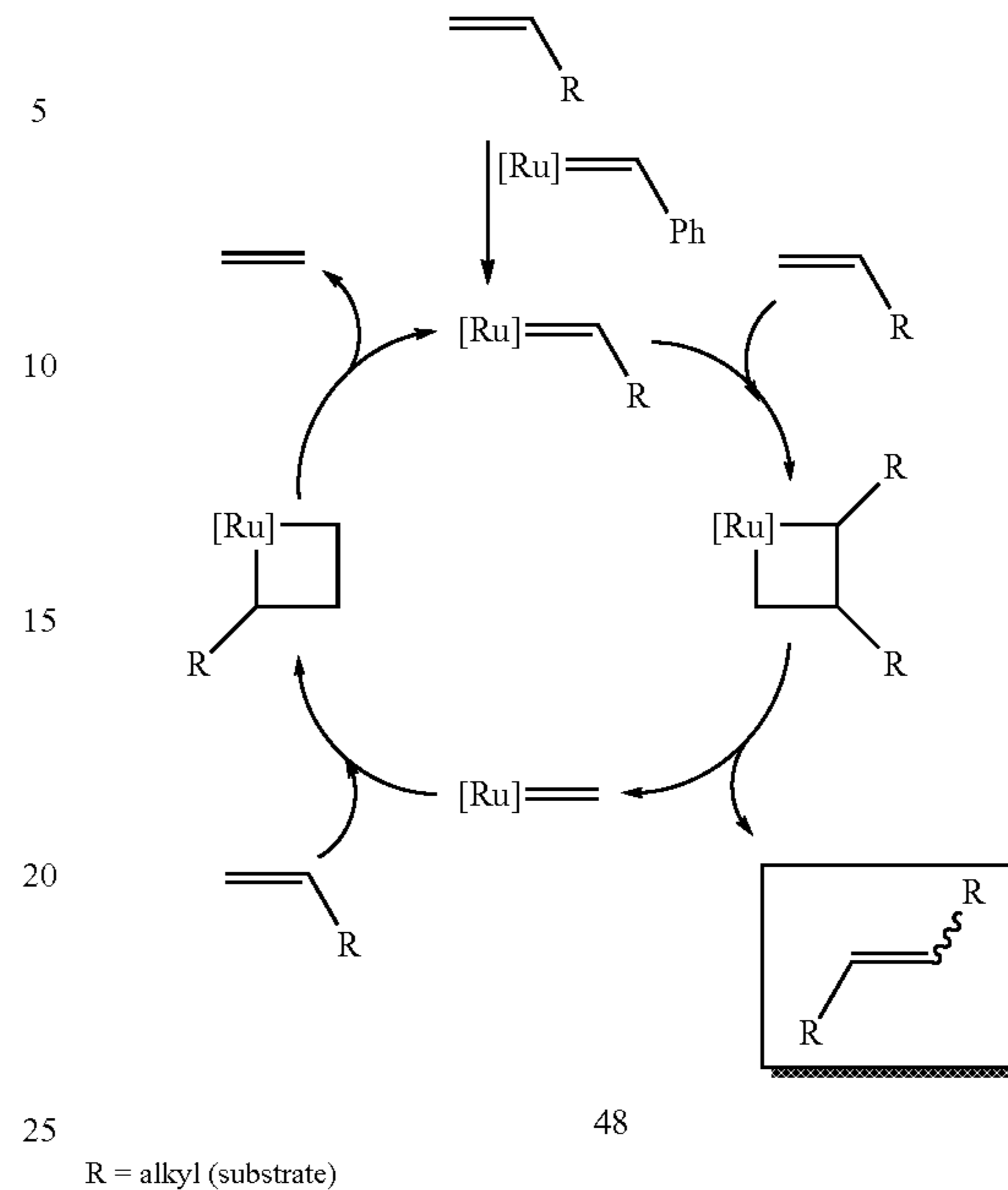
Scheme 4.7
