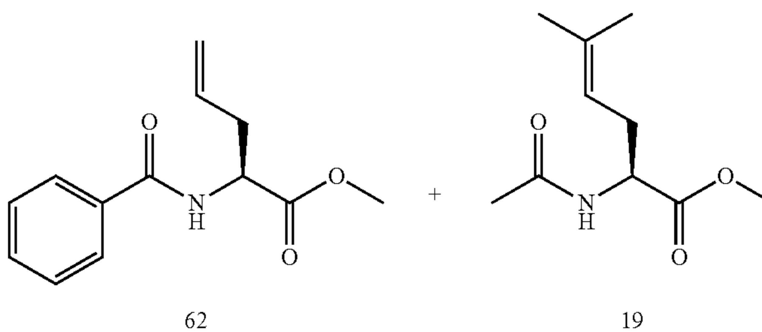
Scheme 4.35
