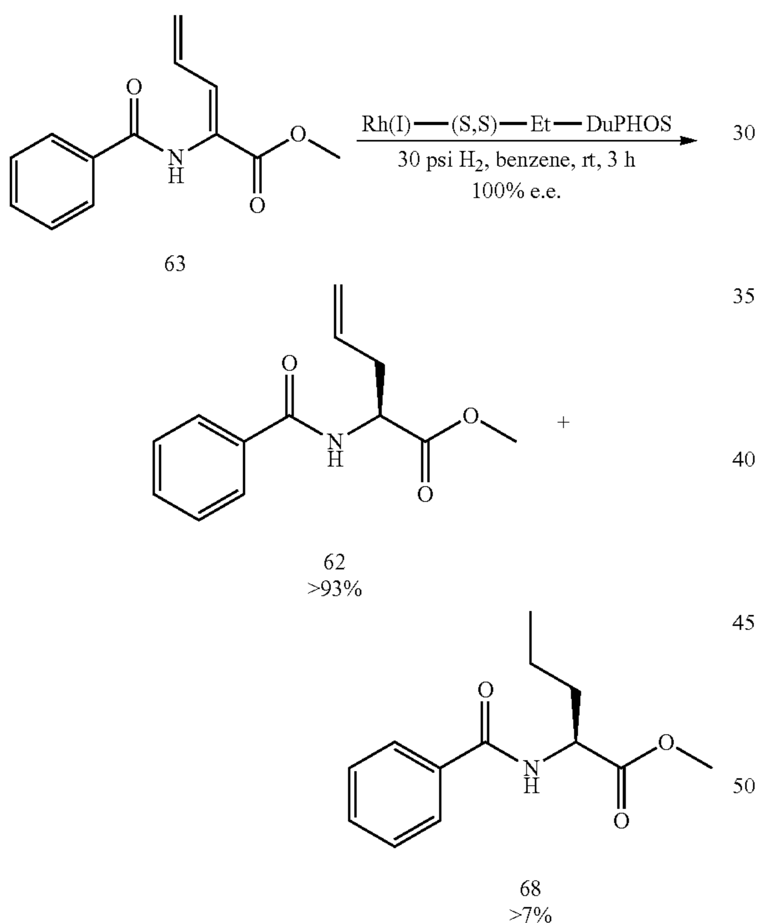
Scheme 4.16
