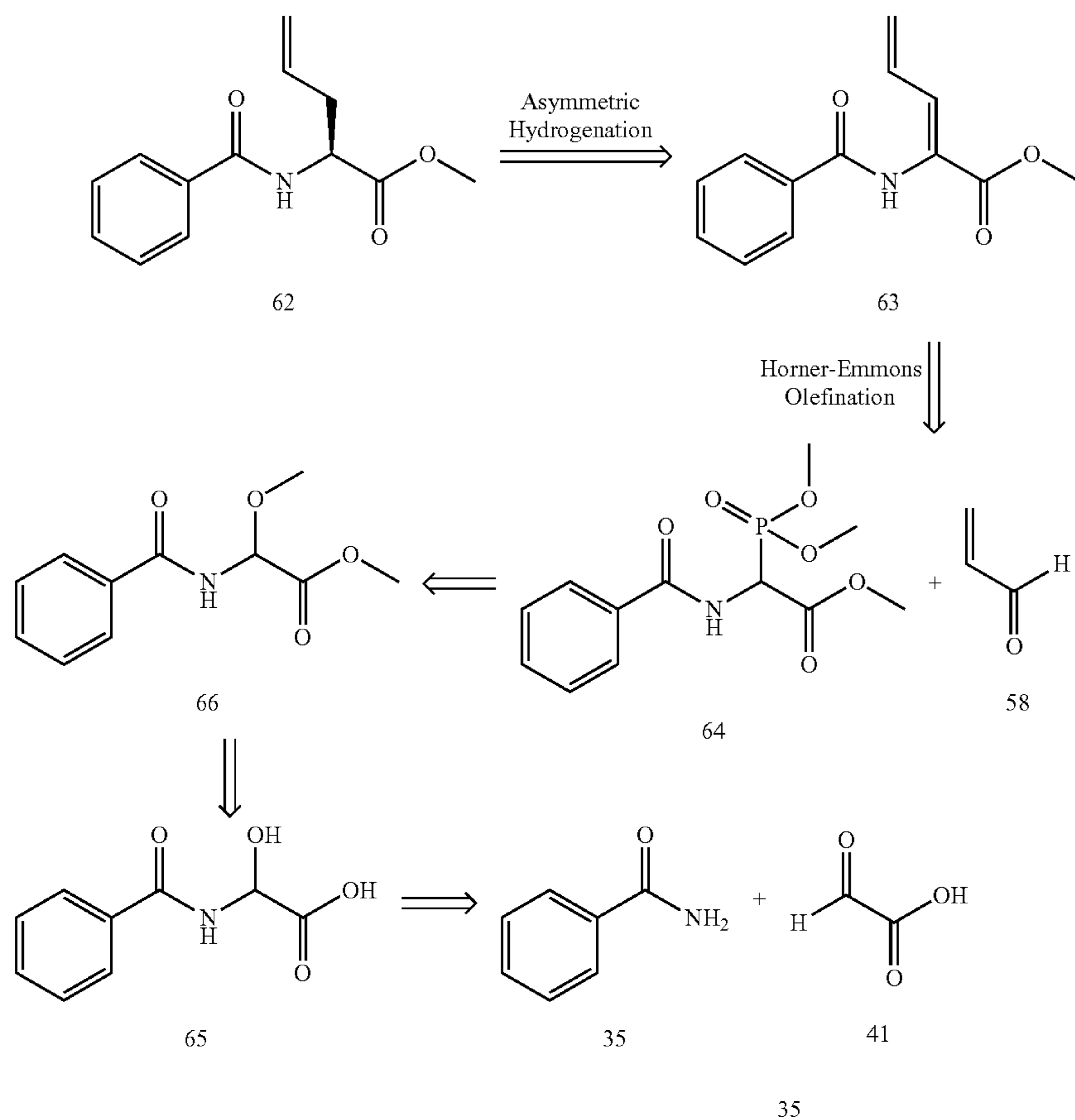
Scheme 4.11
