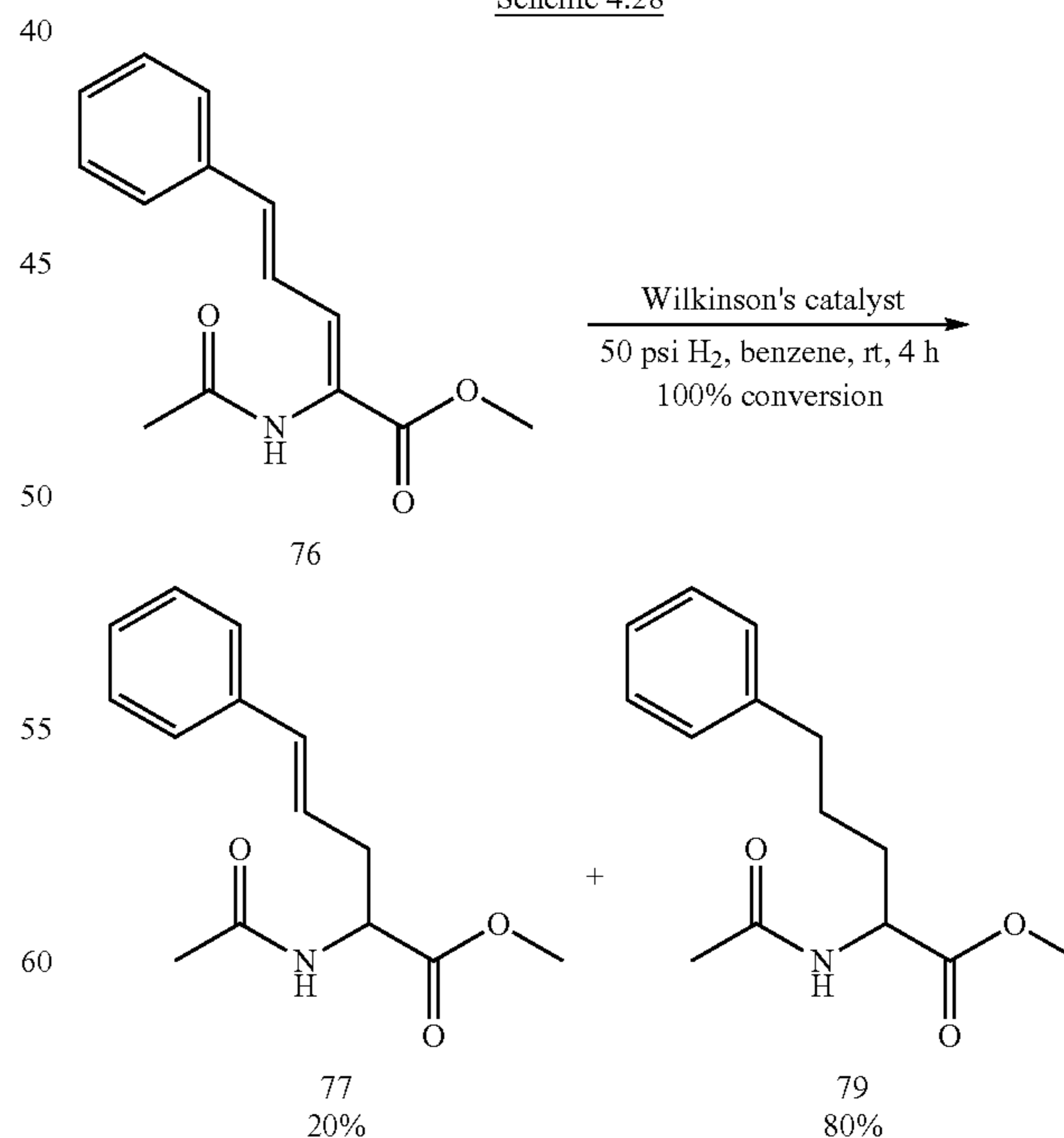
Scheme 4.28
