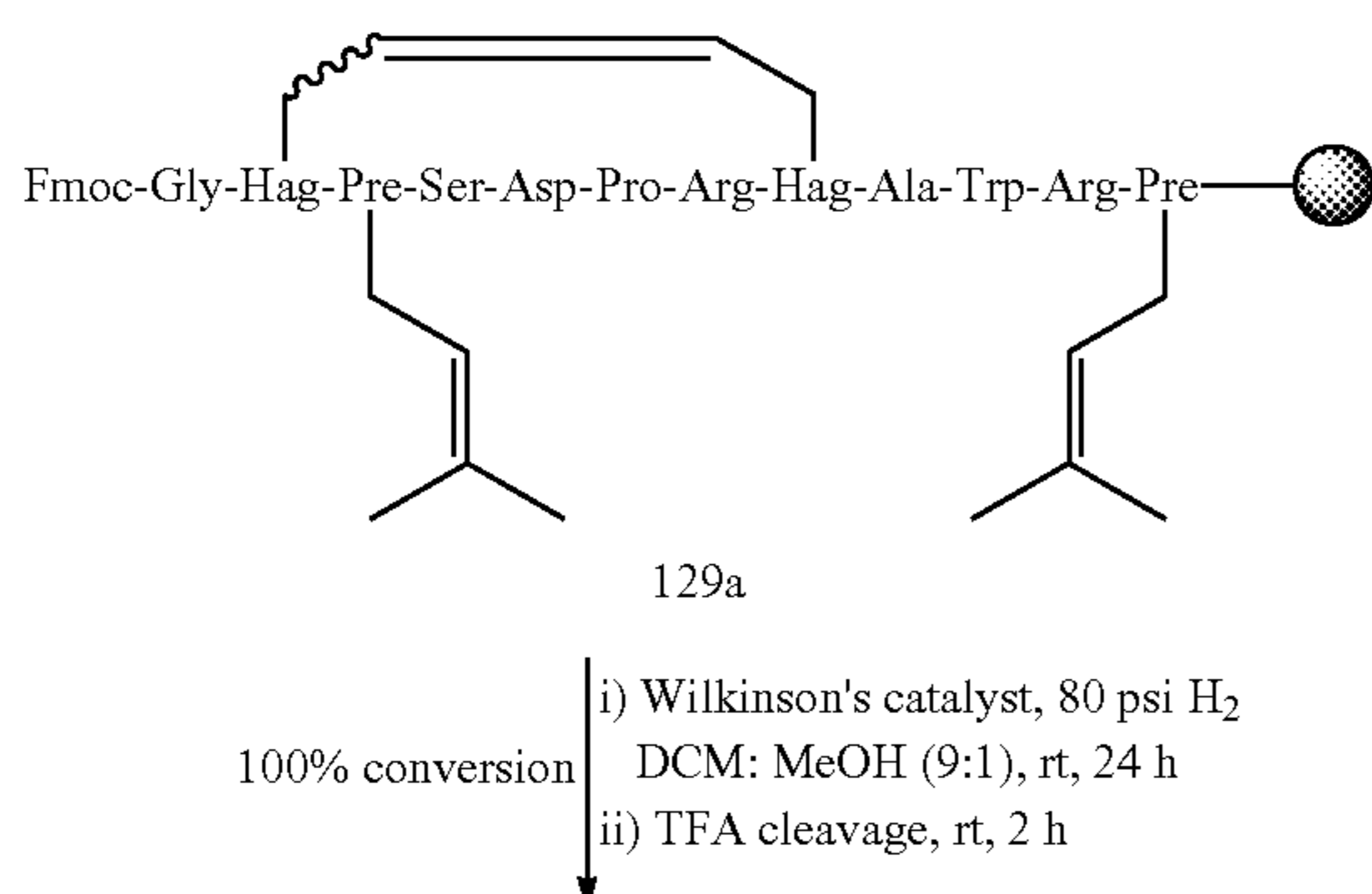
Scheme 6.26
