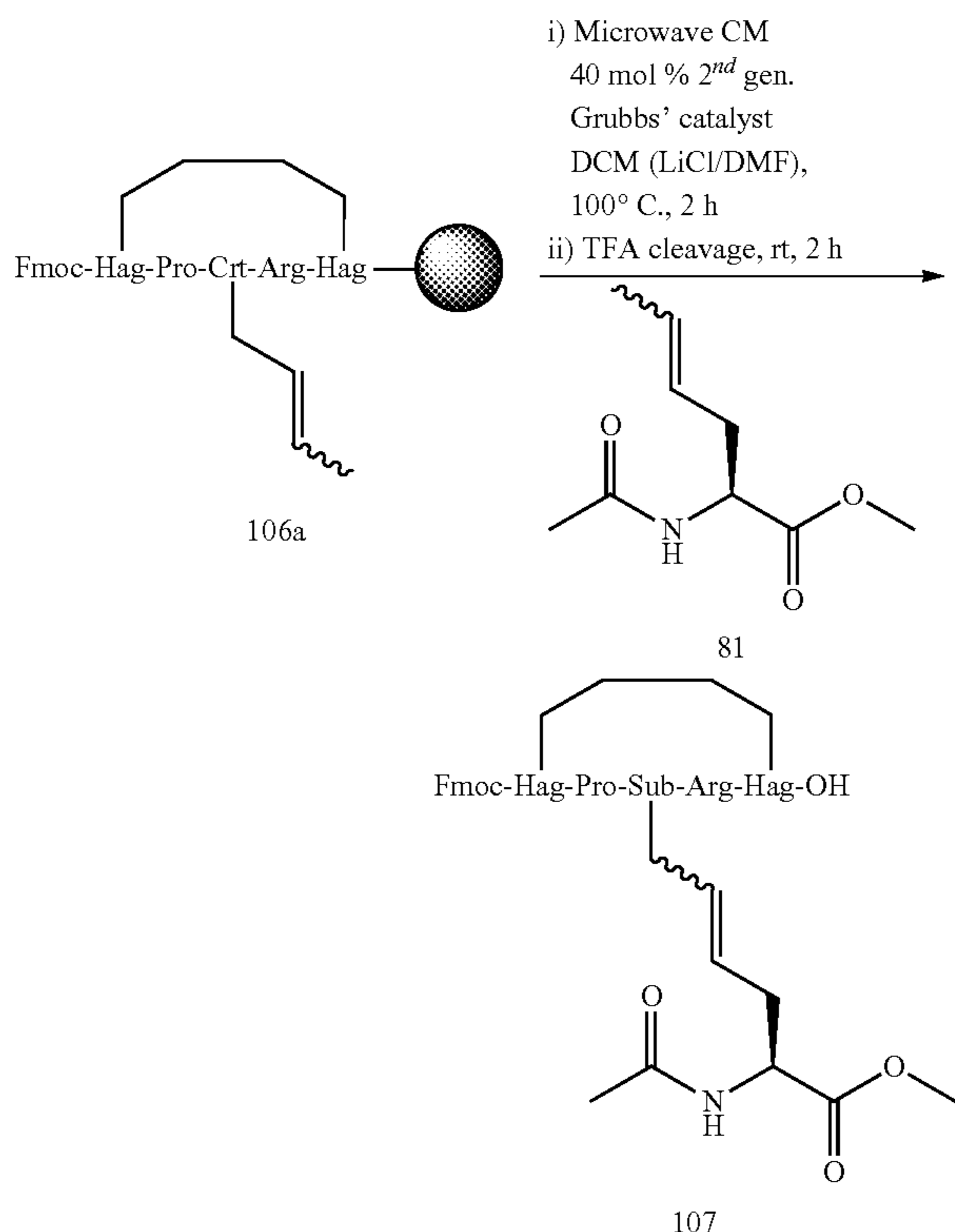
Scheme 6.12
