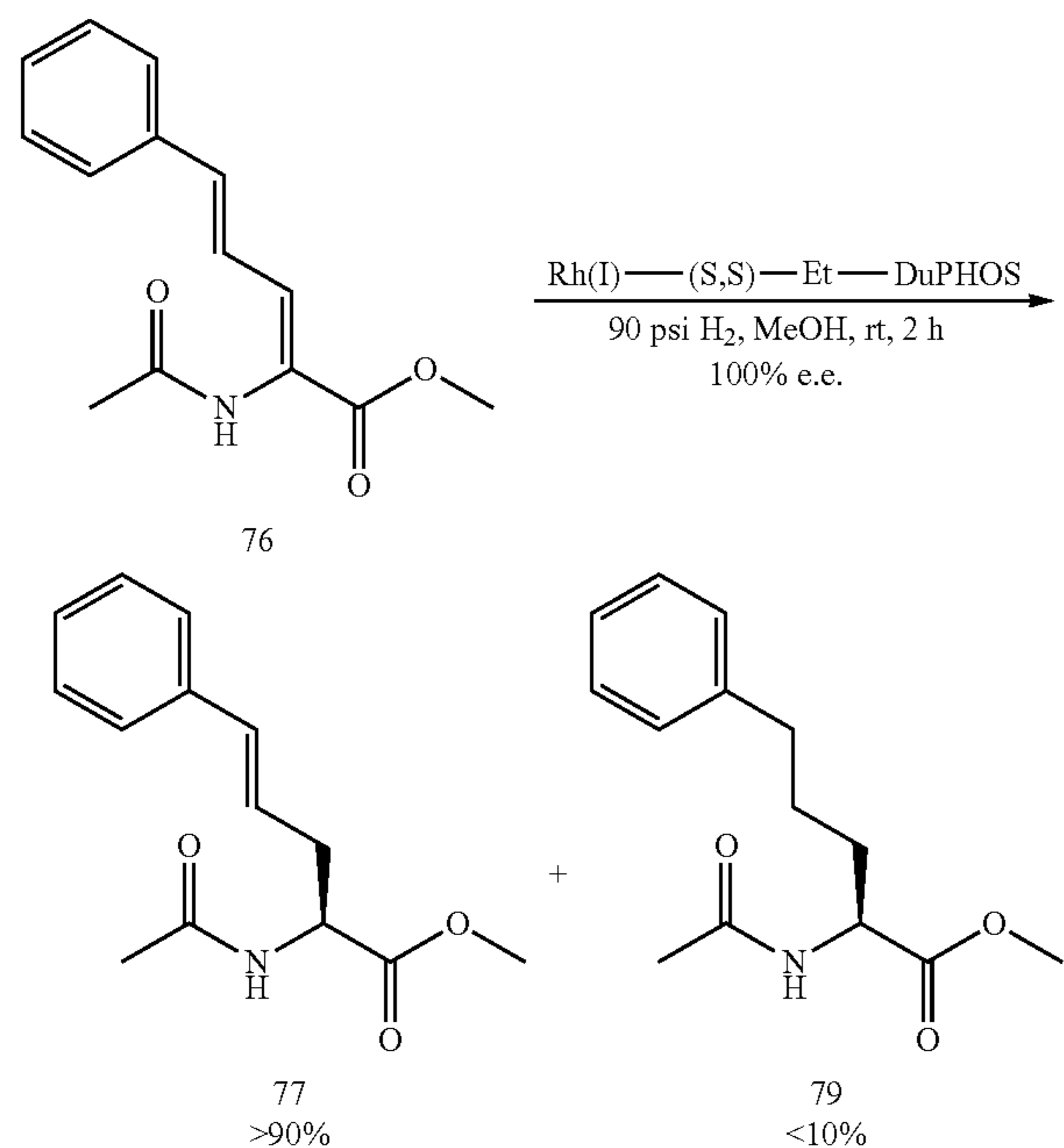
Scheme 4.25
