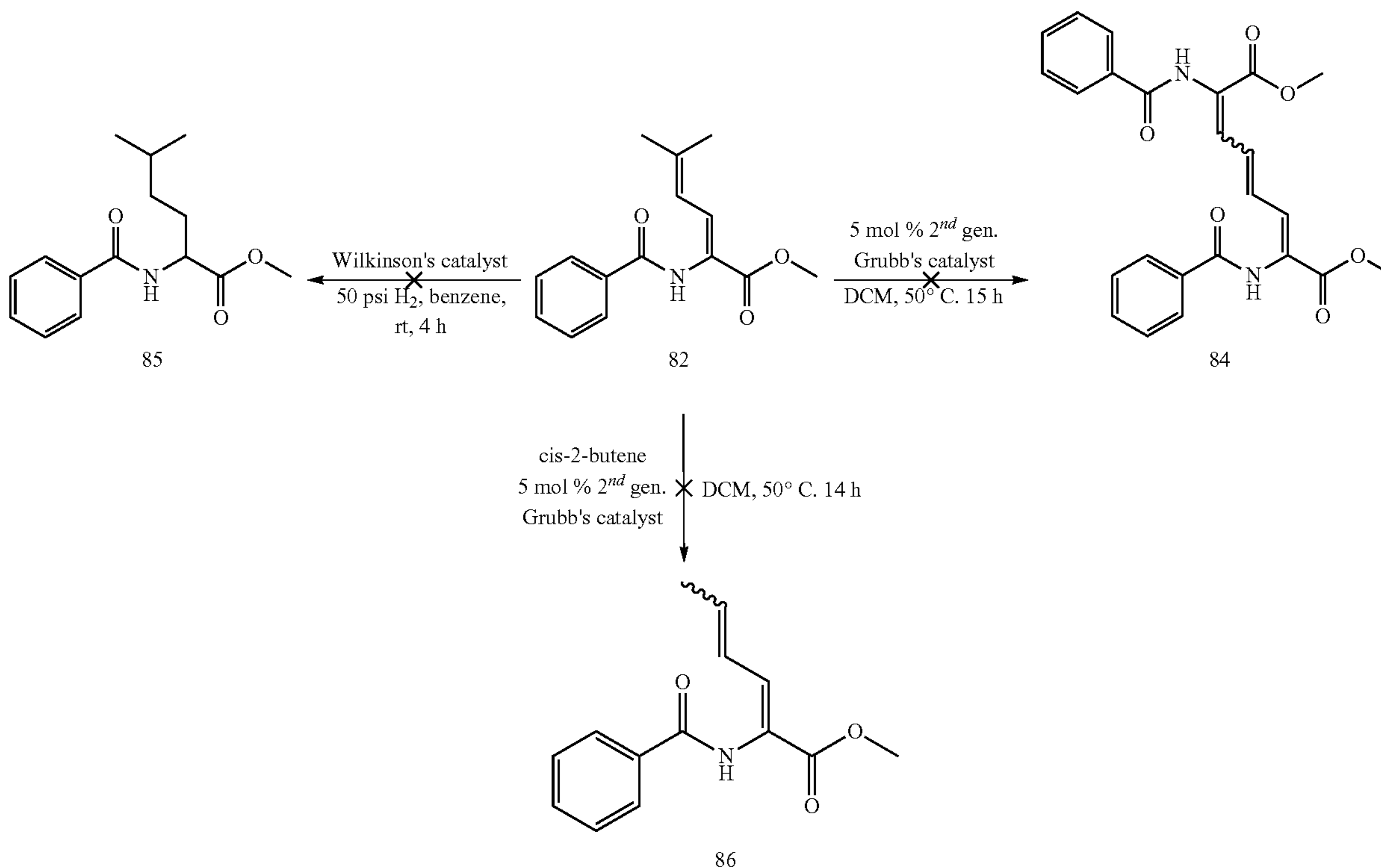
Scheme 5.3
