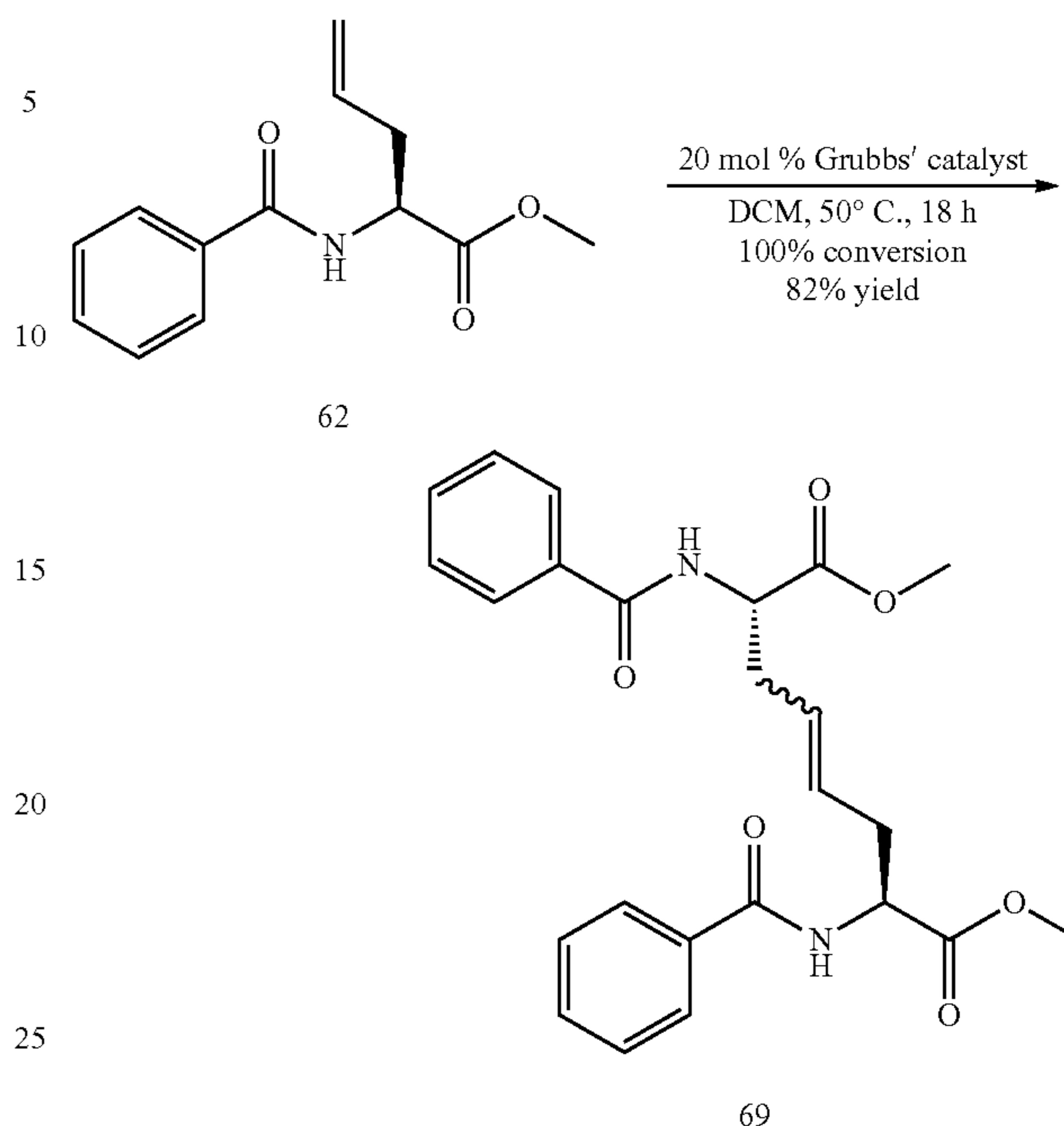
Scheme 4.17
