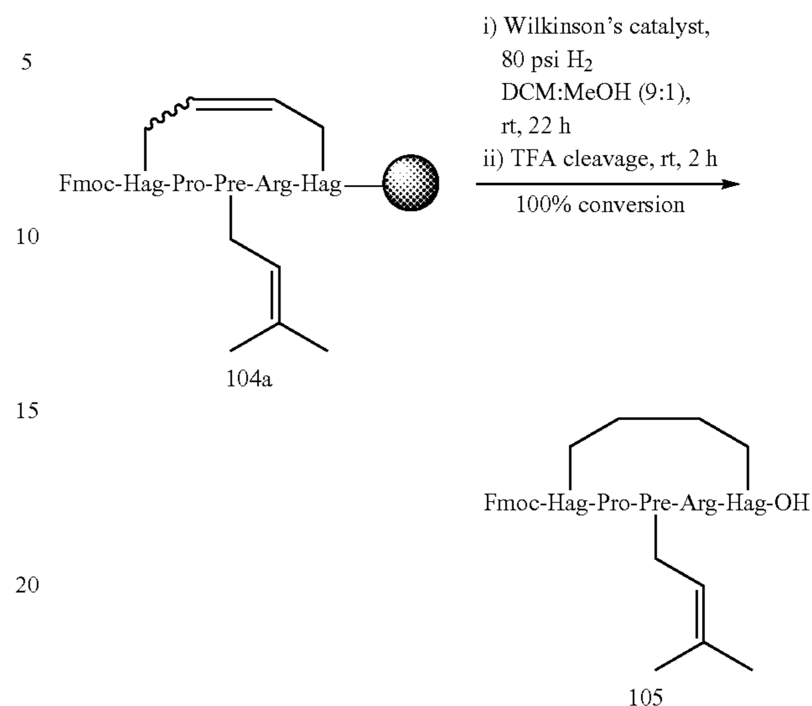
Scheme 6.10
