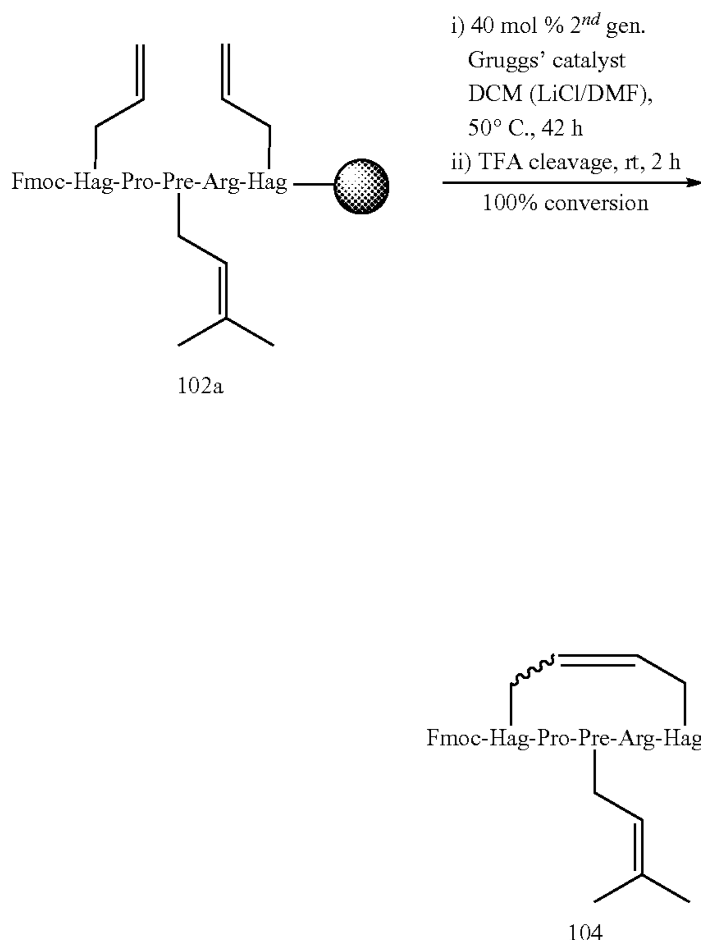
Scheme 6.9
