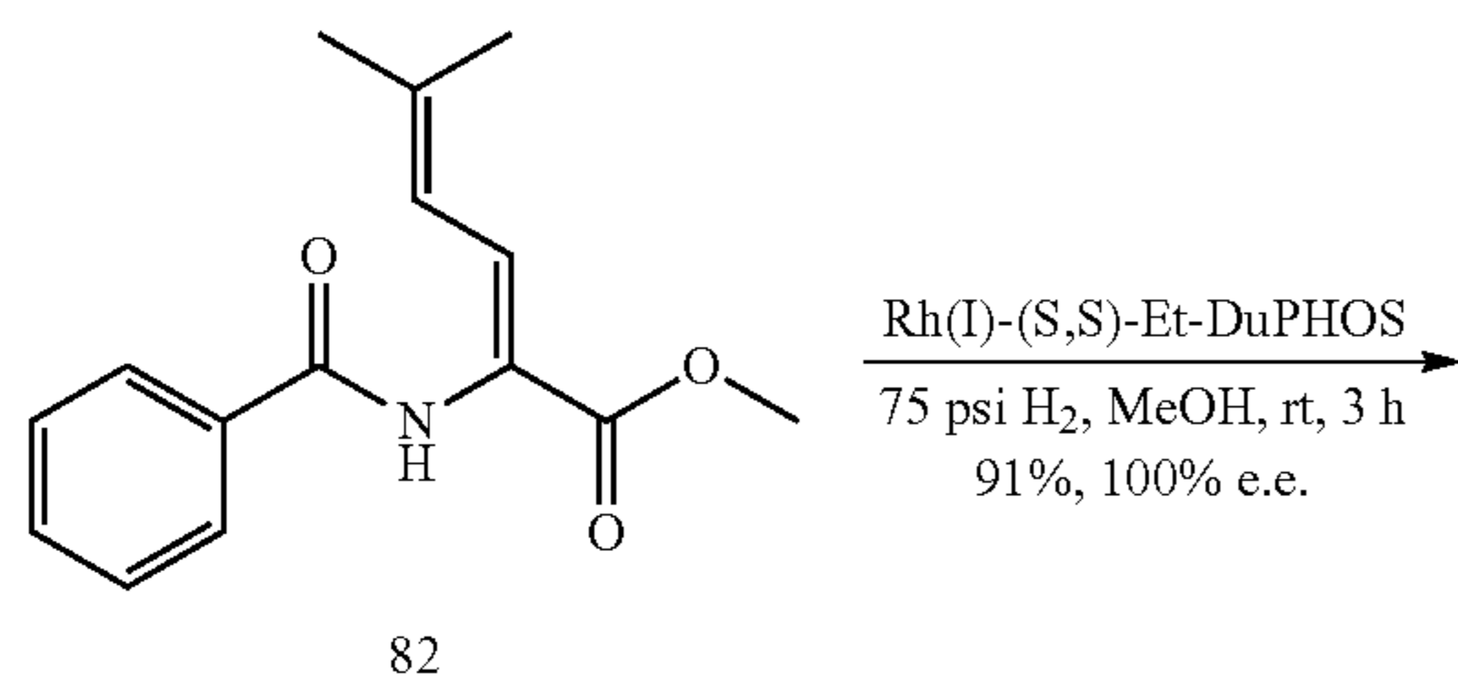
Scheme 5.4
