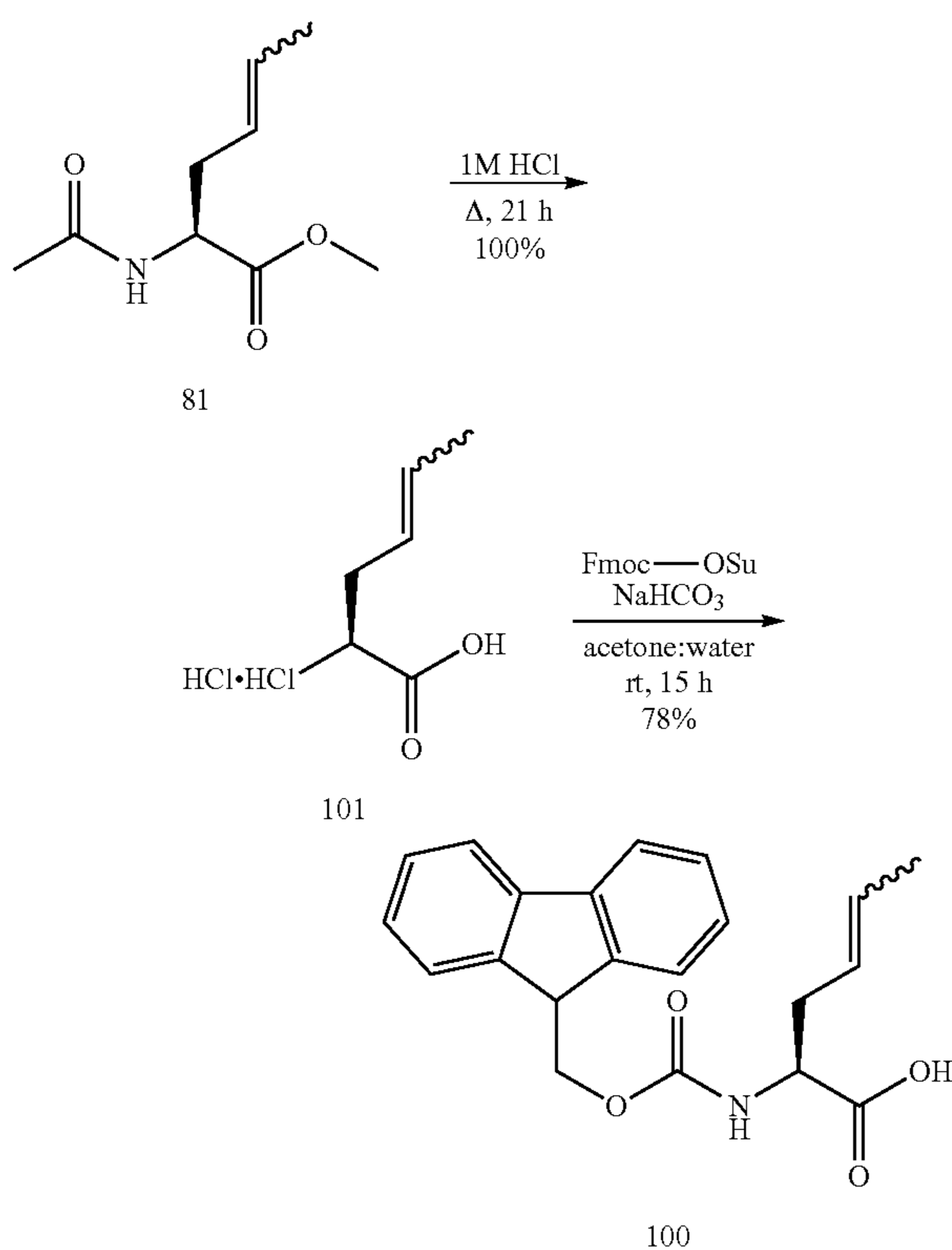
Scheme 6.5
