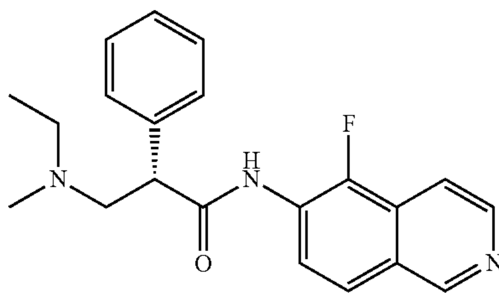
(2S)-3-(ethyl(methyl)amino)-N-(5-fluoroisoquinolin-6-yl)-2-phenylbutanamide
