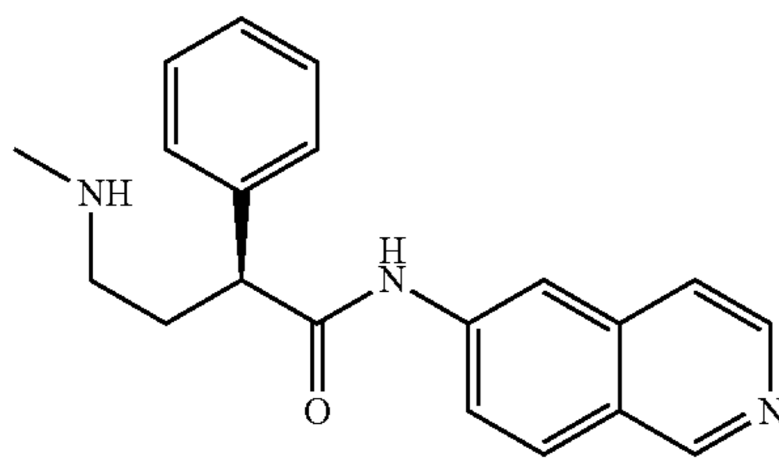
(S)-N-(isoquinolin-6-yl)-4-(methylamino)-2-phenylbutanamide
