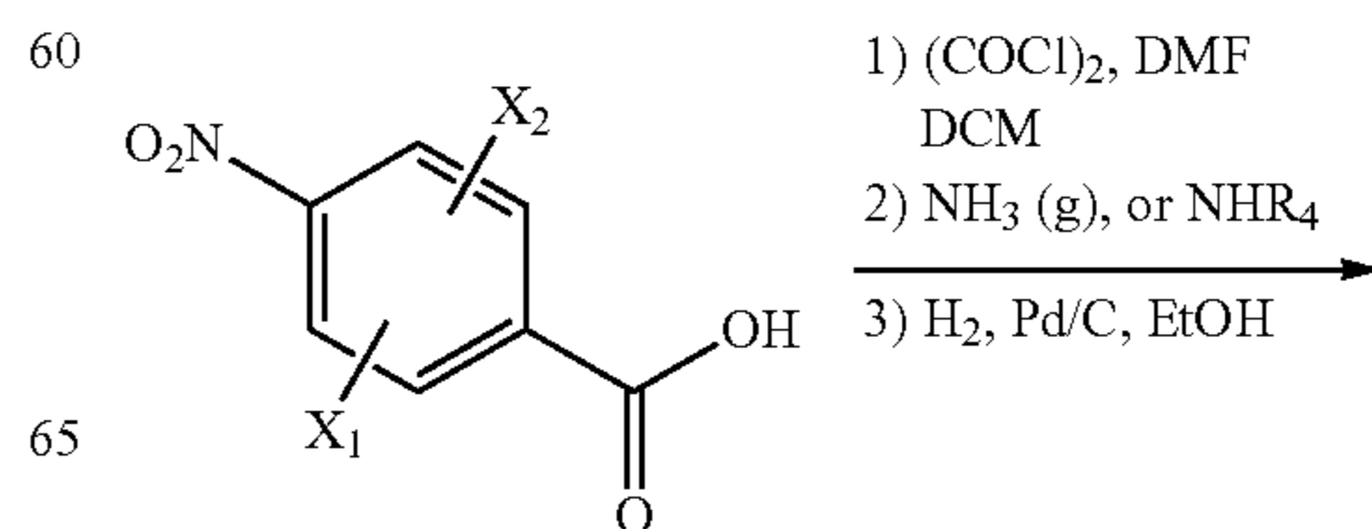
Scheme 6
