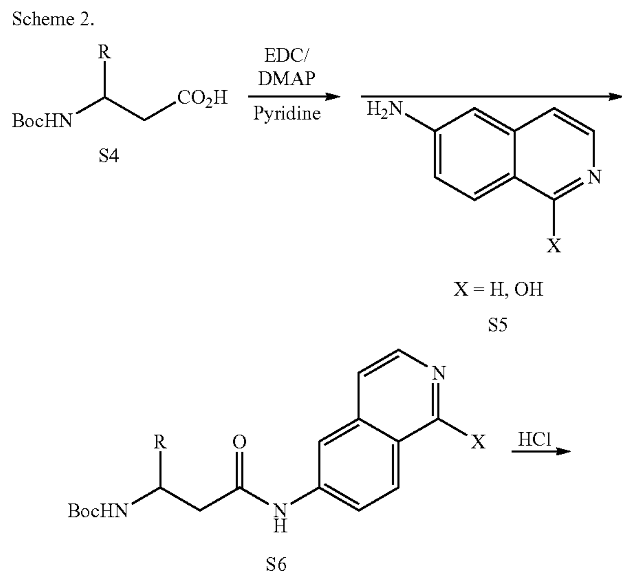
Scheme 2
