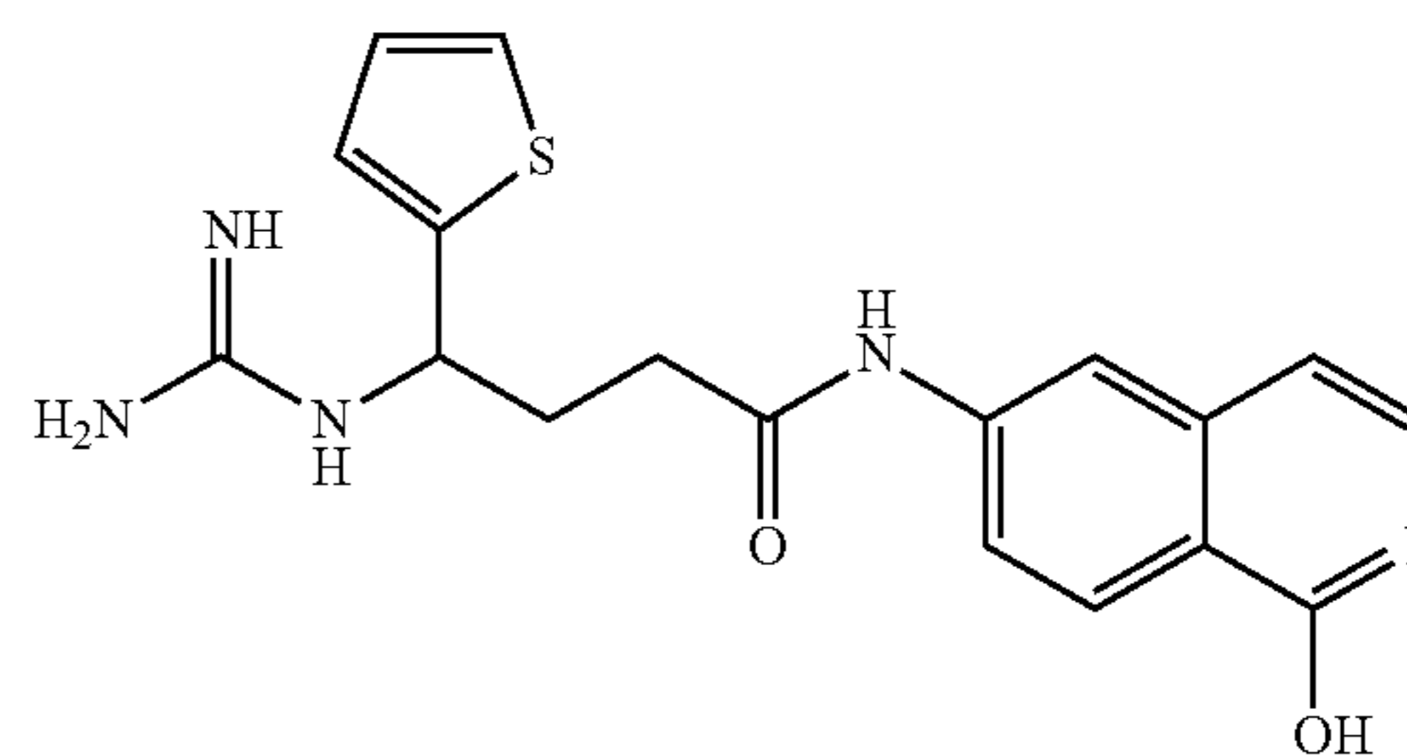
4-guanidino-N-(1-hydroxyisoquinolin-6-yl)-4-(thiophen-2-yl)butanamide
