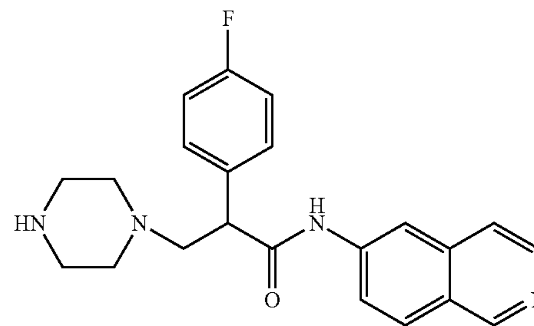
2-(4-fluorophenyl)-N-(isoquinolin-6-yl)-3-(piperazin-1-yl)propanamide
