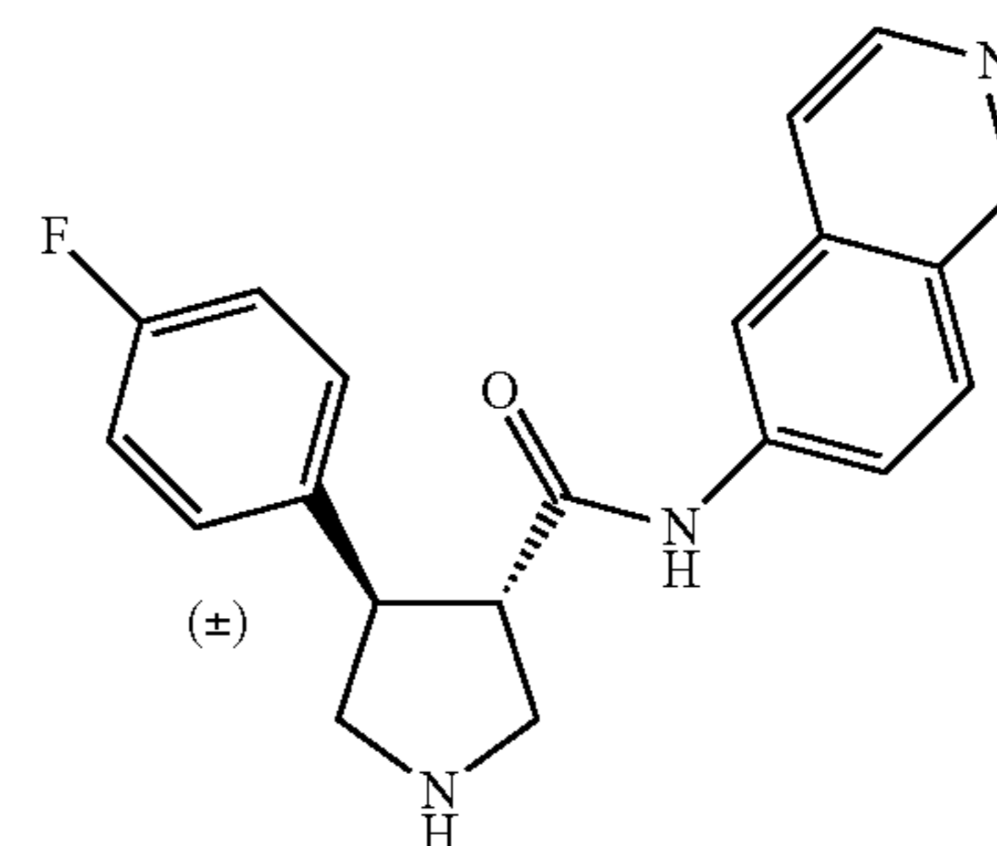
(trans)-4-(4-fluorophenyl)-N-(isoquinolin-6-yl)pyrrolidine-3-carboxamide
