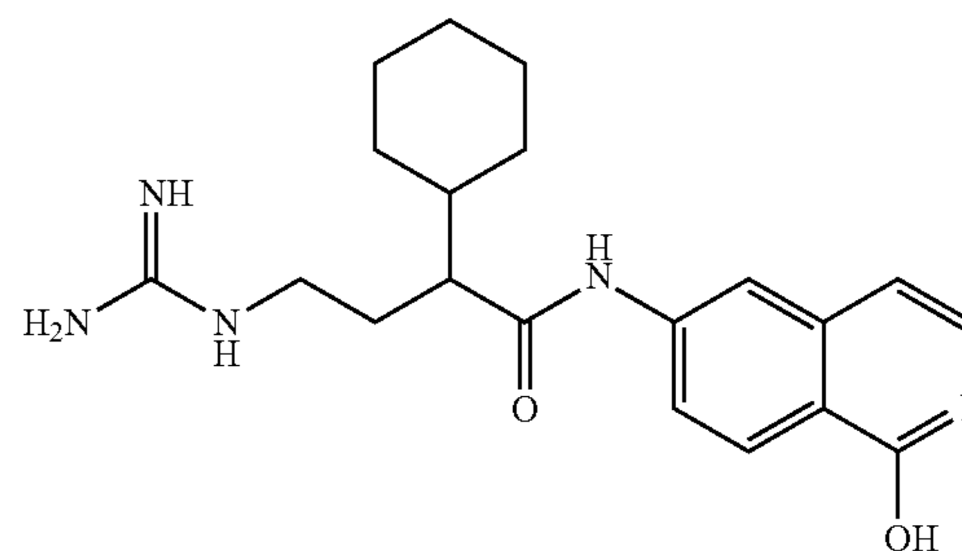
2-cyclohexyl-4-guanidino-N-(1-hydroxyisoquinolin-6-yl)butanamide
