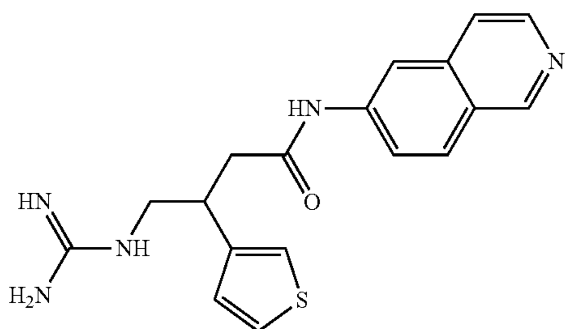
4-guanidino-N-(isoquinolin-6-yl)-3-(thiophen-3-yl)butanamide
