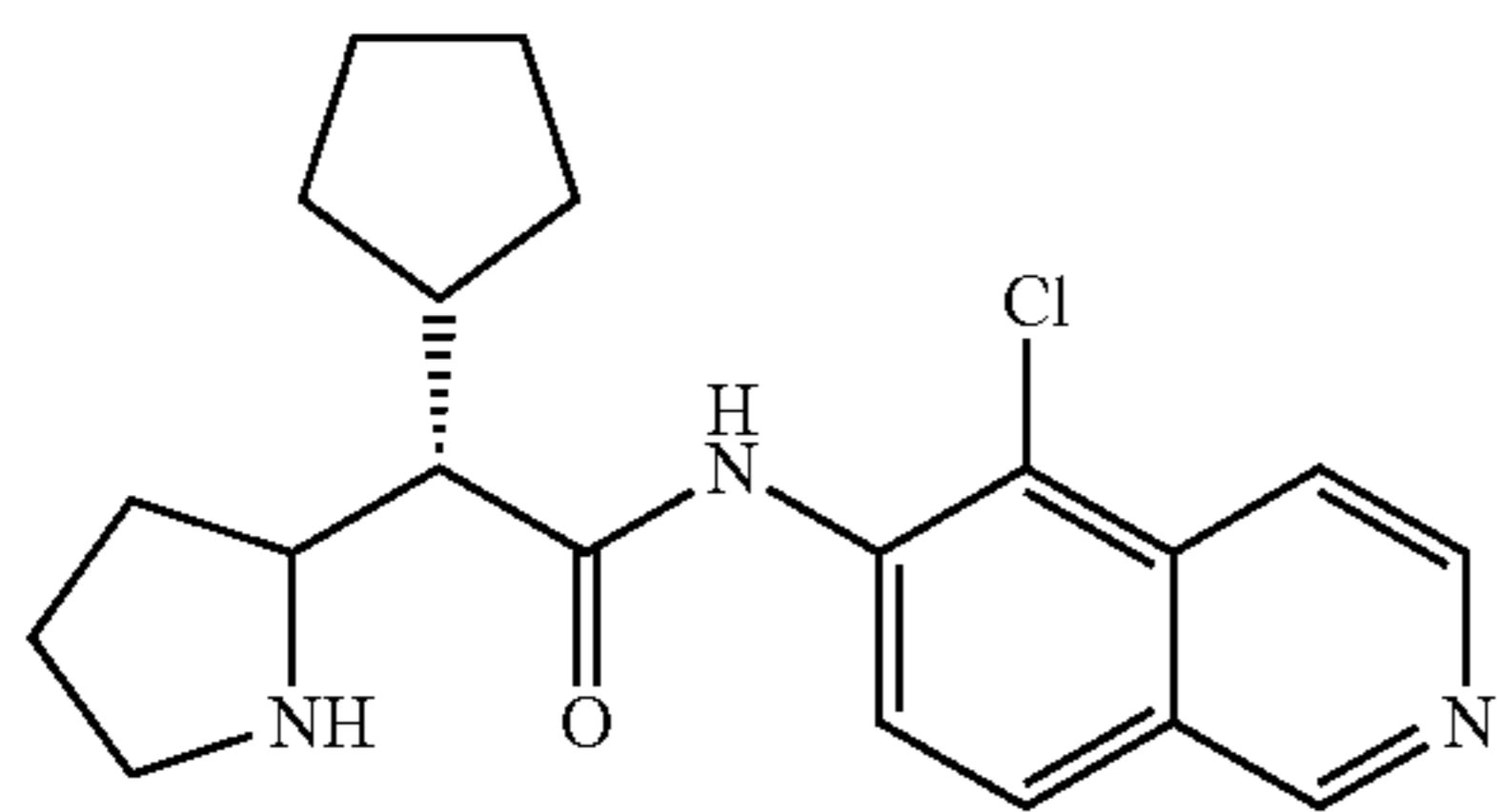
(2S)-N-(5-chloroisoquinolin-6-yl)-2-cyclopentyl-2-(pyrrolidin-2-yl)acetamide
