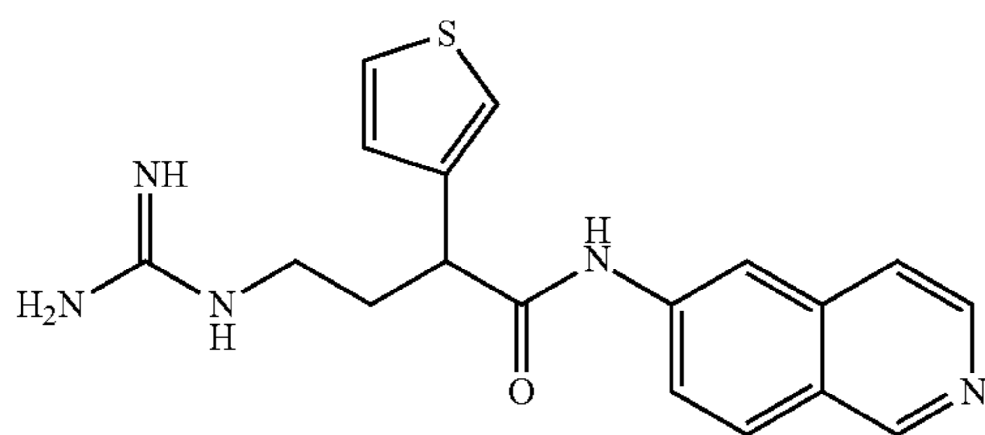
4-guanidino-N-(isoquinolin-6-yl)-2-(thiophen-3-yl)butanamide
