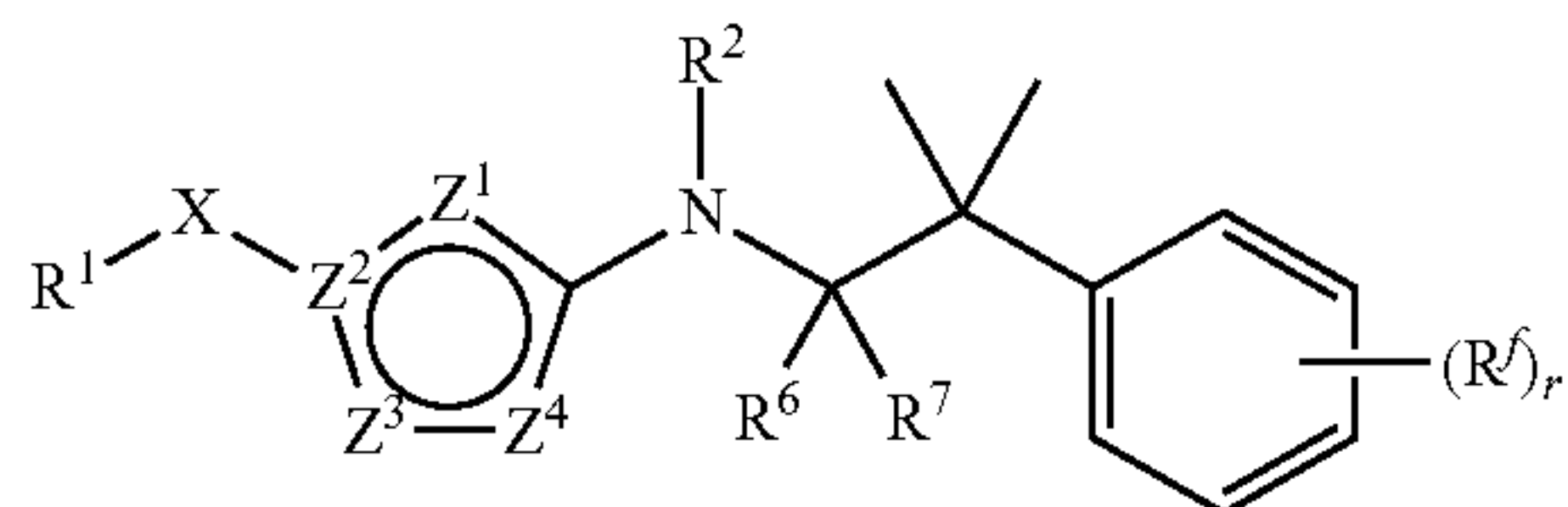
Formula VII(b)
