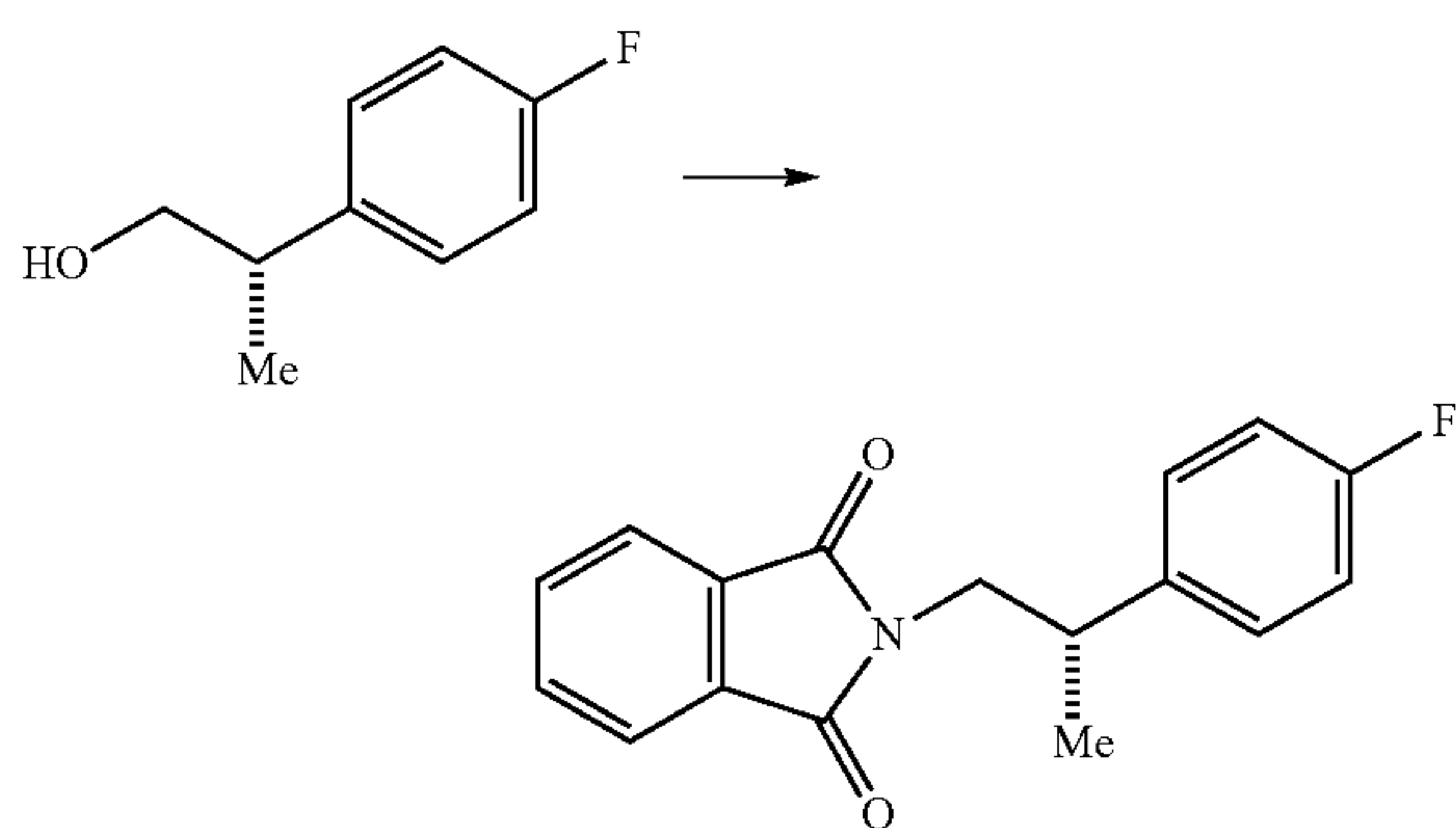
(S)-2-(2-(4-Fluorophenyl)propyl)isoindoline-1,3-dione
