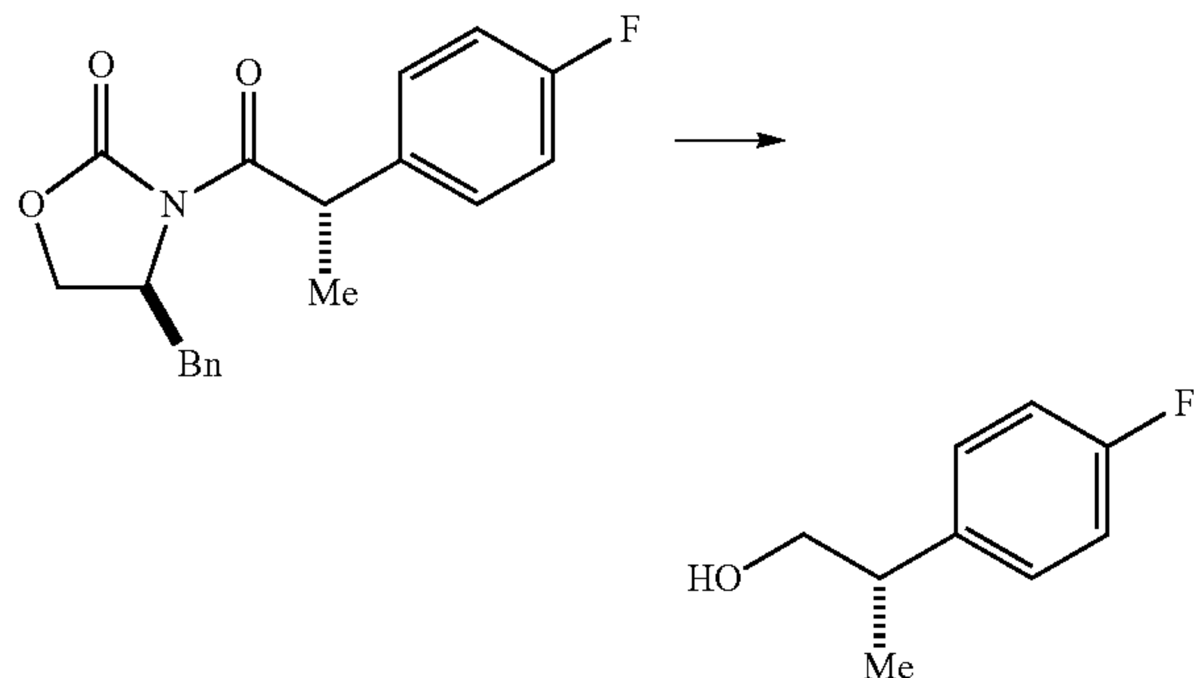
(S)-2-(4-Fluorophenyl)propan-1-ol
