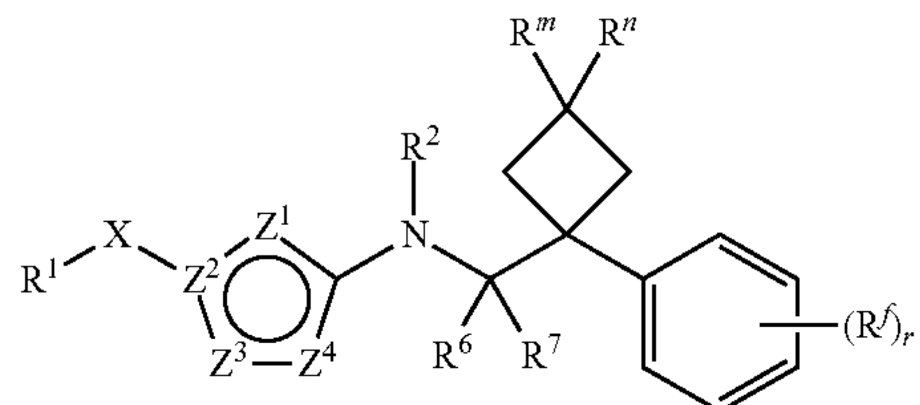
Formula VIII(b)
