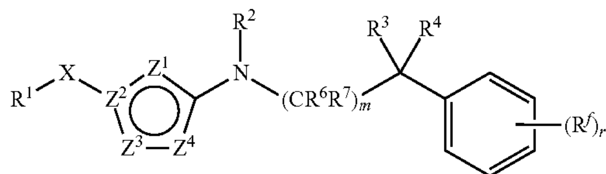
Formula VI
