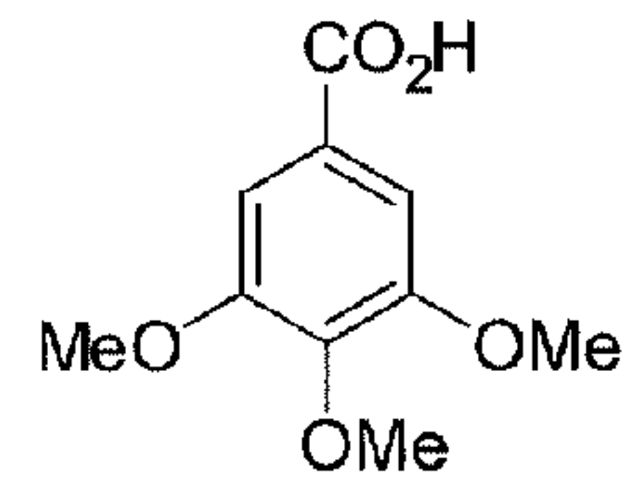
3,4,5-trimethoxybenzoic acid
