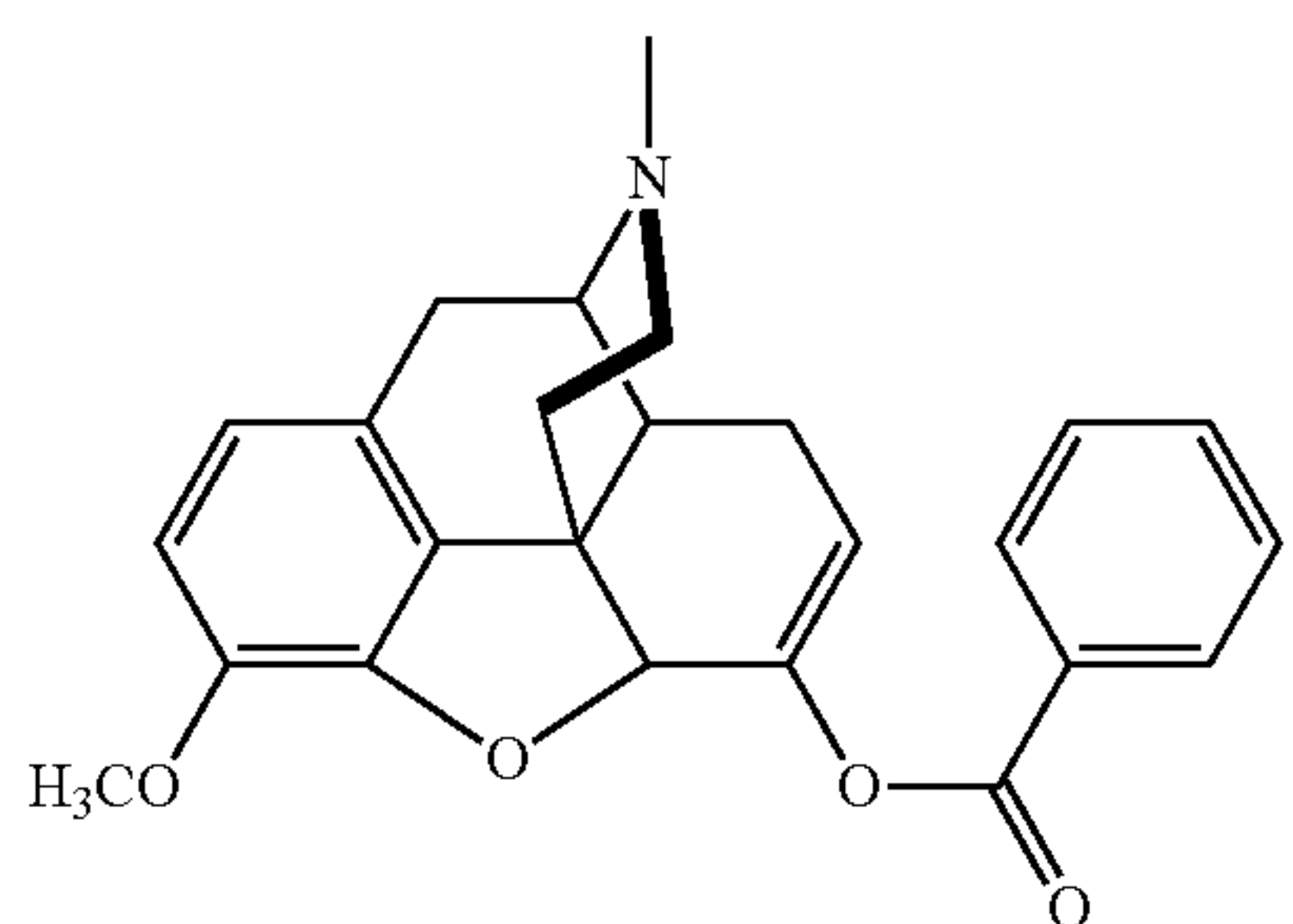
benzoate-hydrocodone (Bz-HC)
