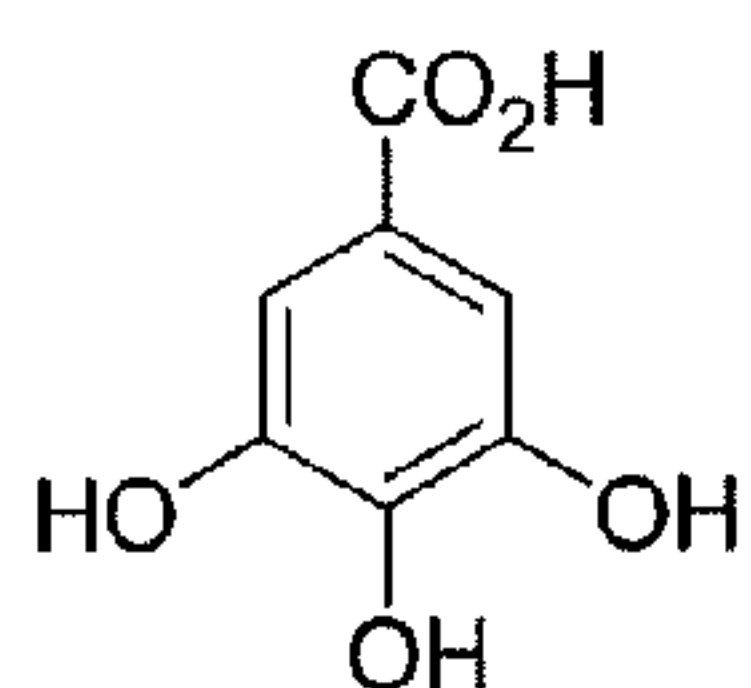
gallic acid
