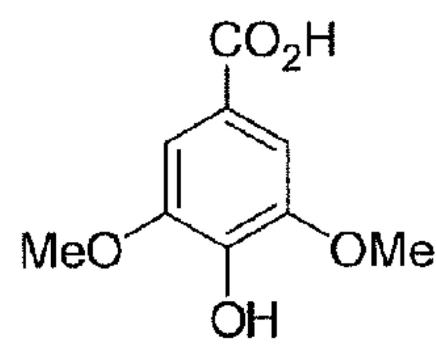
syringic acid
