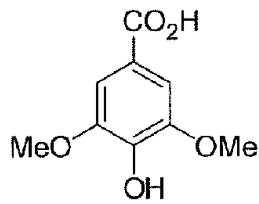
syringic acid
