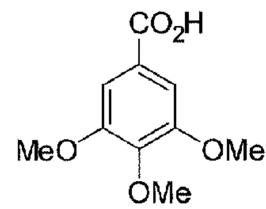
3,4,5-trimethoxy- benzoic acid
