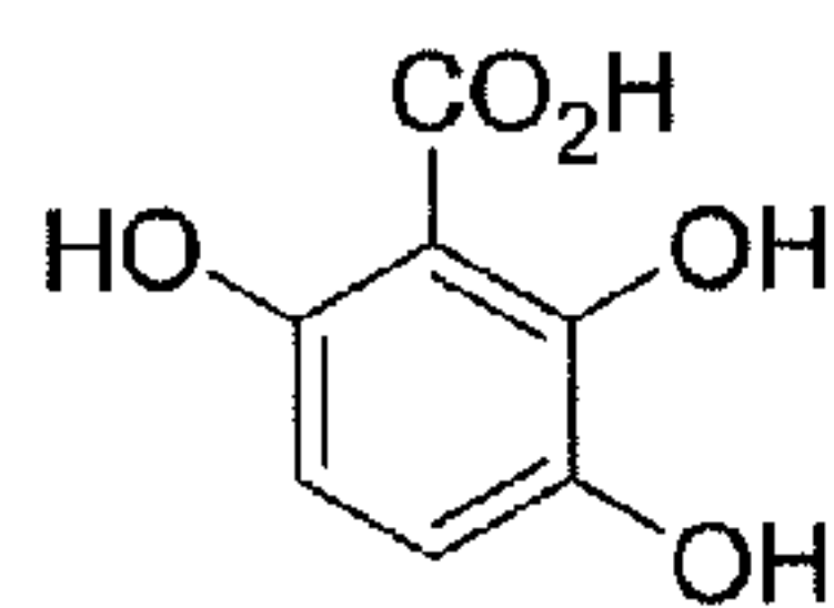
2,3,6-trihydroxybenzoic acid
