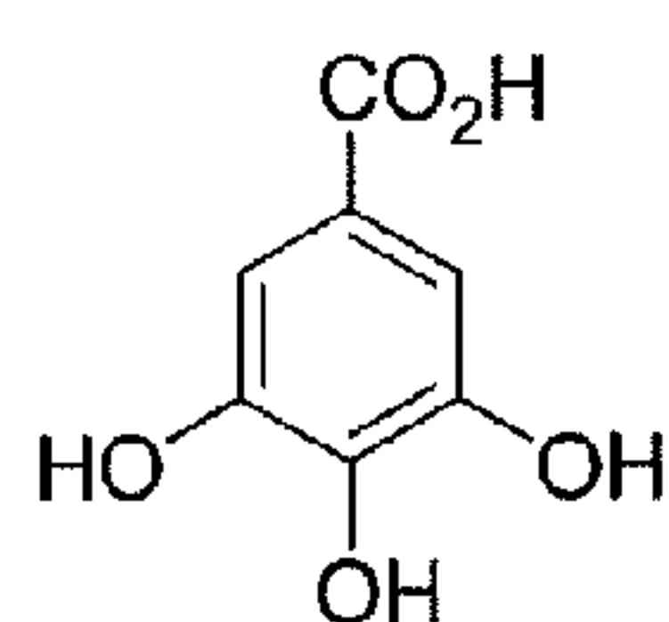
gallic acid
