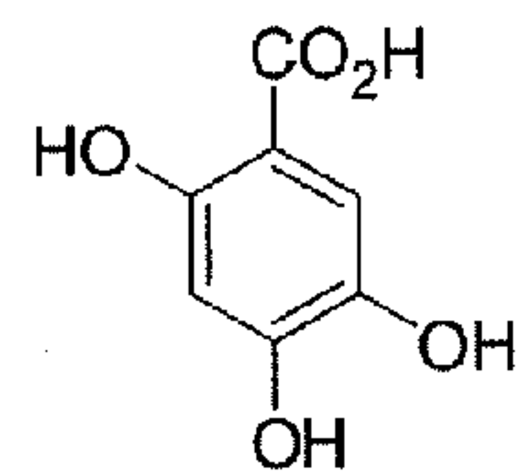
2,4,5-trihydroxybenzoic acid
