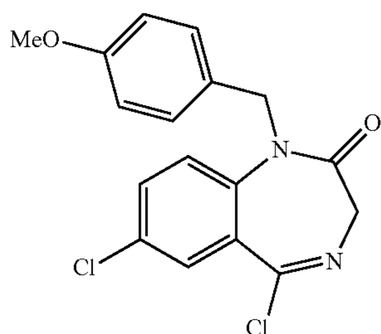
(E)-5,7-Dichloro-1-(4-methoxybenzyl)-1H-benzo[e] [1,4]diazepin-2(3H)-one
