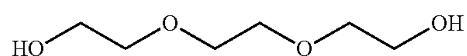
Triethylene glycol
