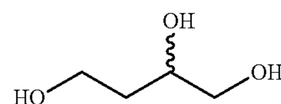
1,2,4-Butanetriol
