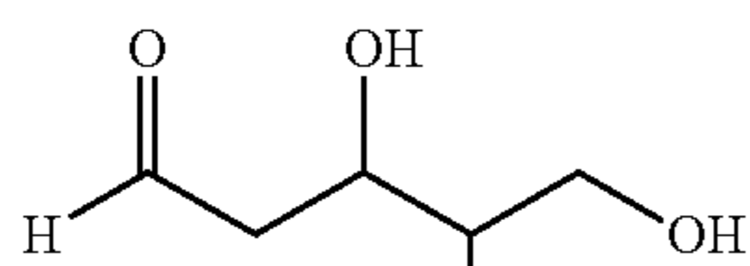
2-Deoxy-D-ribose
