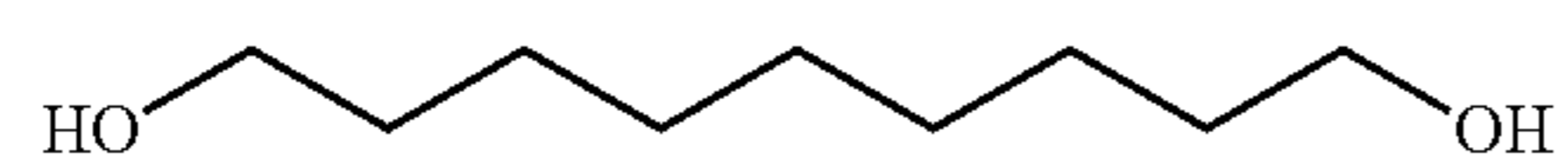
1,9-Nonanediol
