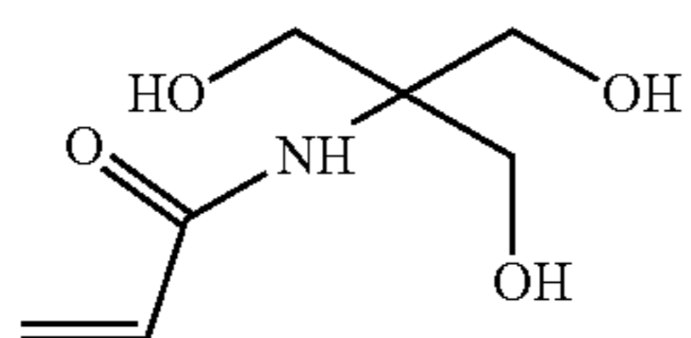
N-[Tris(hydroxymethyl) methyl]acrylamide
