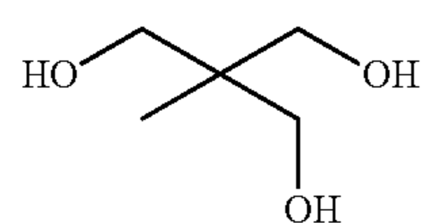
1,1,1-Tris(hydroxymethyl) ethane
