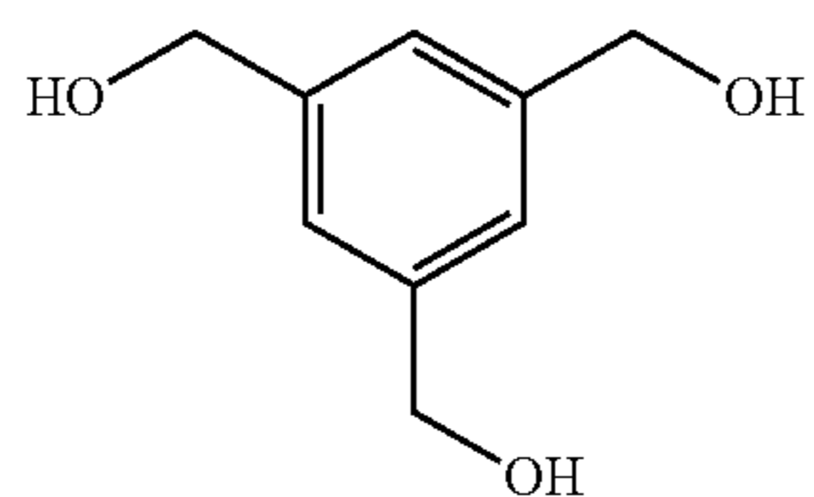
1,3,5-Tri(hydroxymethyl)benzene
