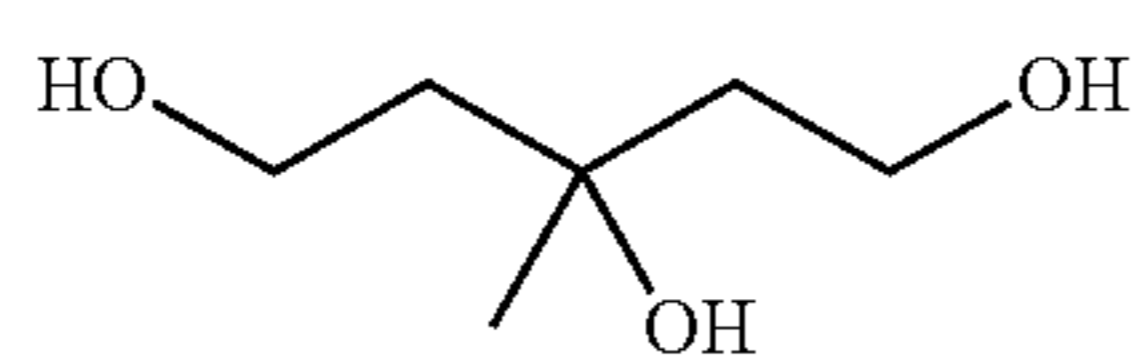
3-Methyl-1,3,5-pentanetriol
