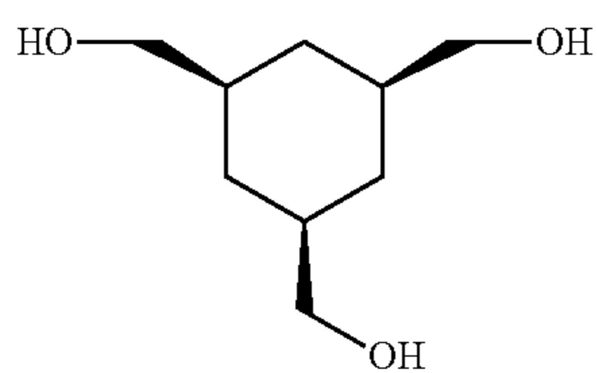
cis-1,3,5-Tri(hydroxymethyl) cyclohexane
