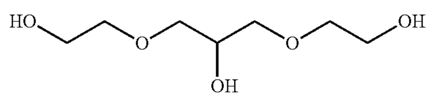
1,3-Di(hydroxyethoxy)-2-hydroxyl-propane
