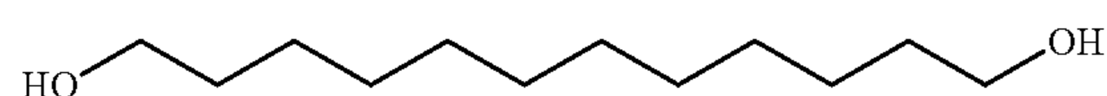
1,12-Dodecanediol
