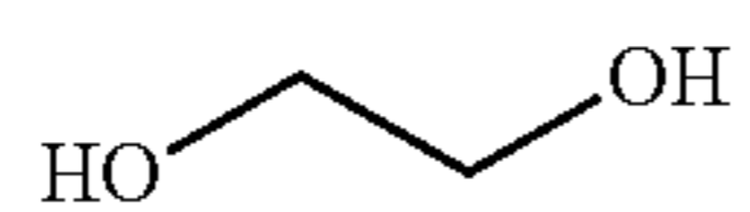
Ethylene glycol
