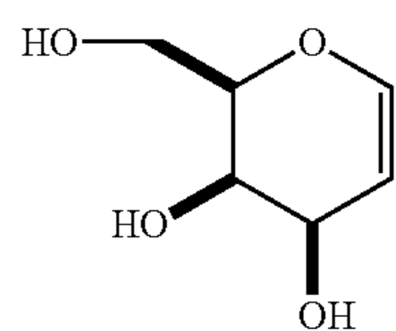
D-Galactal
