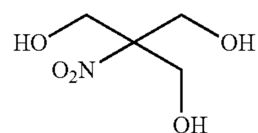
1,1,1-Tris(hydroxymethyl) nitromethane
