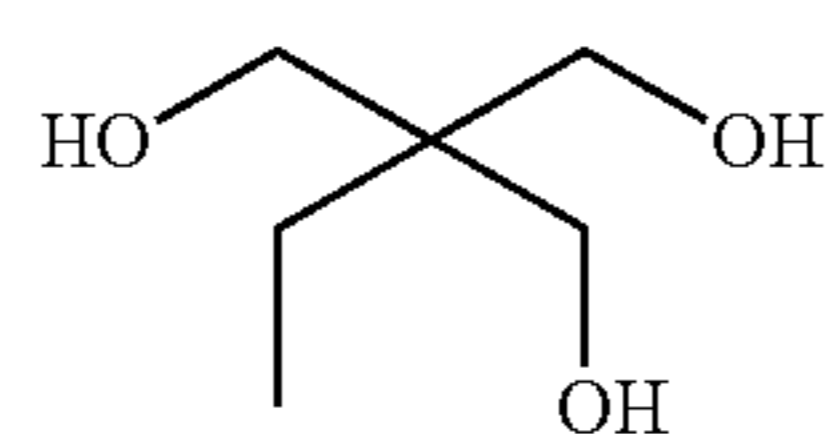
1,1,1-Tris(hydroxymethyl)propane
