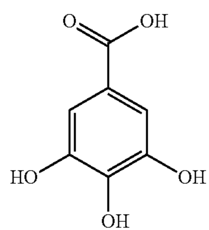
Gallic acid
