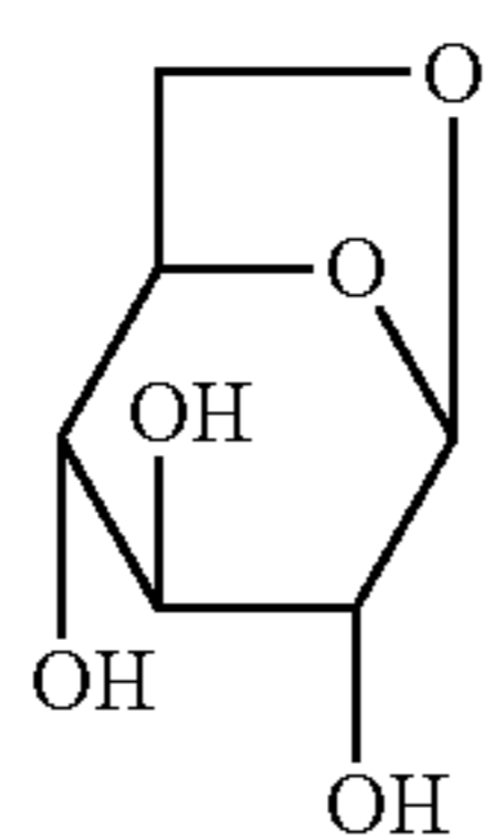
1,6-anhydro-β-D-Glucose
