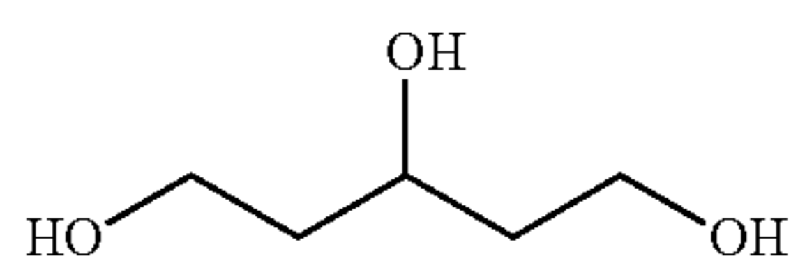
1,3,5-Pentanetriol
