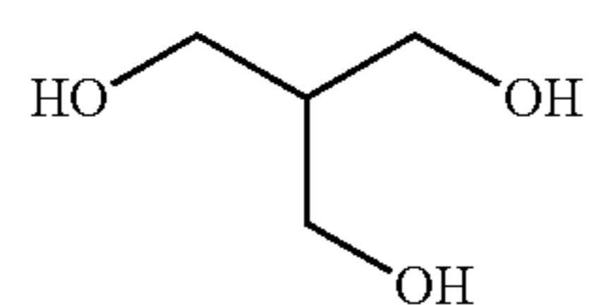
2-(hydroxymethyl)-1,3-propanediol
