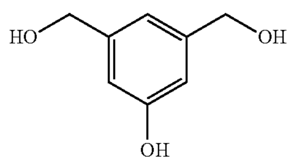
3,5-Di(hydroxymethyl)phenol
