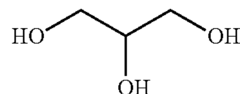
Glycerol (1,2,3-Propanetriol)
