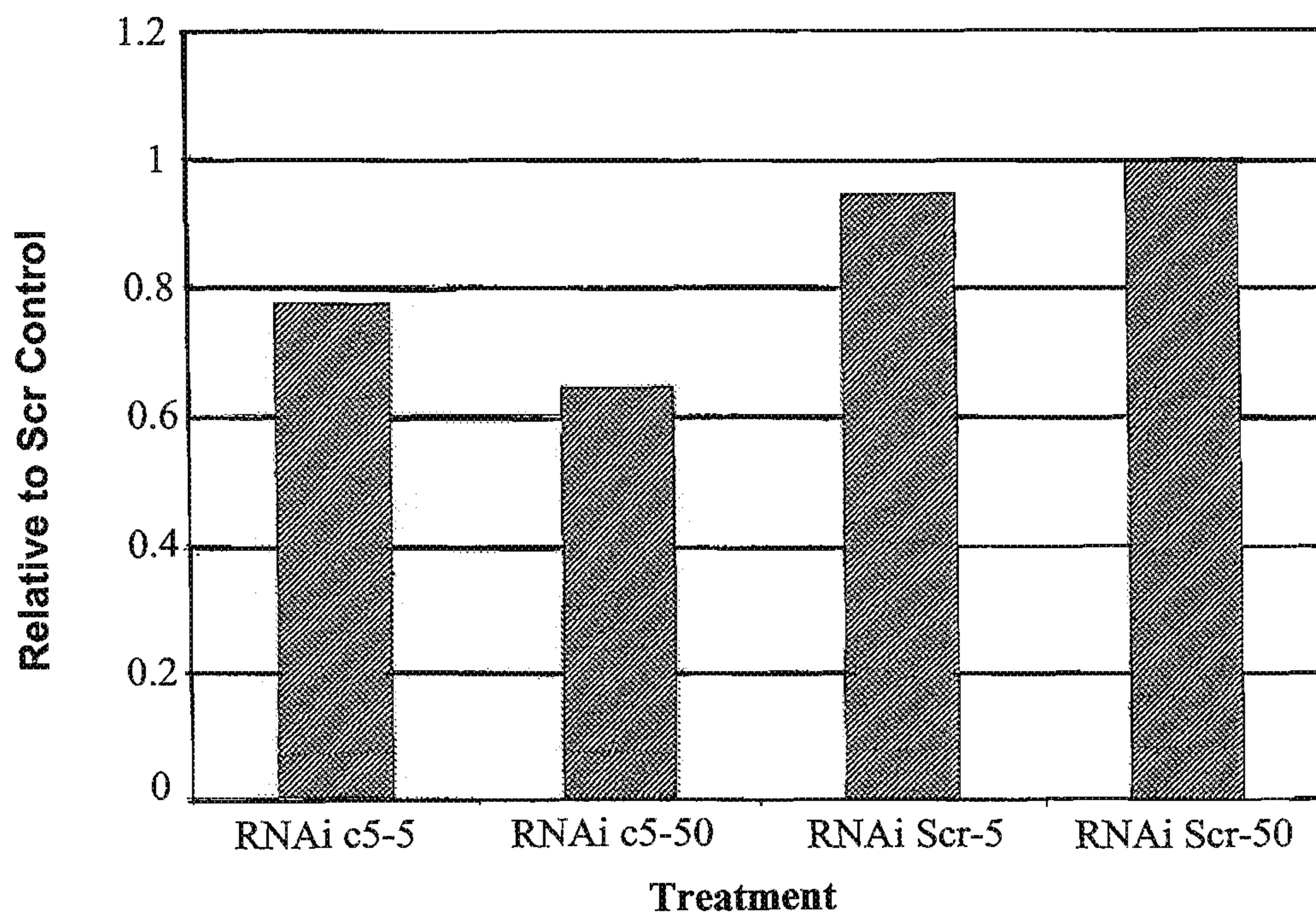
Clusterin Levels From Western
