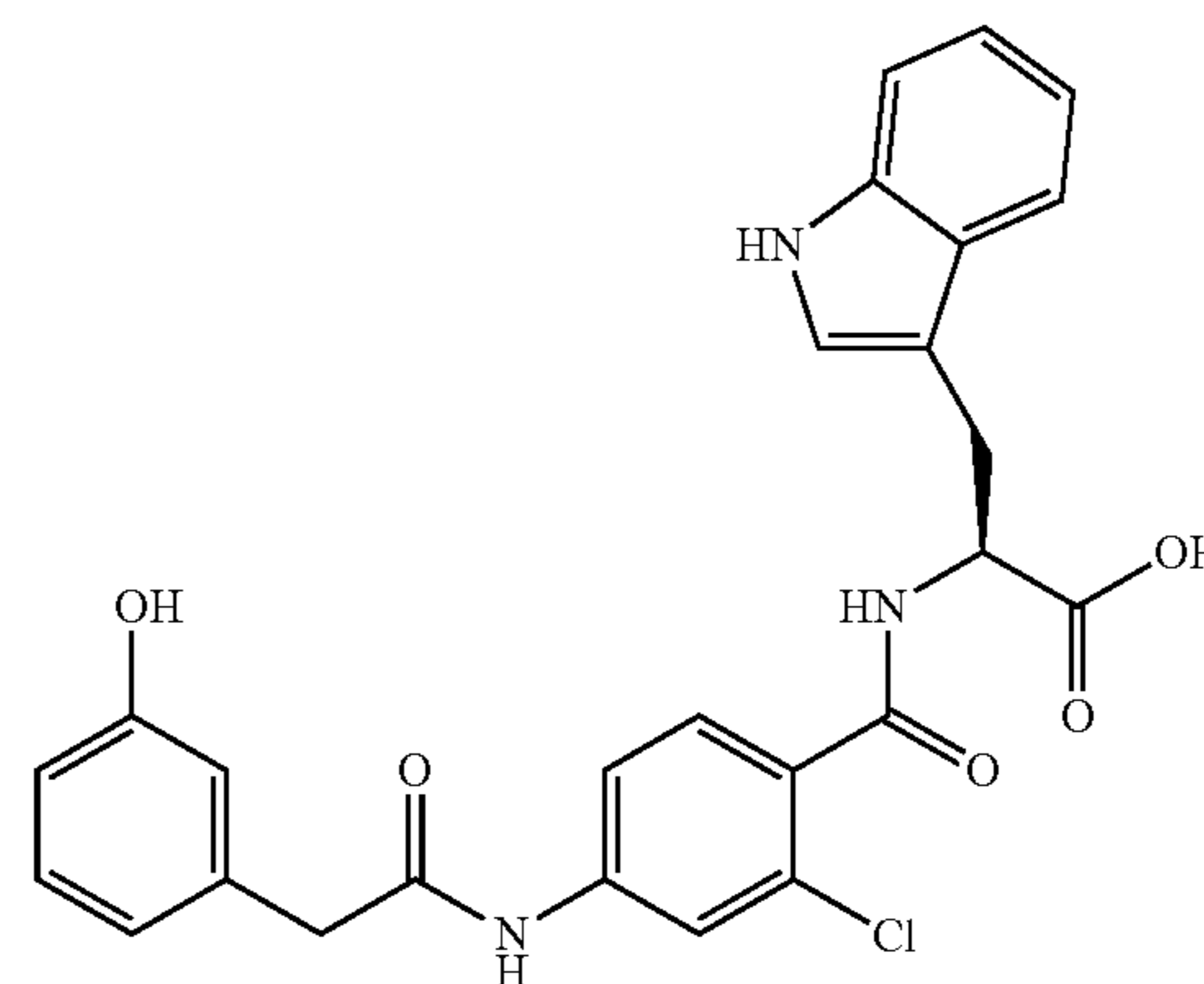
Compound 7
