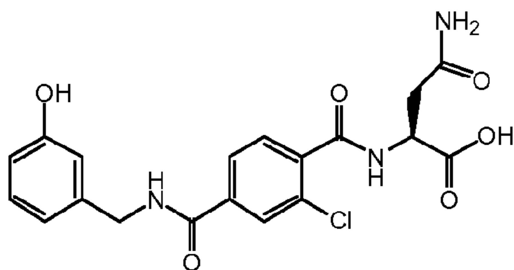
Compound 3
