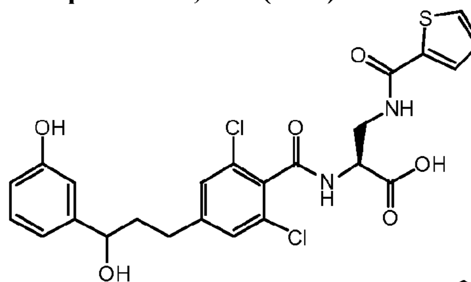
Compound 4
