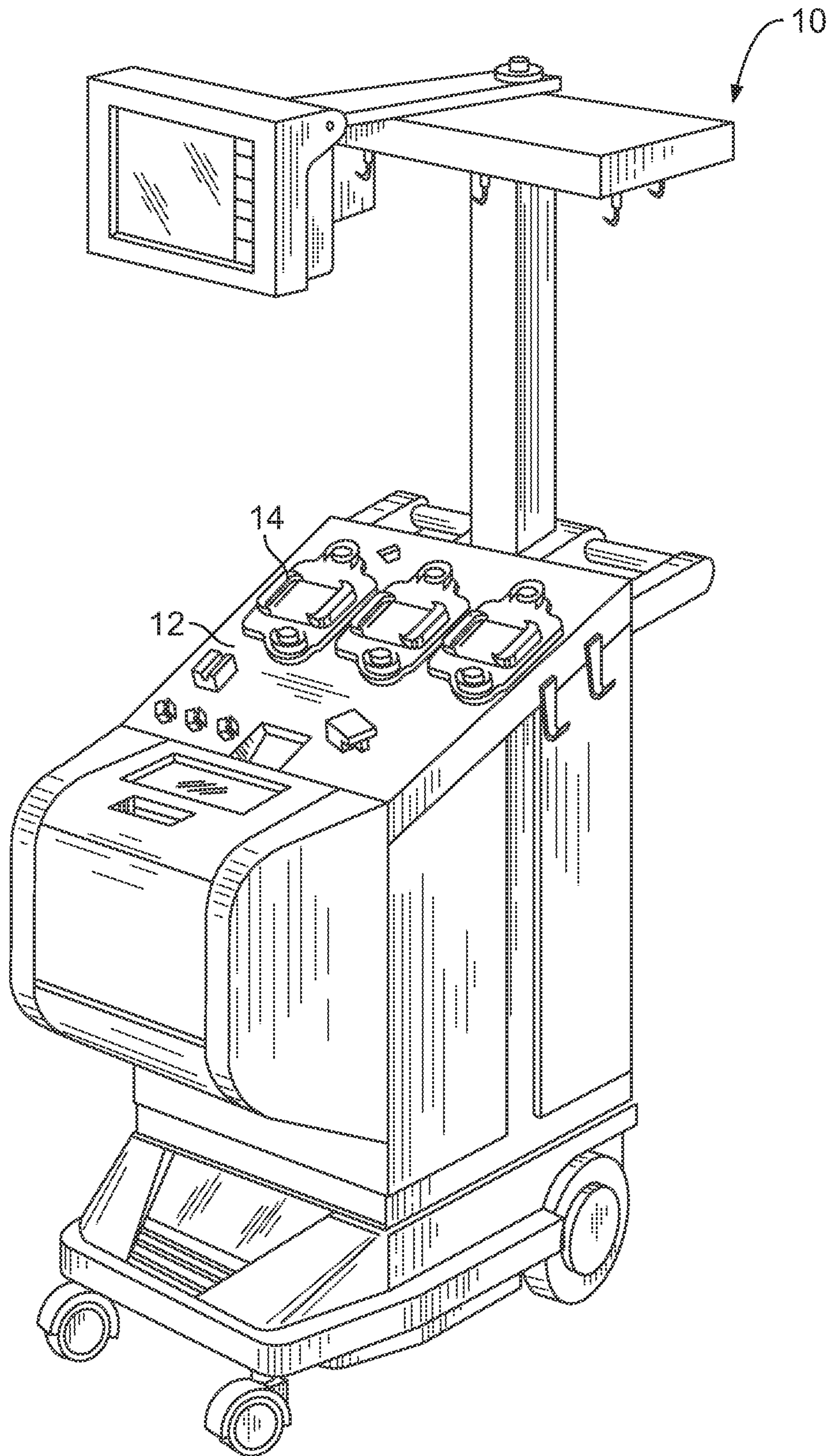
FIG. 1 (PRIOR ART)
