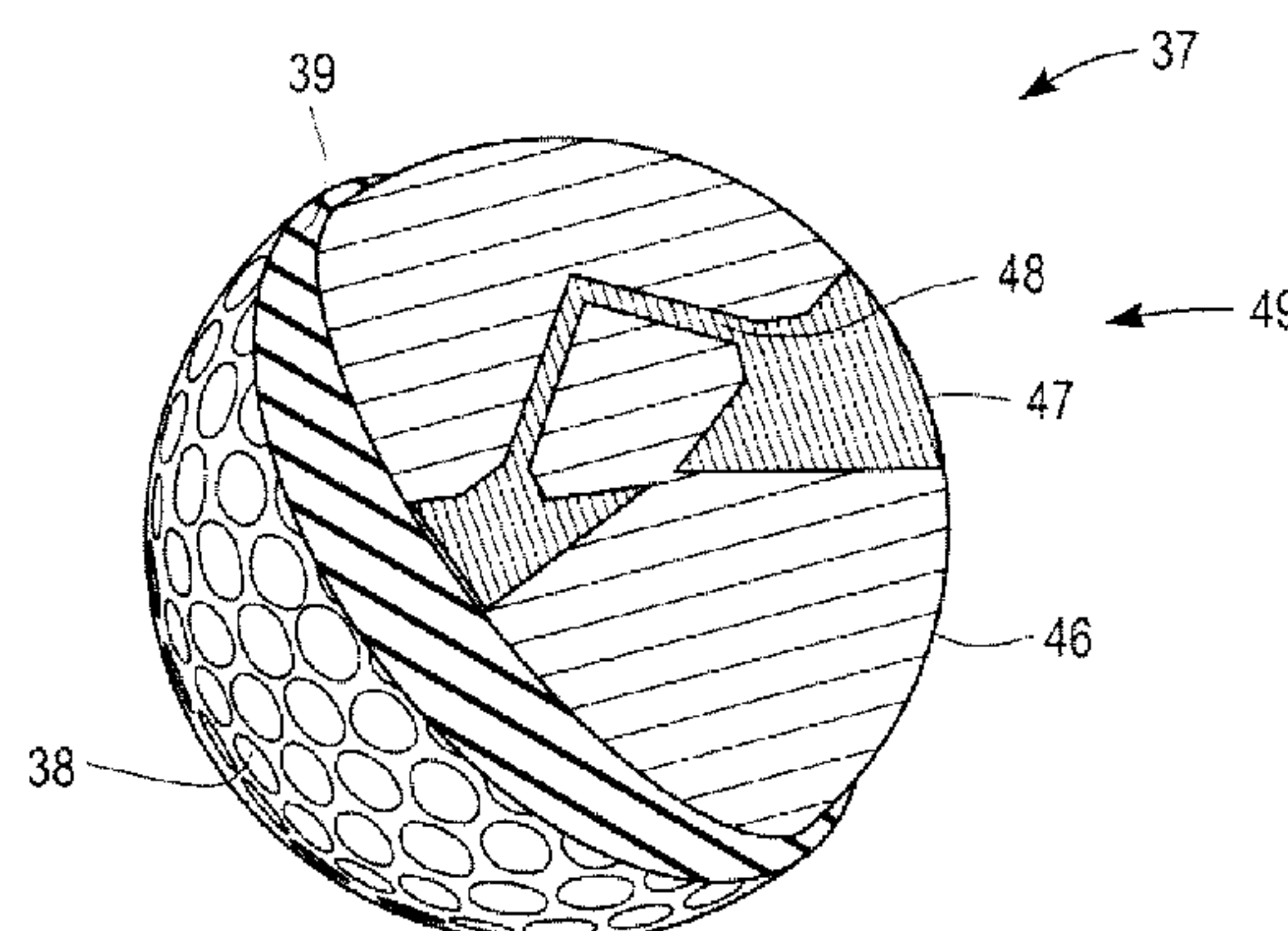
Antenna On Core (Not To Scale) Shown On A 3-piece Ball
