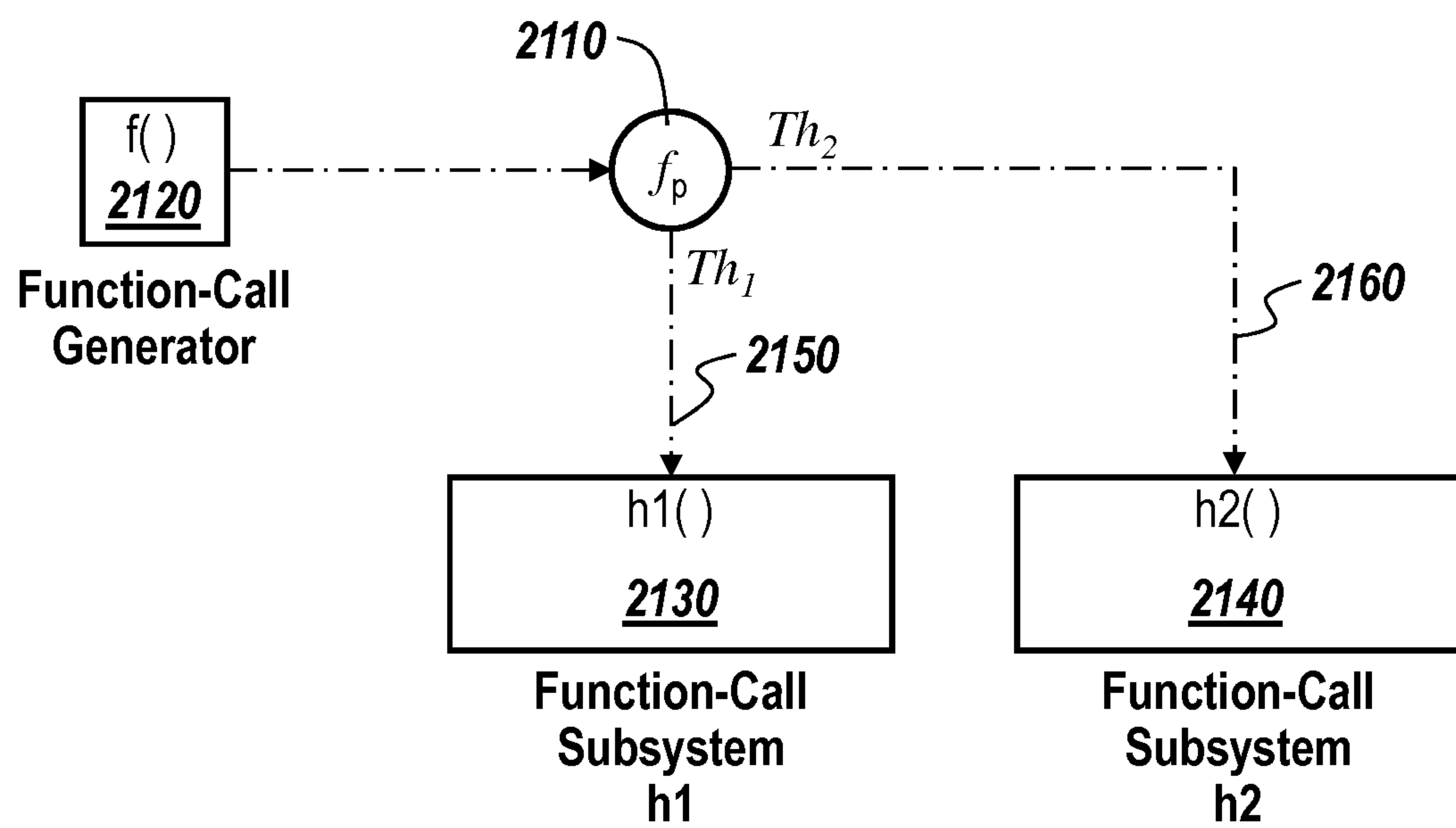
Fig fcn_call_parallel_h1_and_h2.mdl
