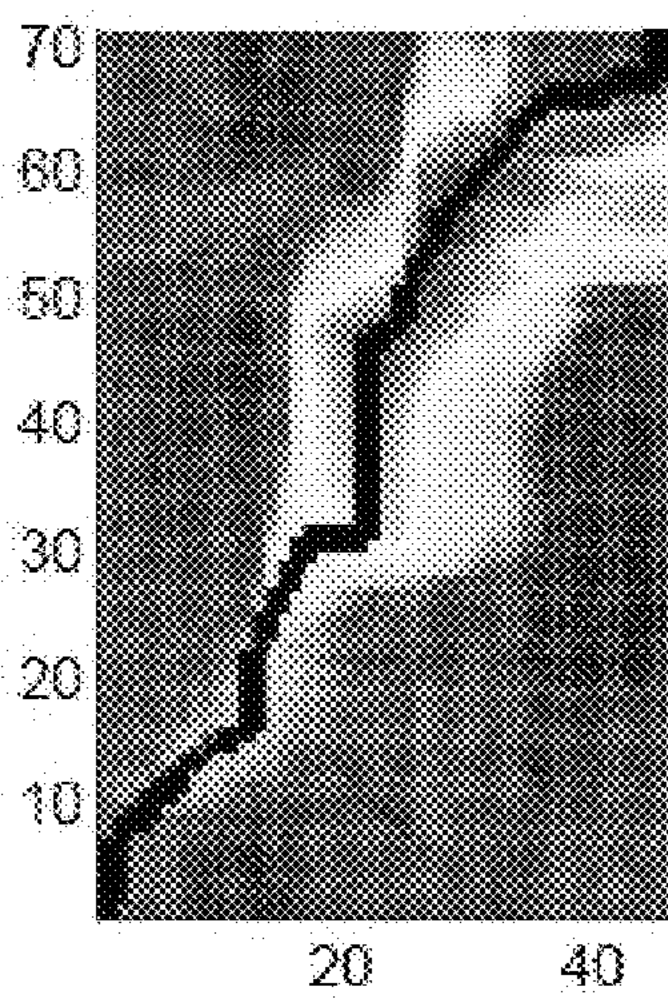
(c) \tau = 0.3
