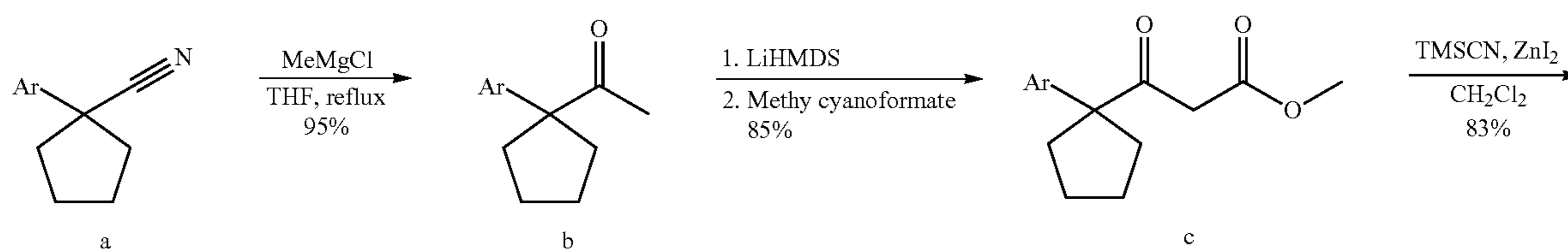
Scheme 7
