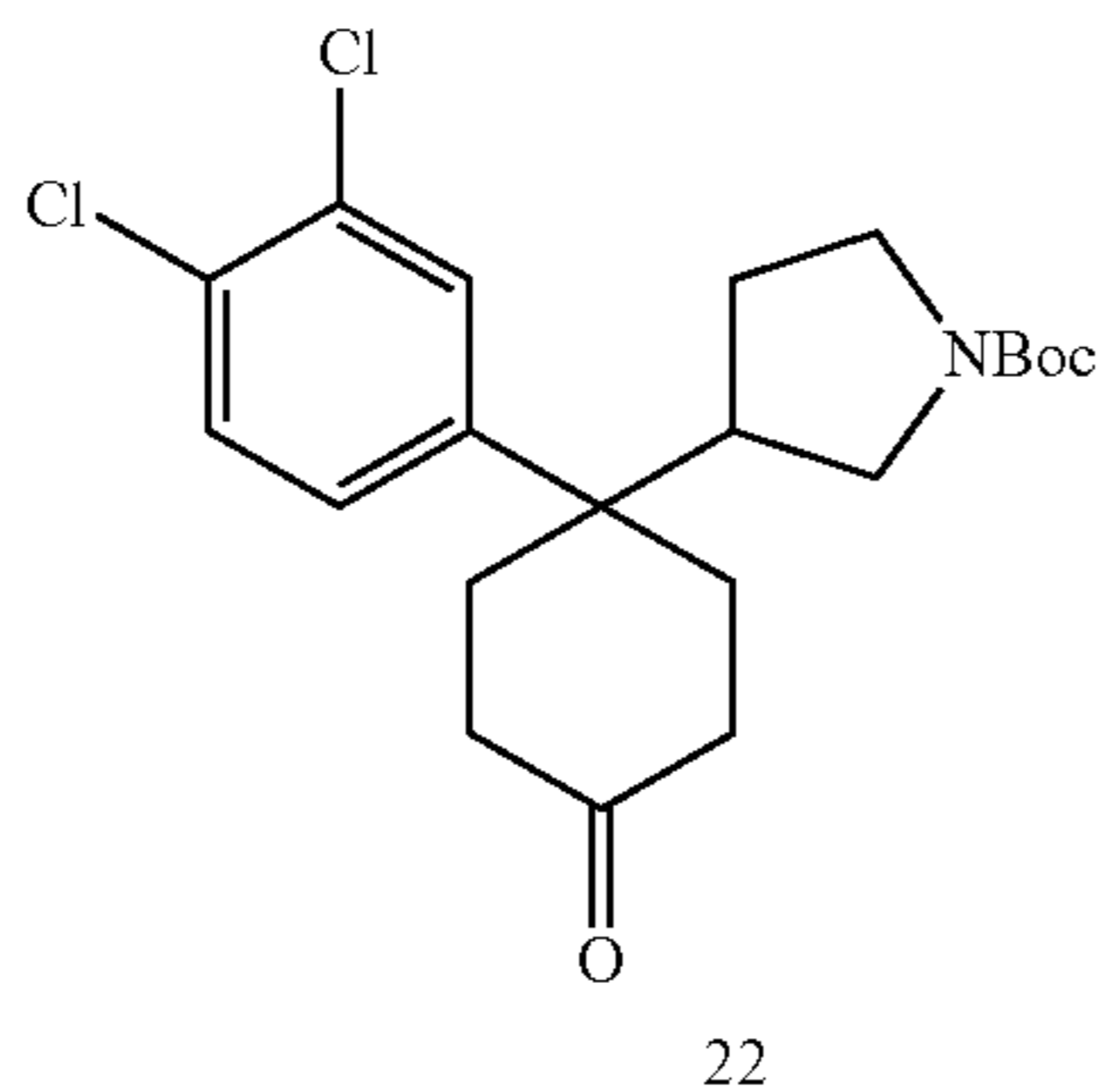
Scheme 4
