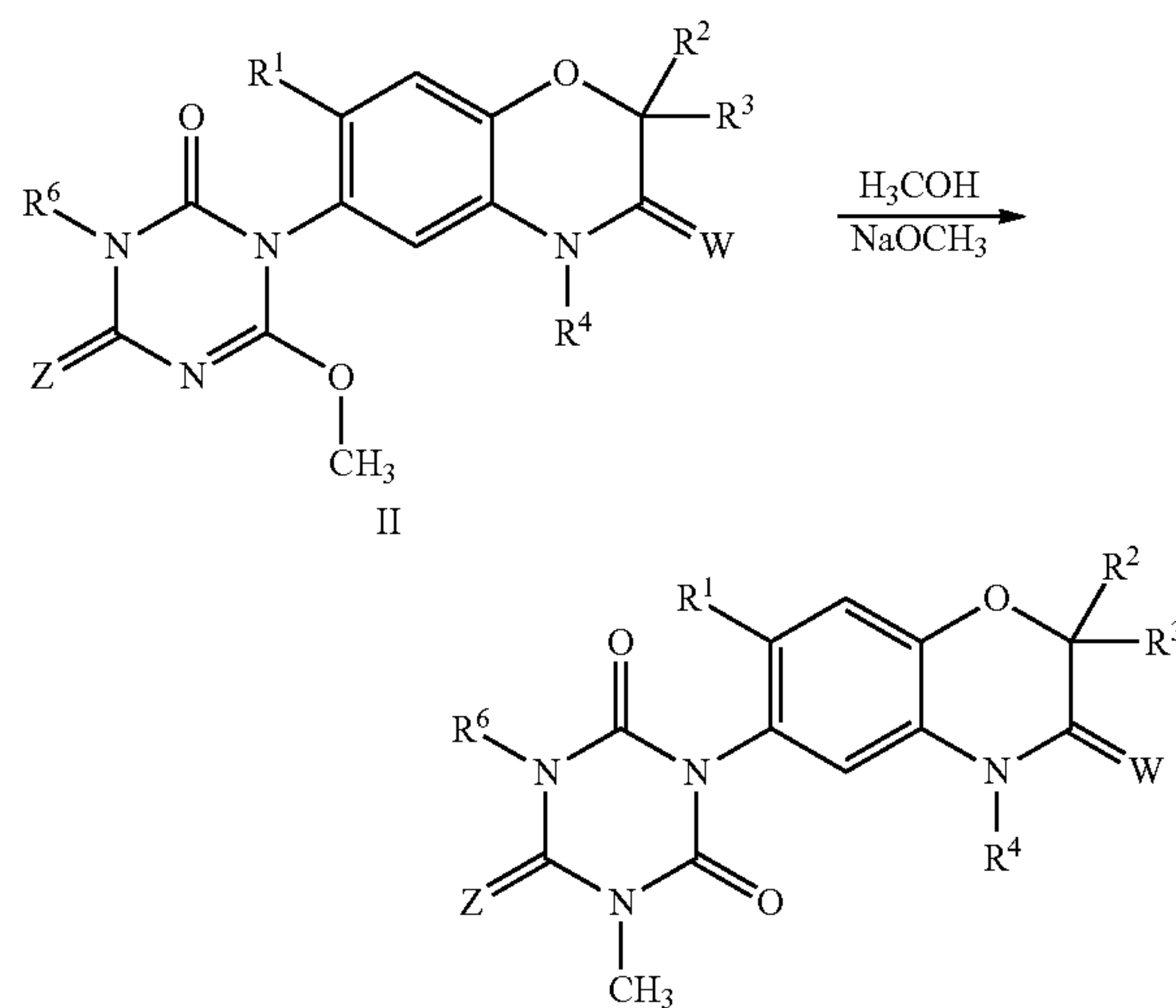
I wherein R 5 is CH 3
