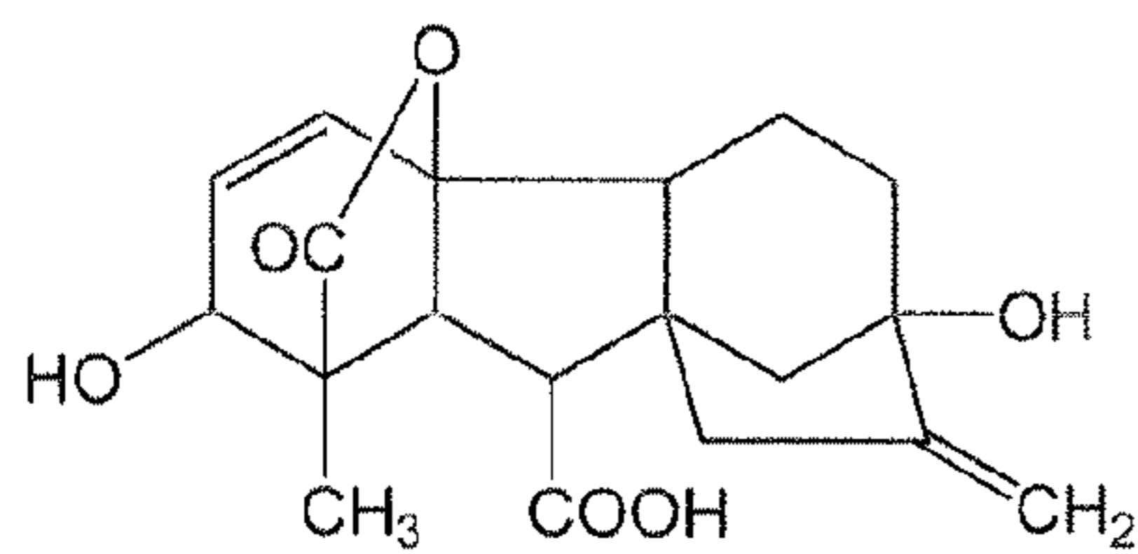
Gibberellic acid
