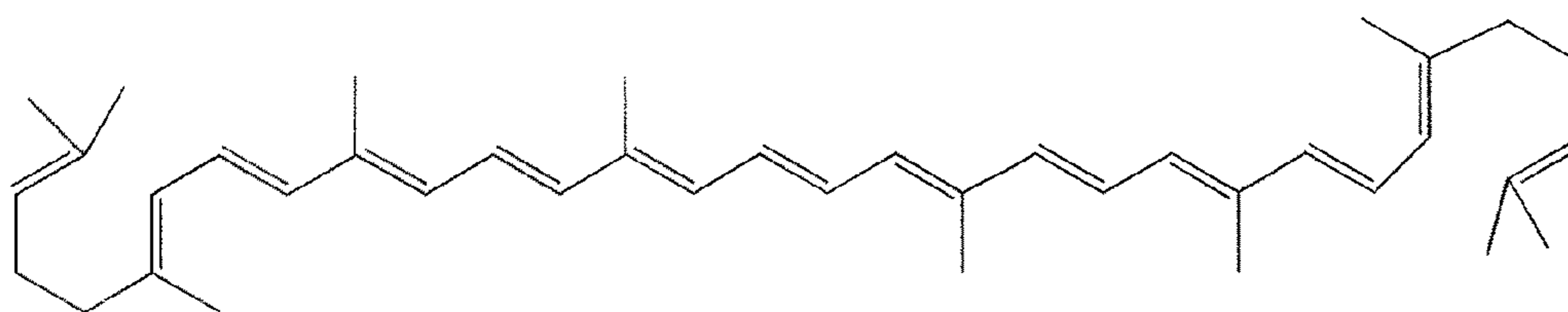
Lycopene
