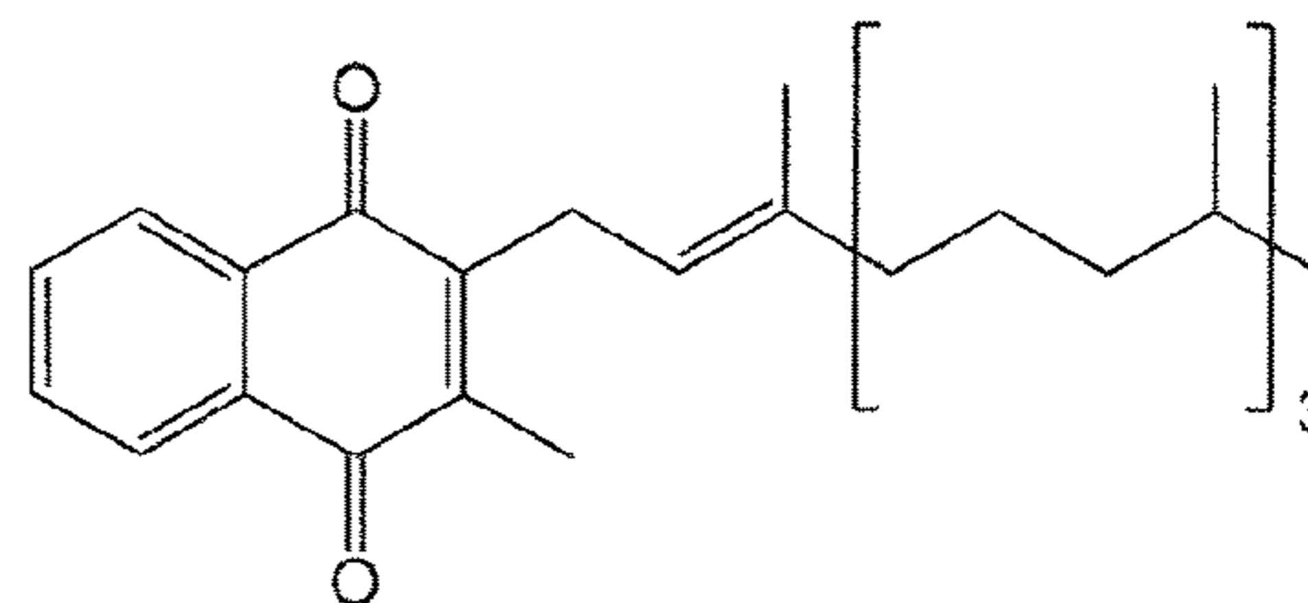
Phylloquinone
