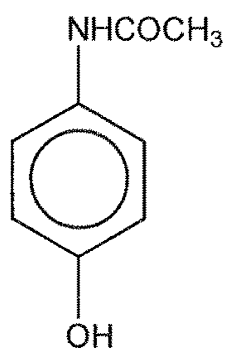
Acetaminophen
