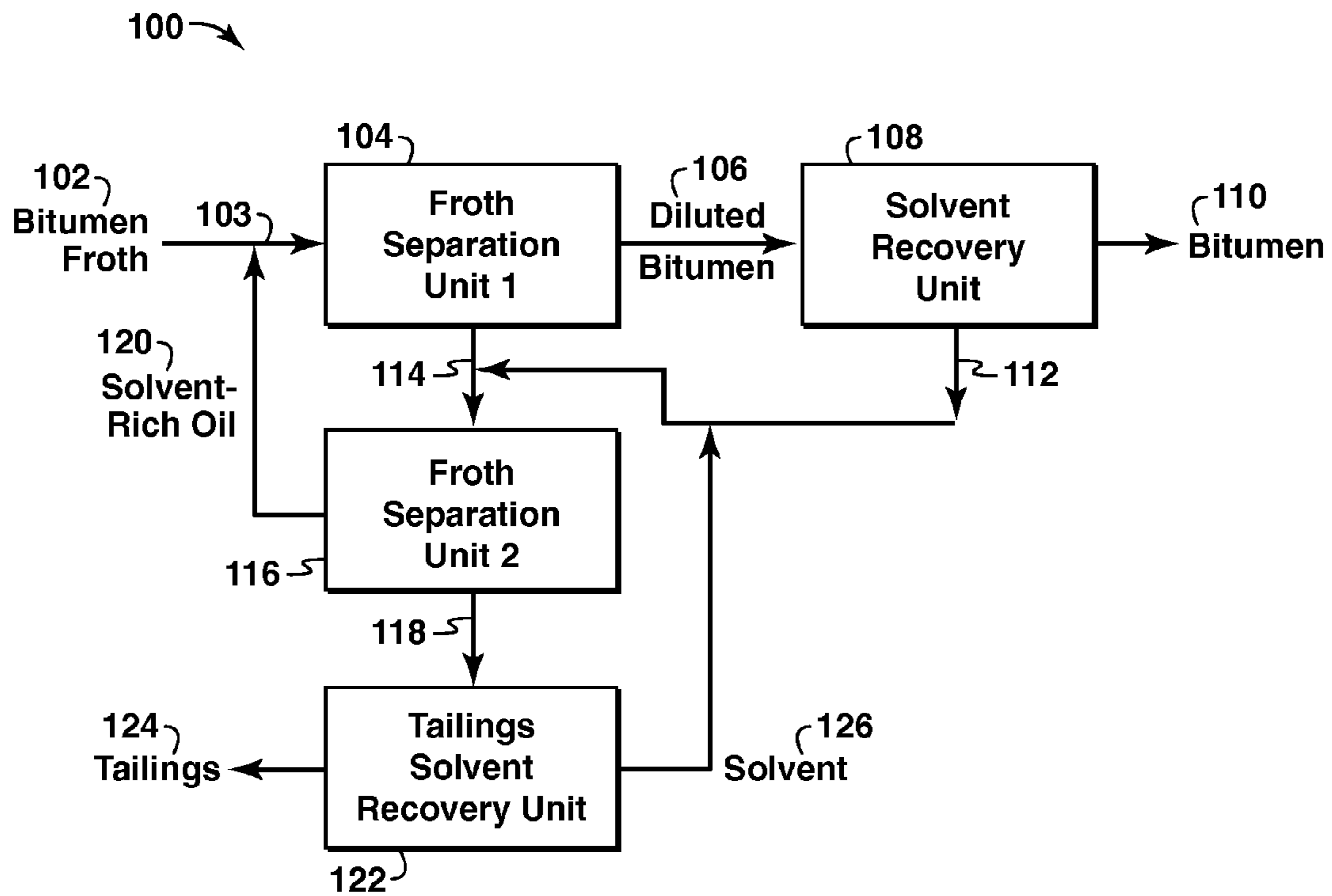
FIG. 1 Prior Art
