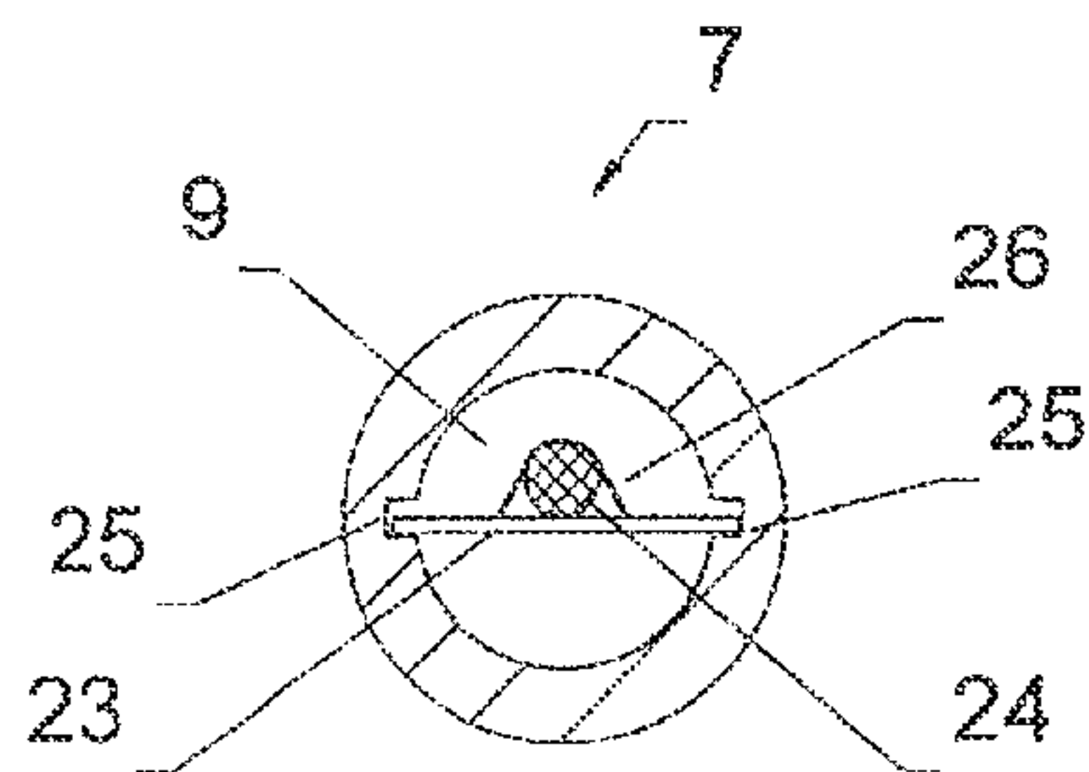
Section 3-3
