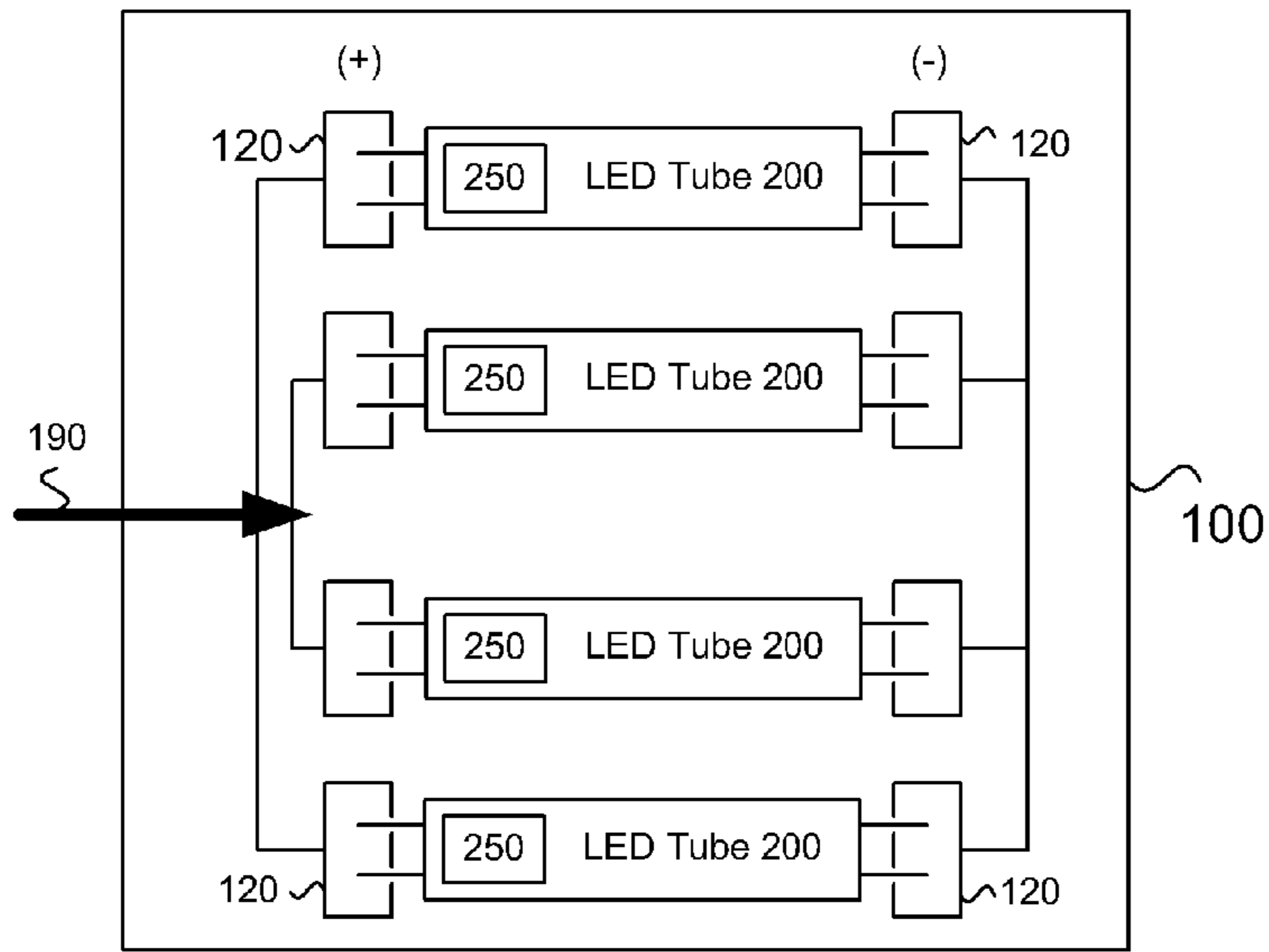
FIG. 3 (Prior Art)
