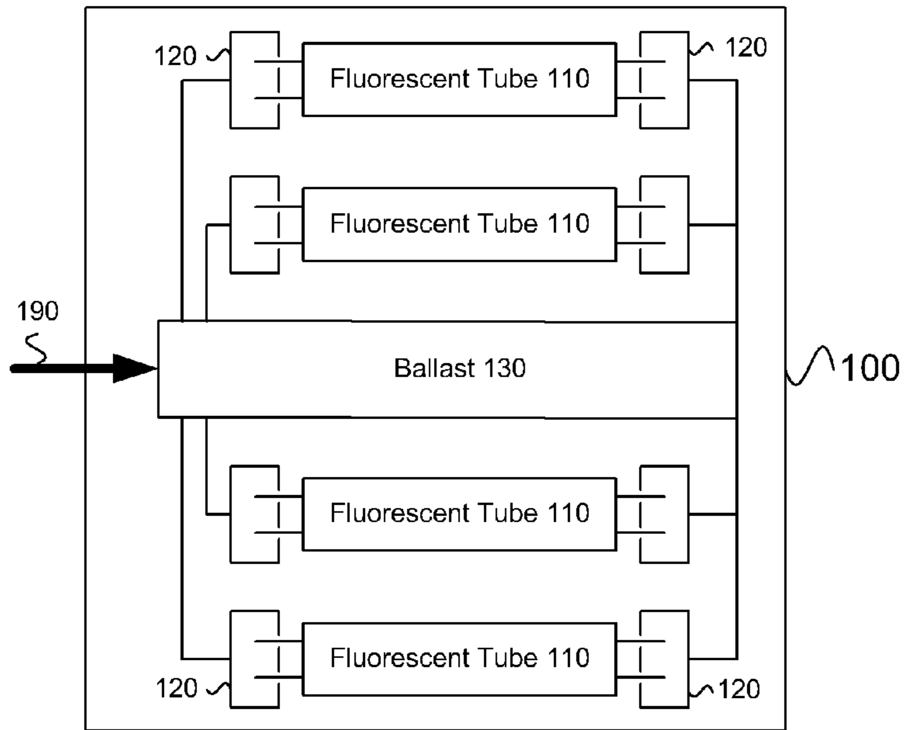
FIG. 1 (Prior Art)
