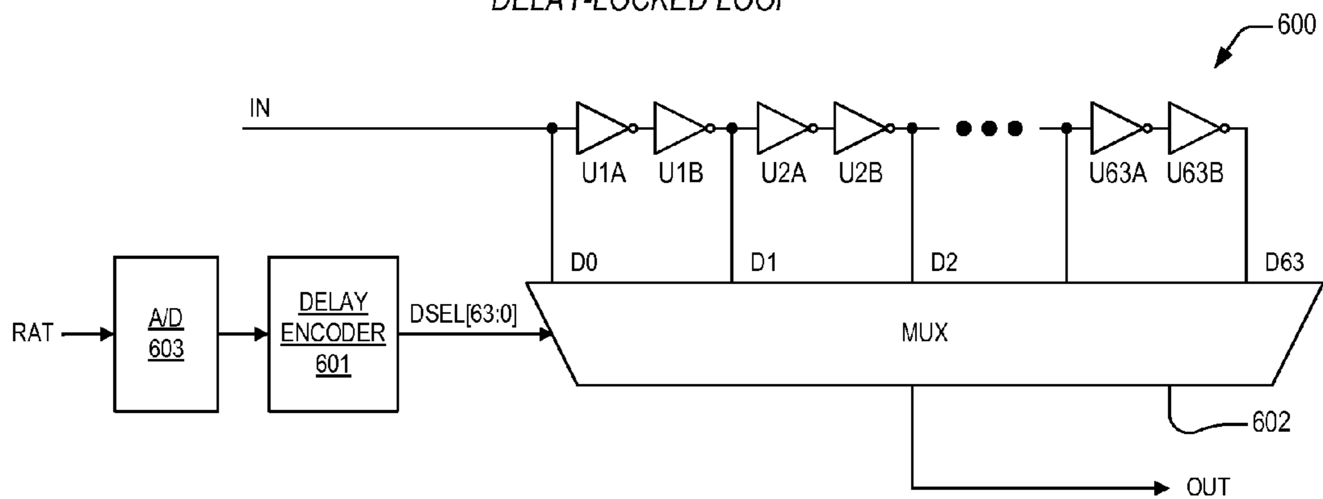
DELAY-LOCKED LOOP
