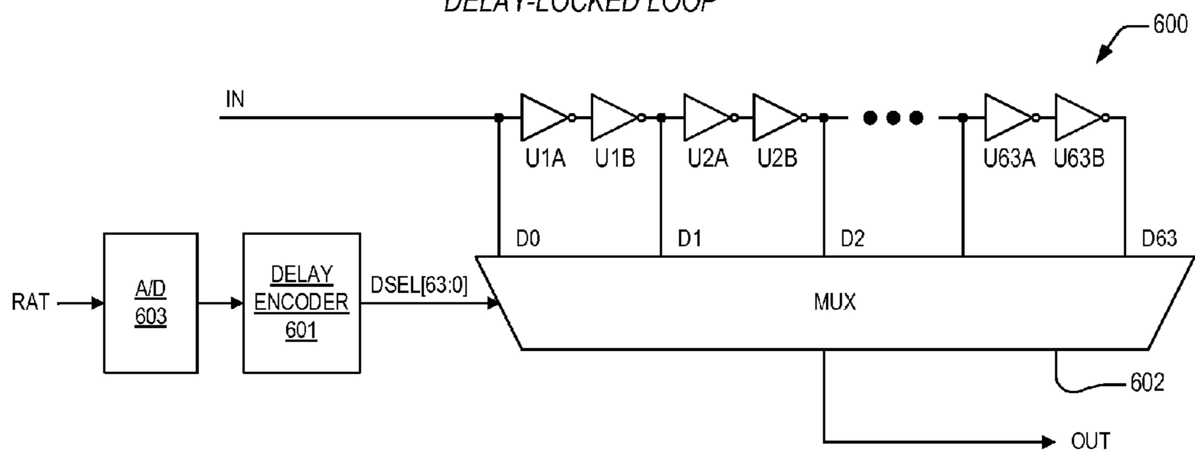
DELAY-LOCKED LOOP
