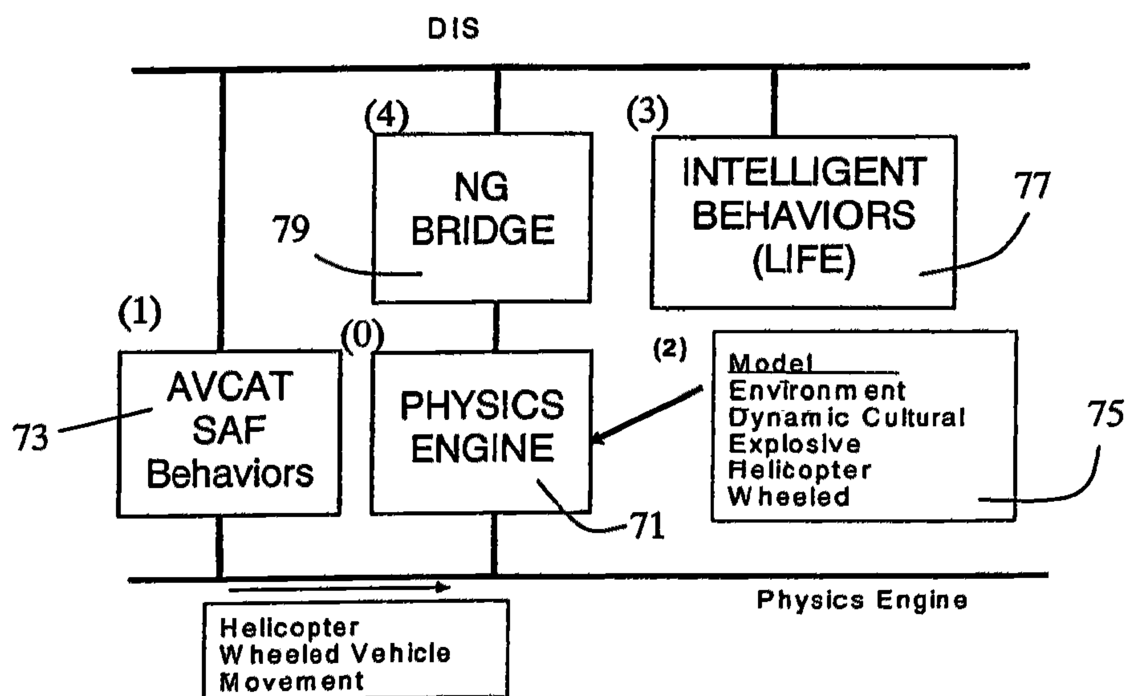
Physics Based Simulation Proof of Concept
