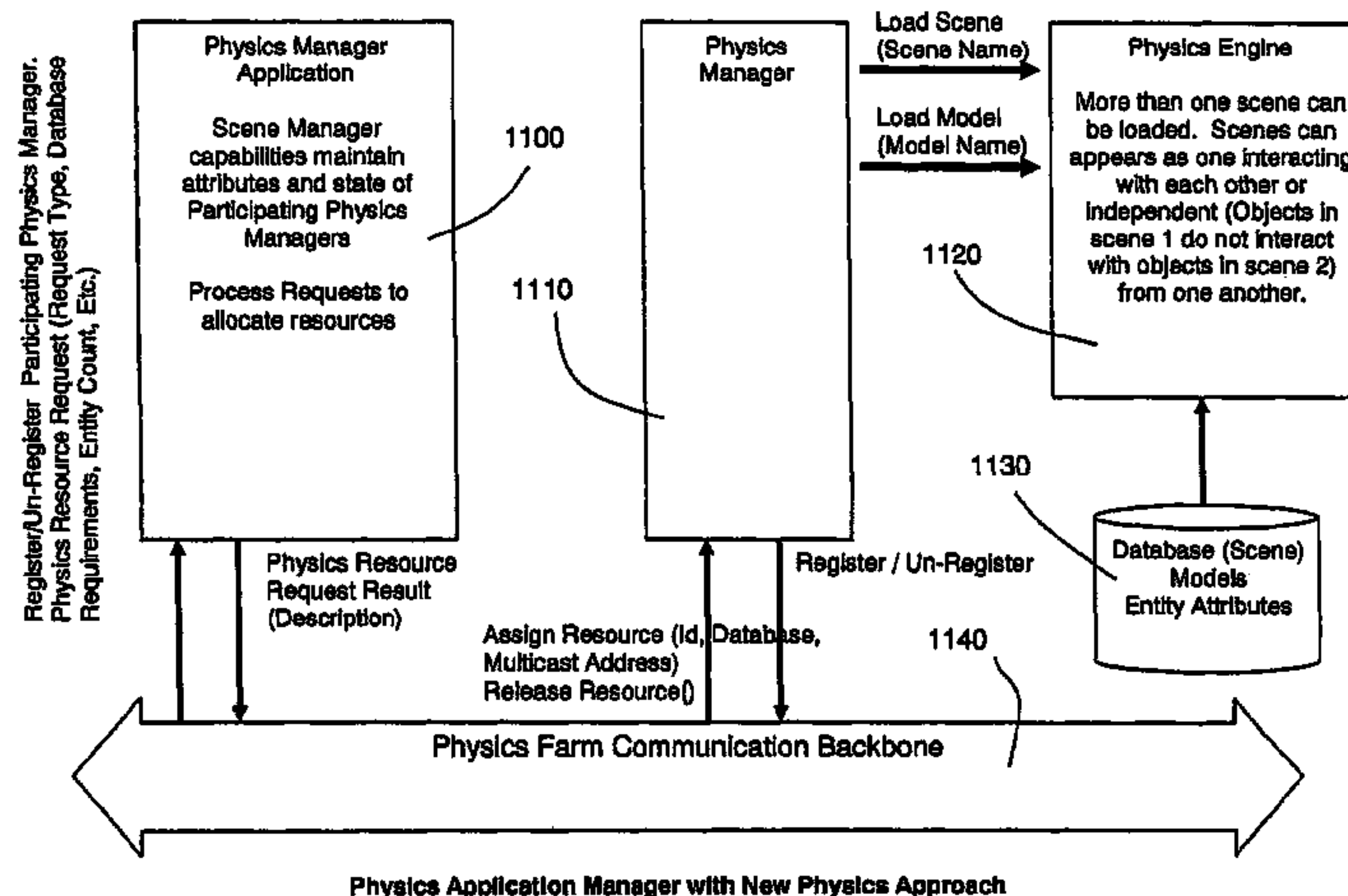
Physics Application Manager with New Physics Approach
