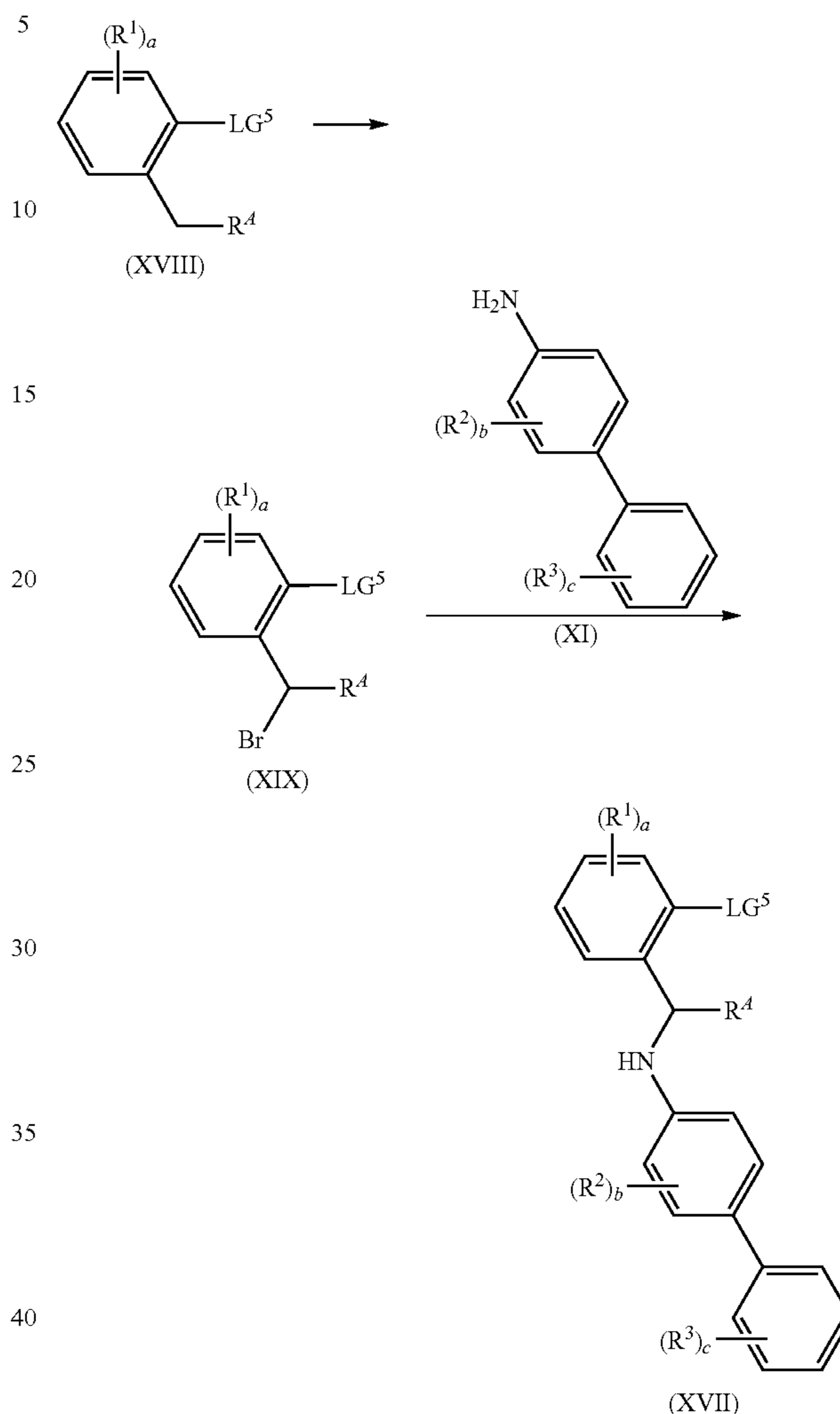
Scheme 6
