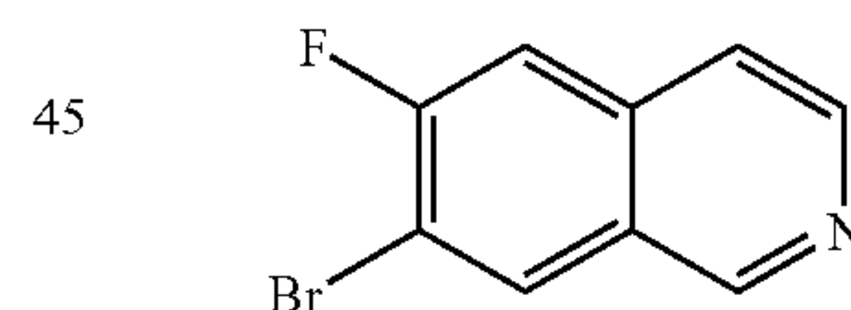
265: 6-Fluoro-7-bromo-isoquinoline
