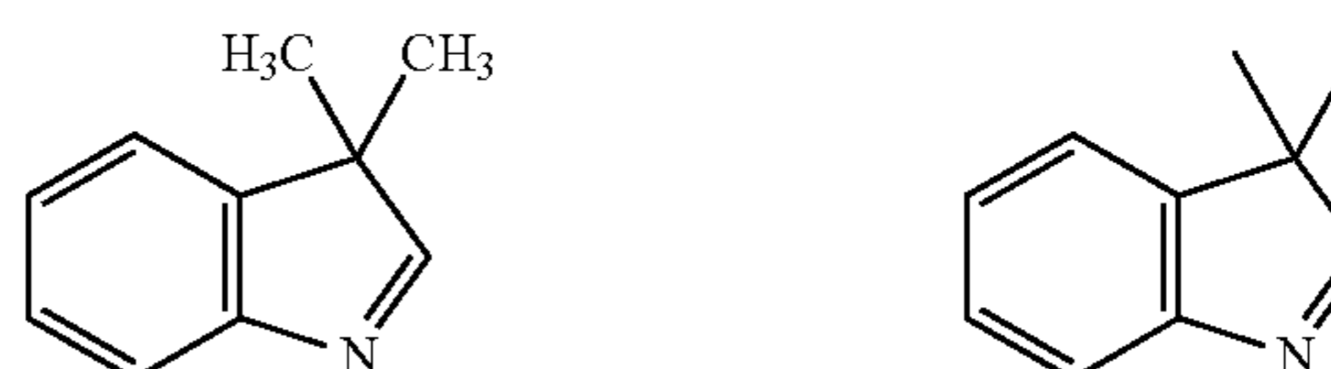
3,3-Dimethylindolenine (3,3-Dimethyl-3H-indole)
