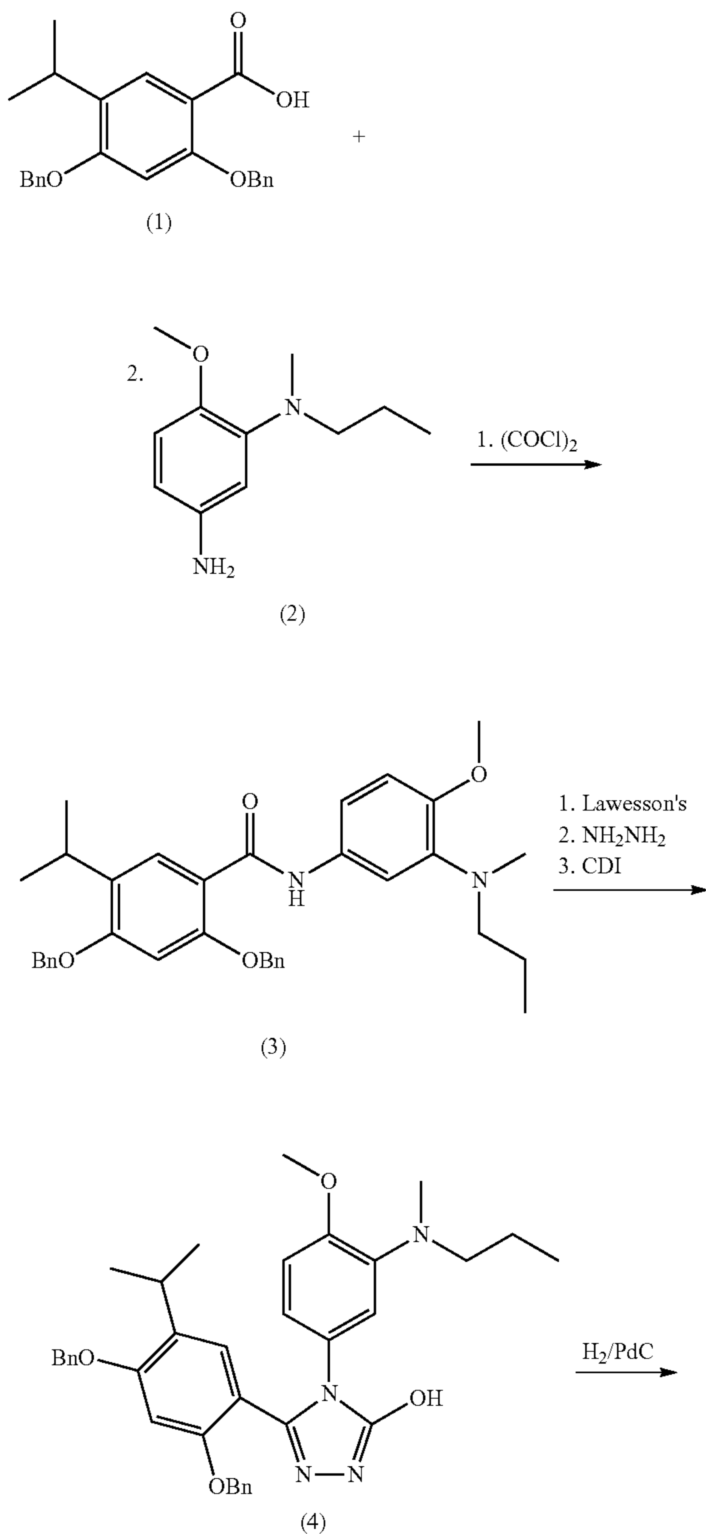
Scheme I: Scheme I: Synthesis of triazole compounds of the invention
