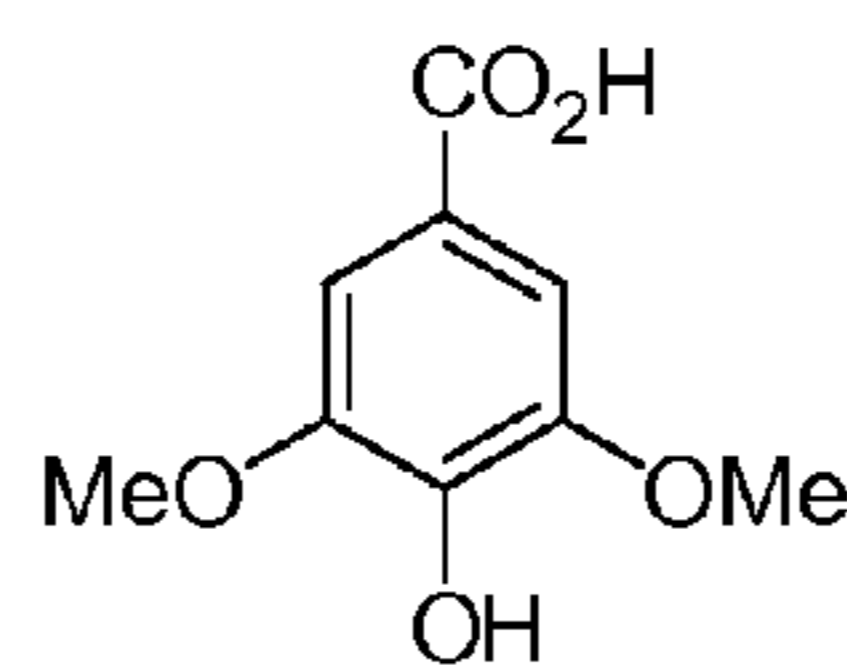
syringic acid
