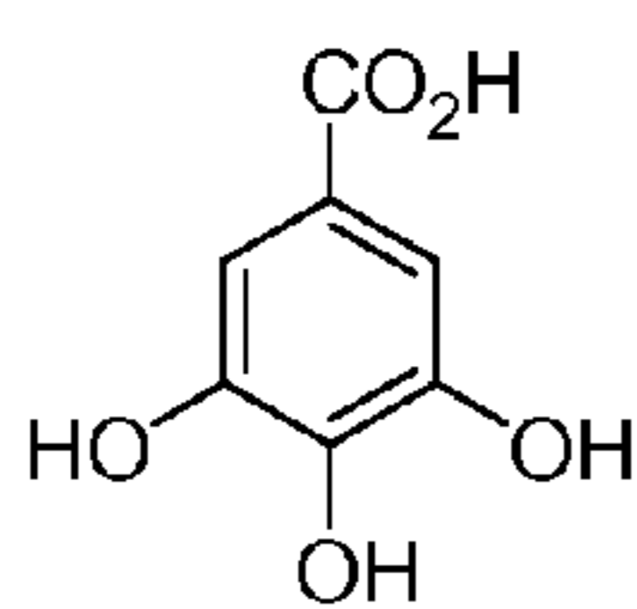
gallic acid
