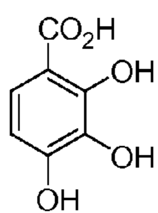
2,3,4-trihydroxybenzoic acid
