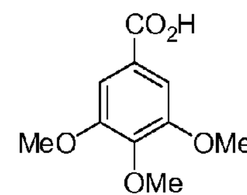
3,4,5-trimethoxybenzoic acid
