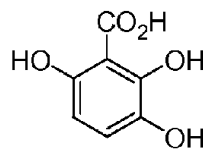
2,3,6-trihydroxybenzoic acid
