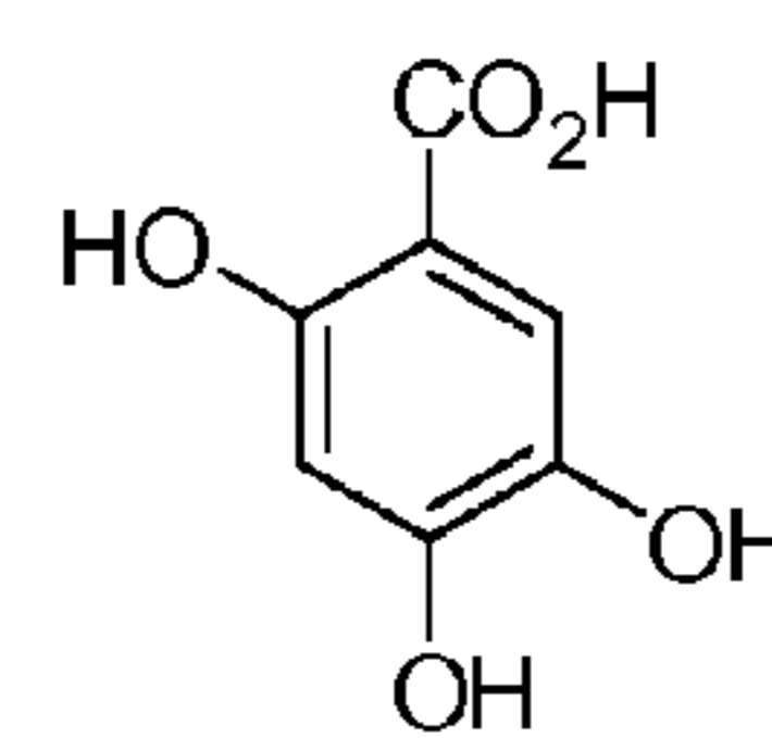
2,4,5-trihydroxybenzoic acid
