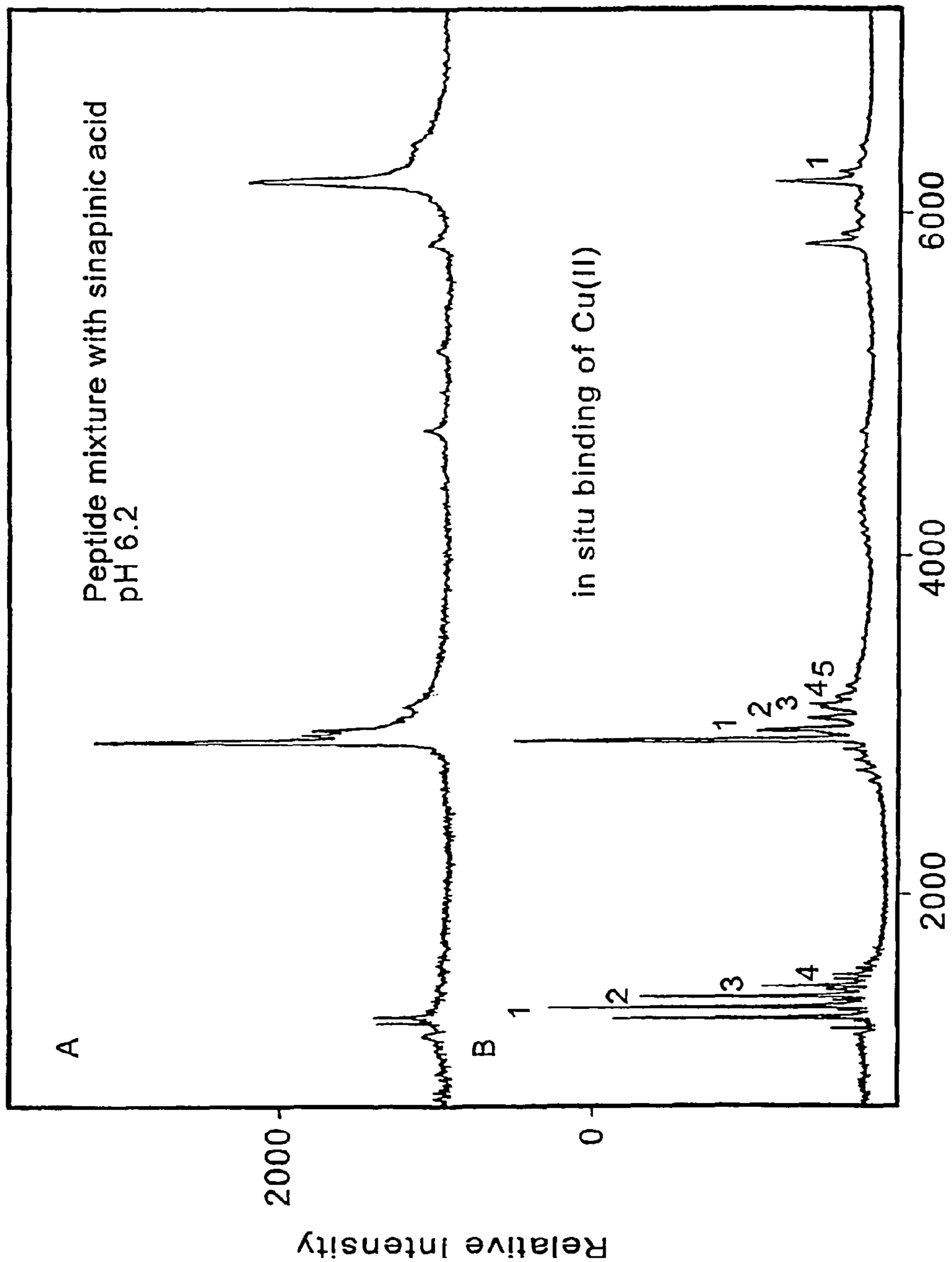
Mass/Charge (m/z)
