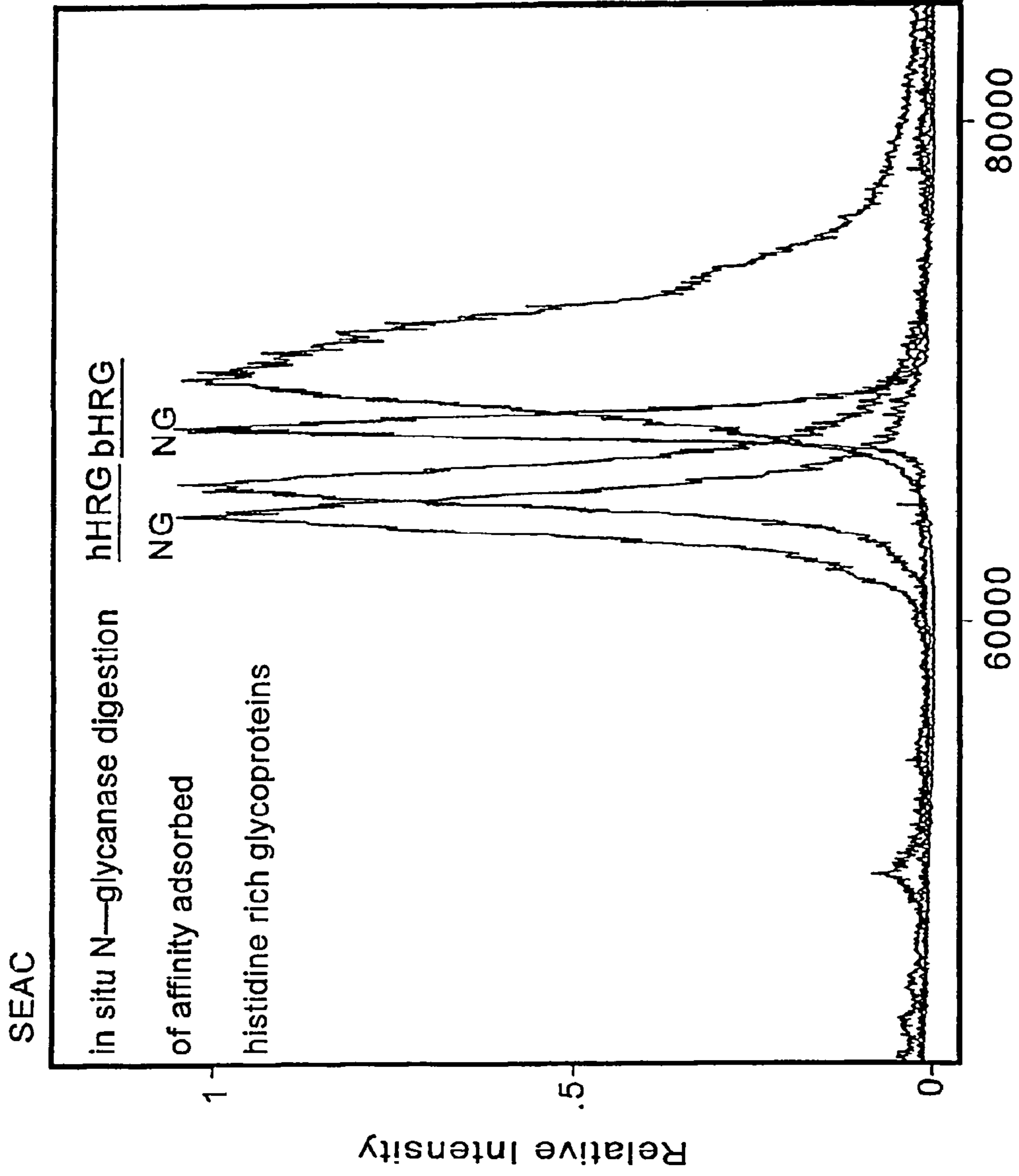
Mass/Charge (m/z)
