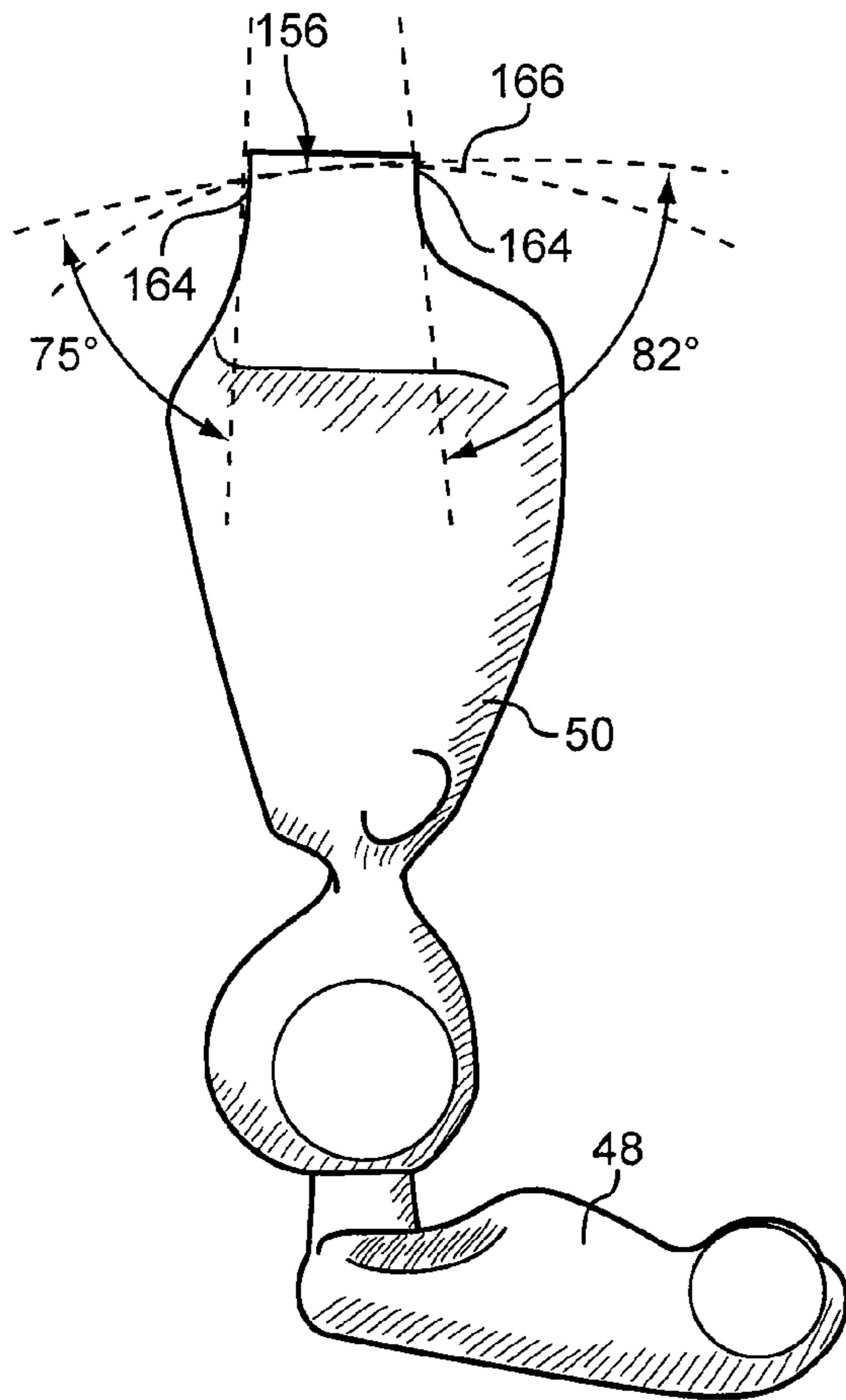
FIG. 26 PRIOR ART
