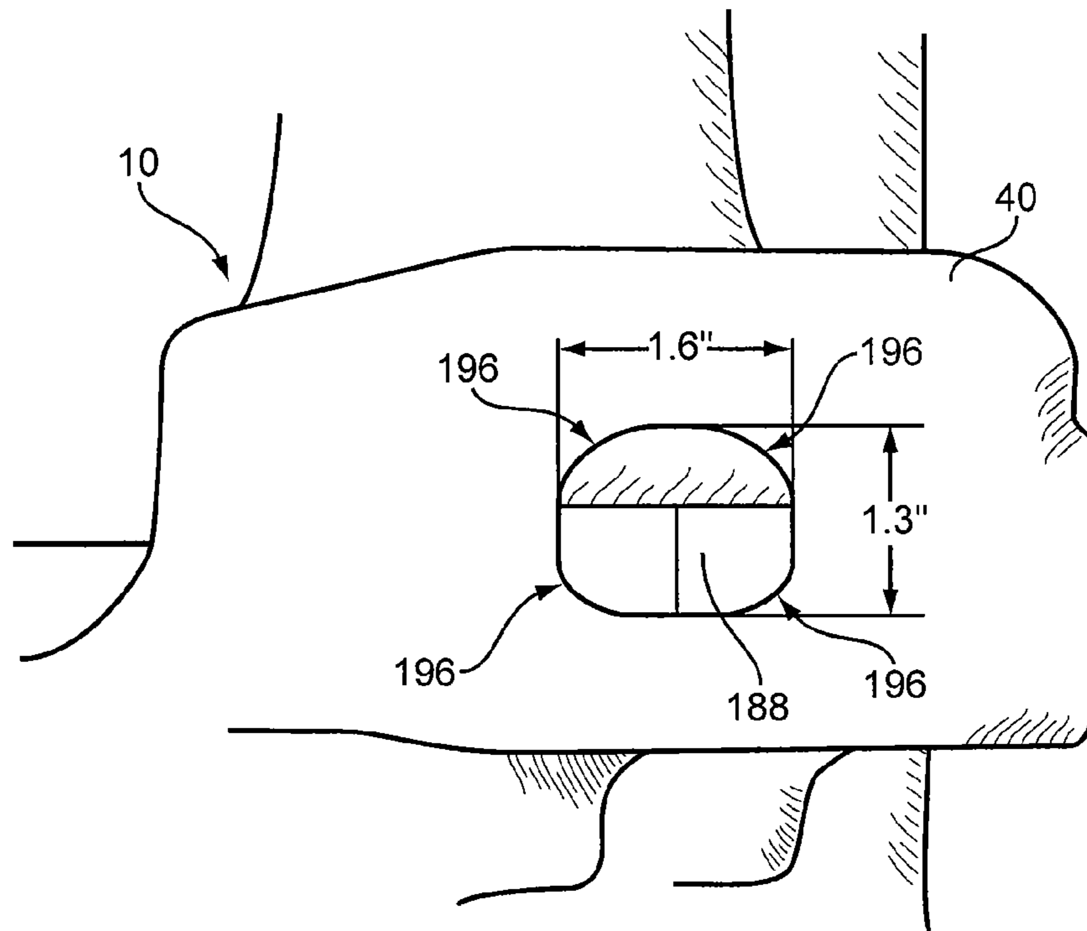
FIG. 30 PRIOR ART
