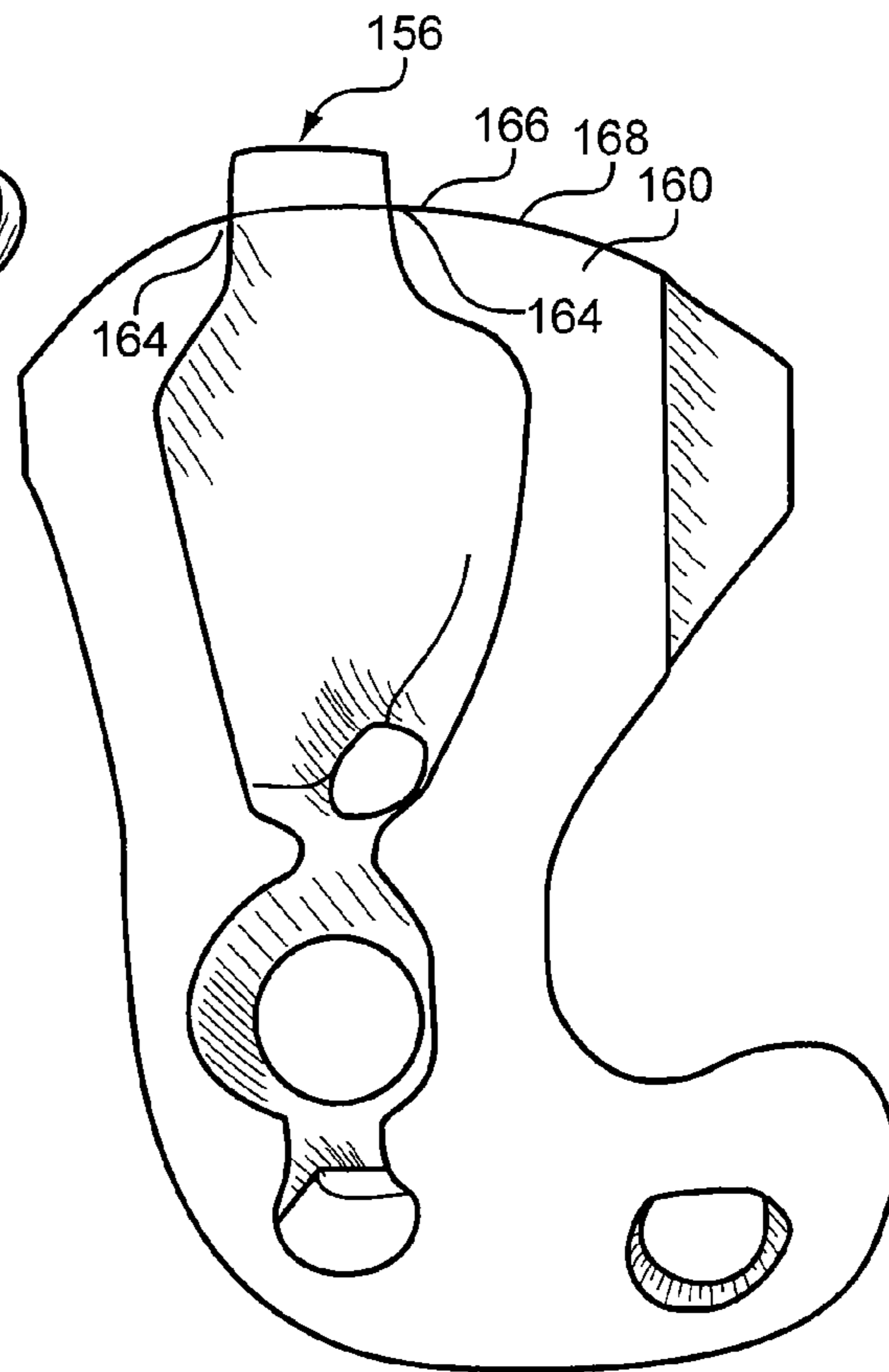
FIG. 27 PRIOR ART
