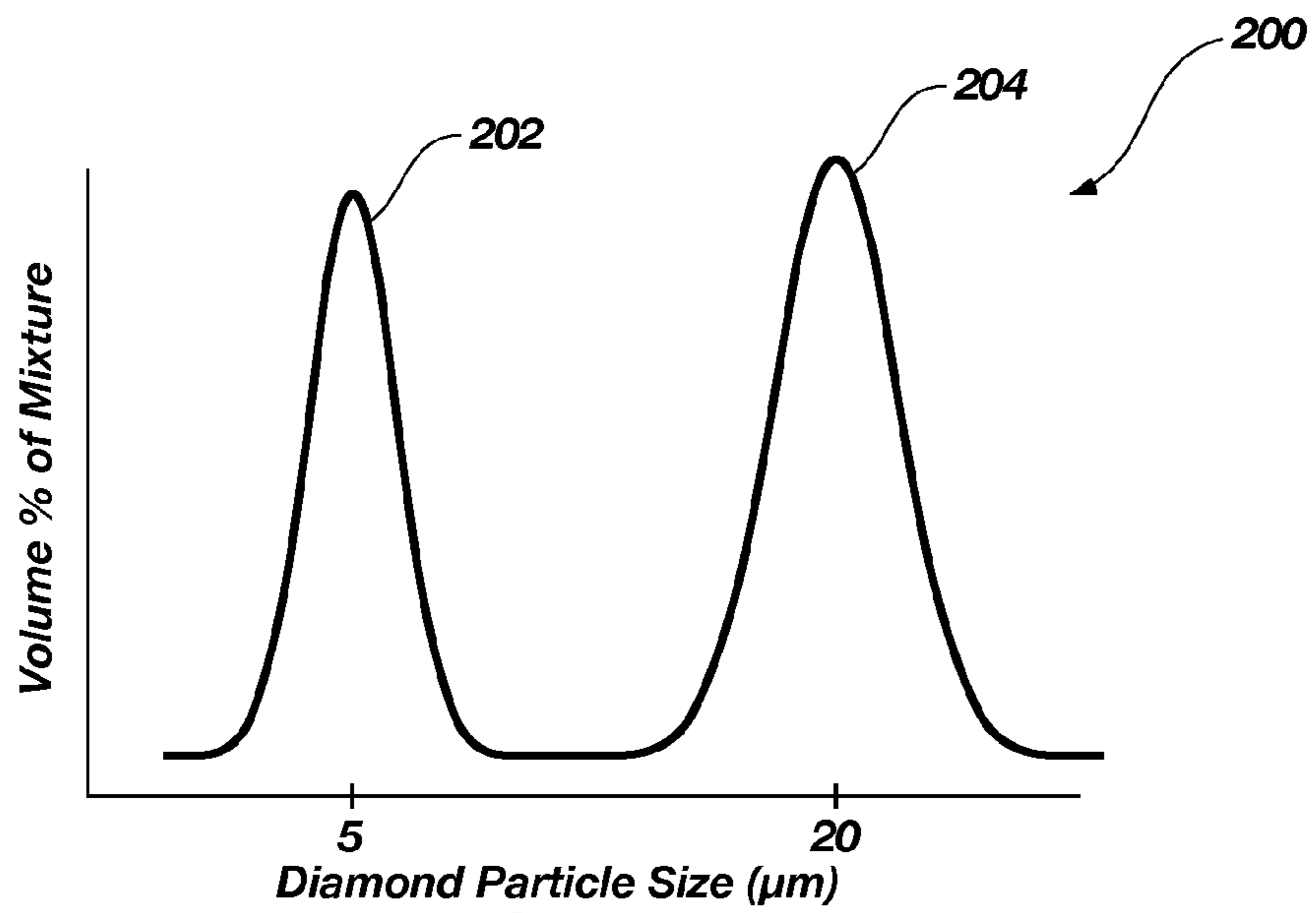
Diamond Particle Size (μm) FIG. 2A
