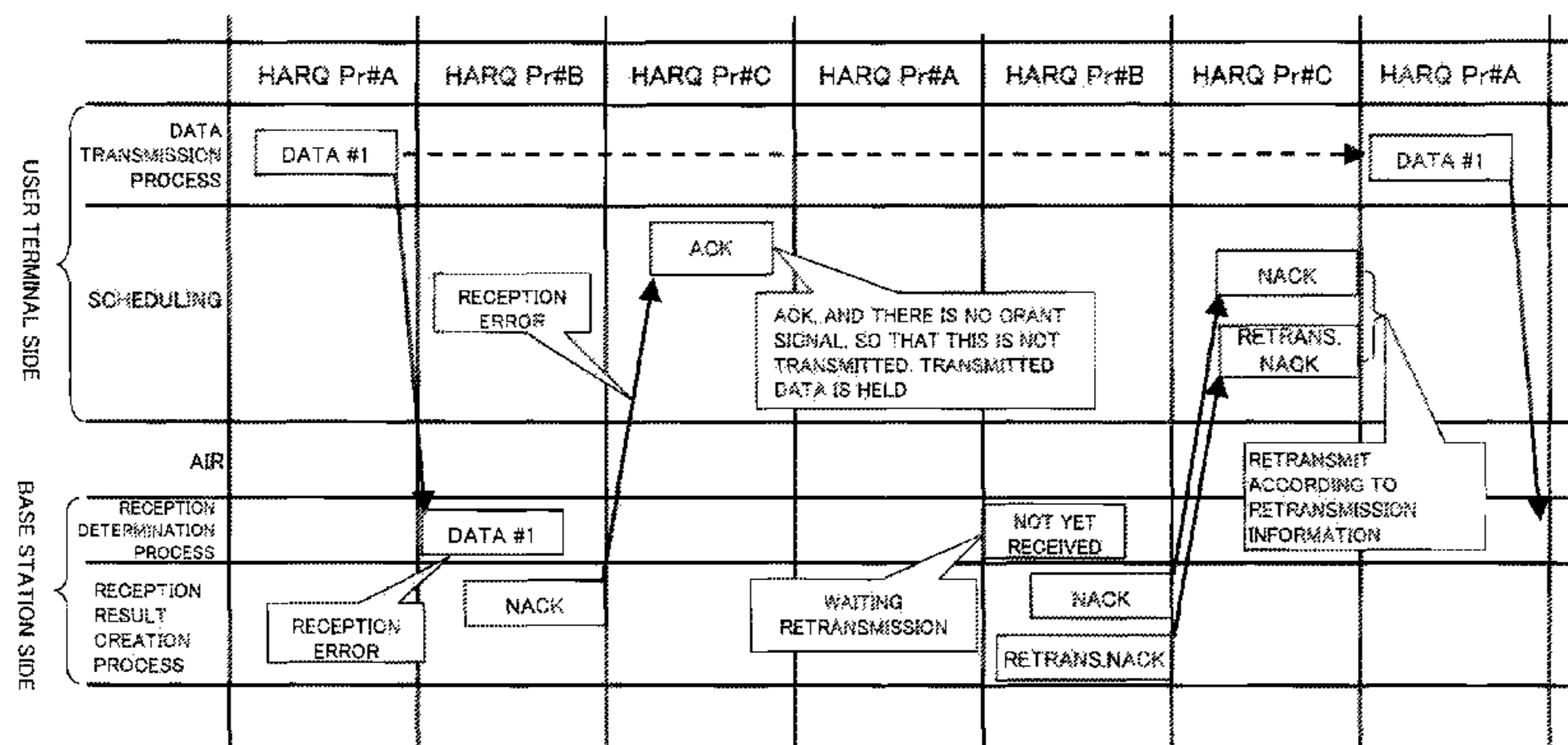
VIEW ILLUSTRATING PROCESS FLOW OF EMBODIMENT
