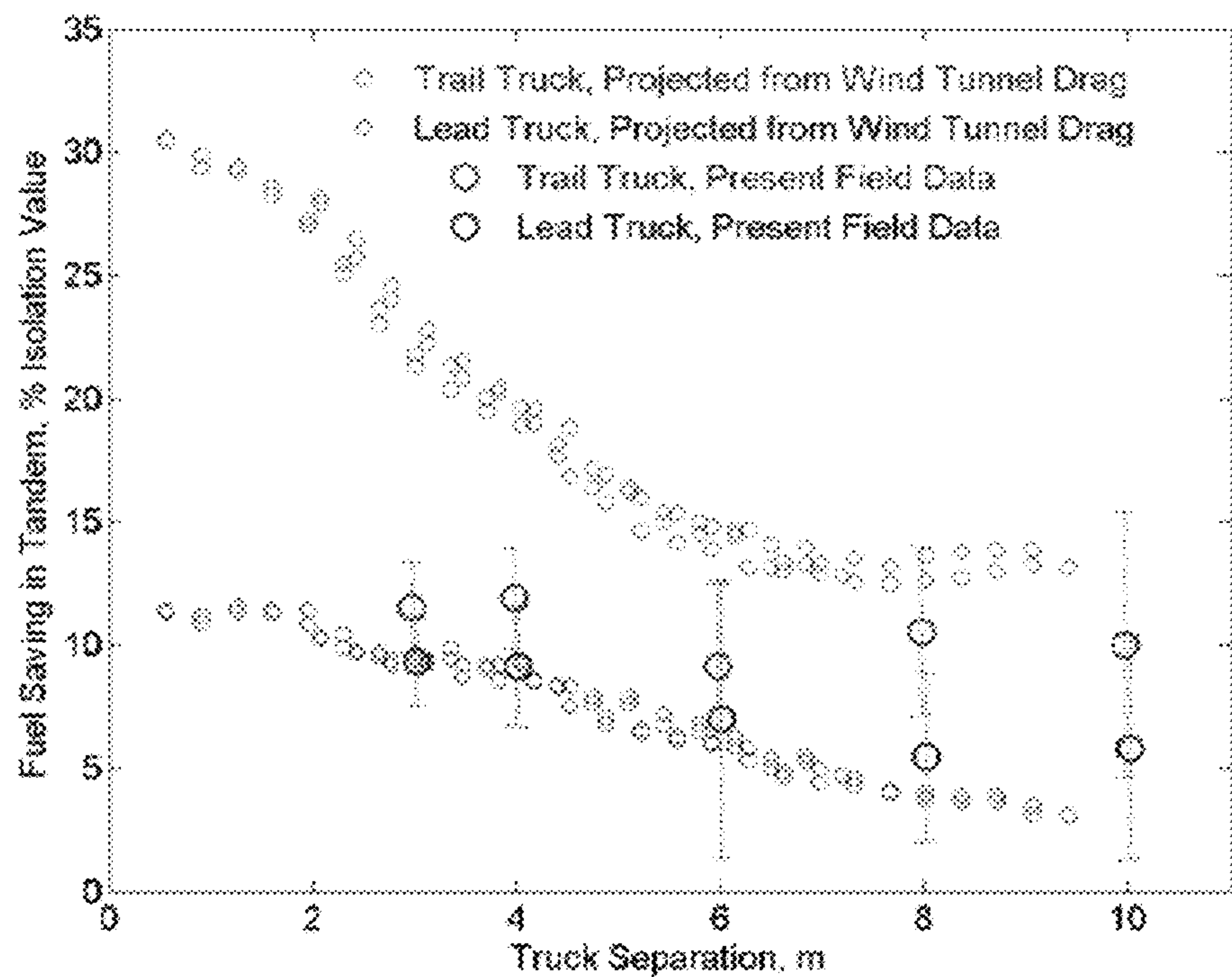
Figure 5: Fuel savings versus vehicle gap (Heavy Trucks)
