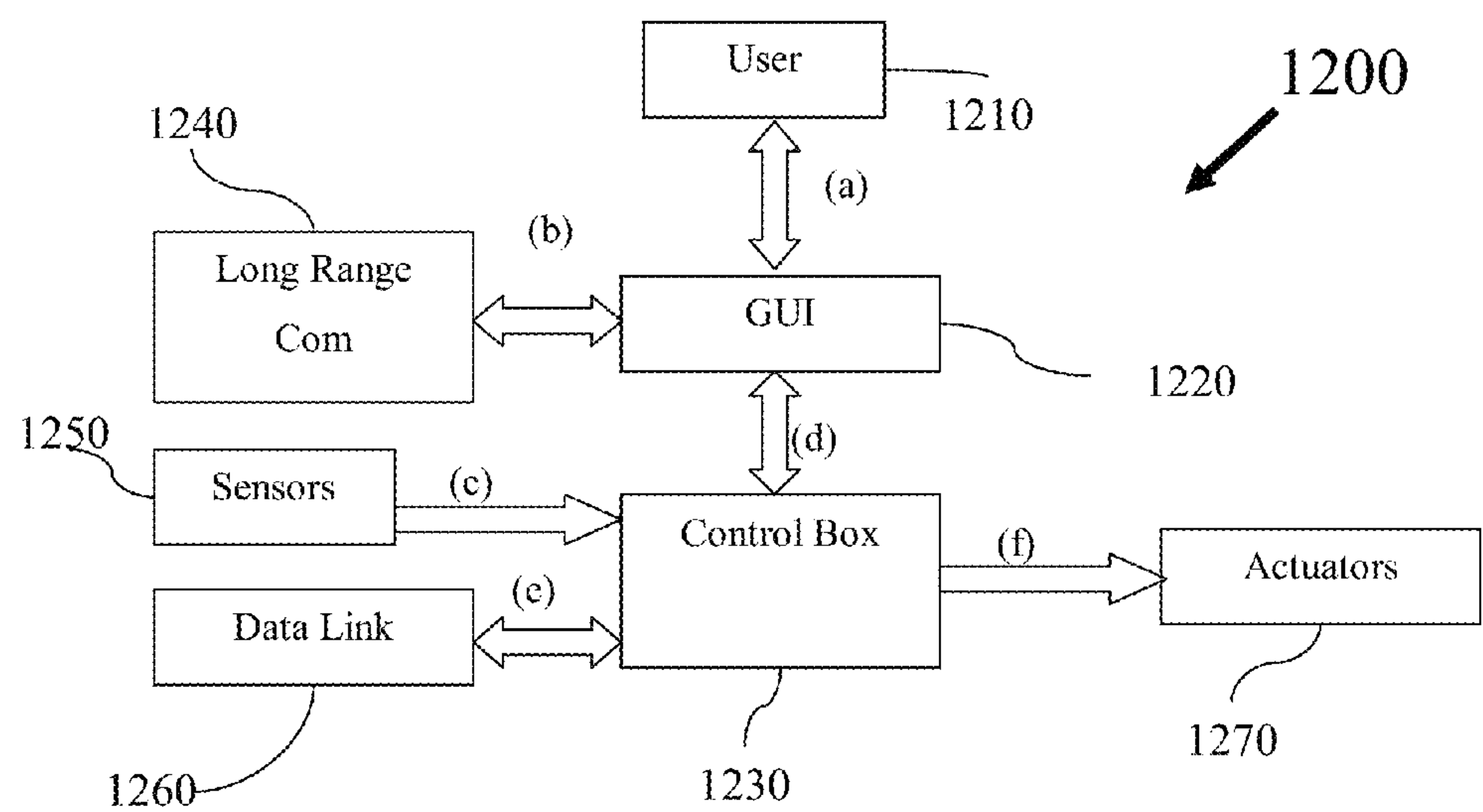
Figure 12: Simplified system block diagram
