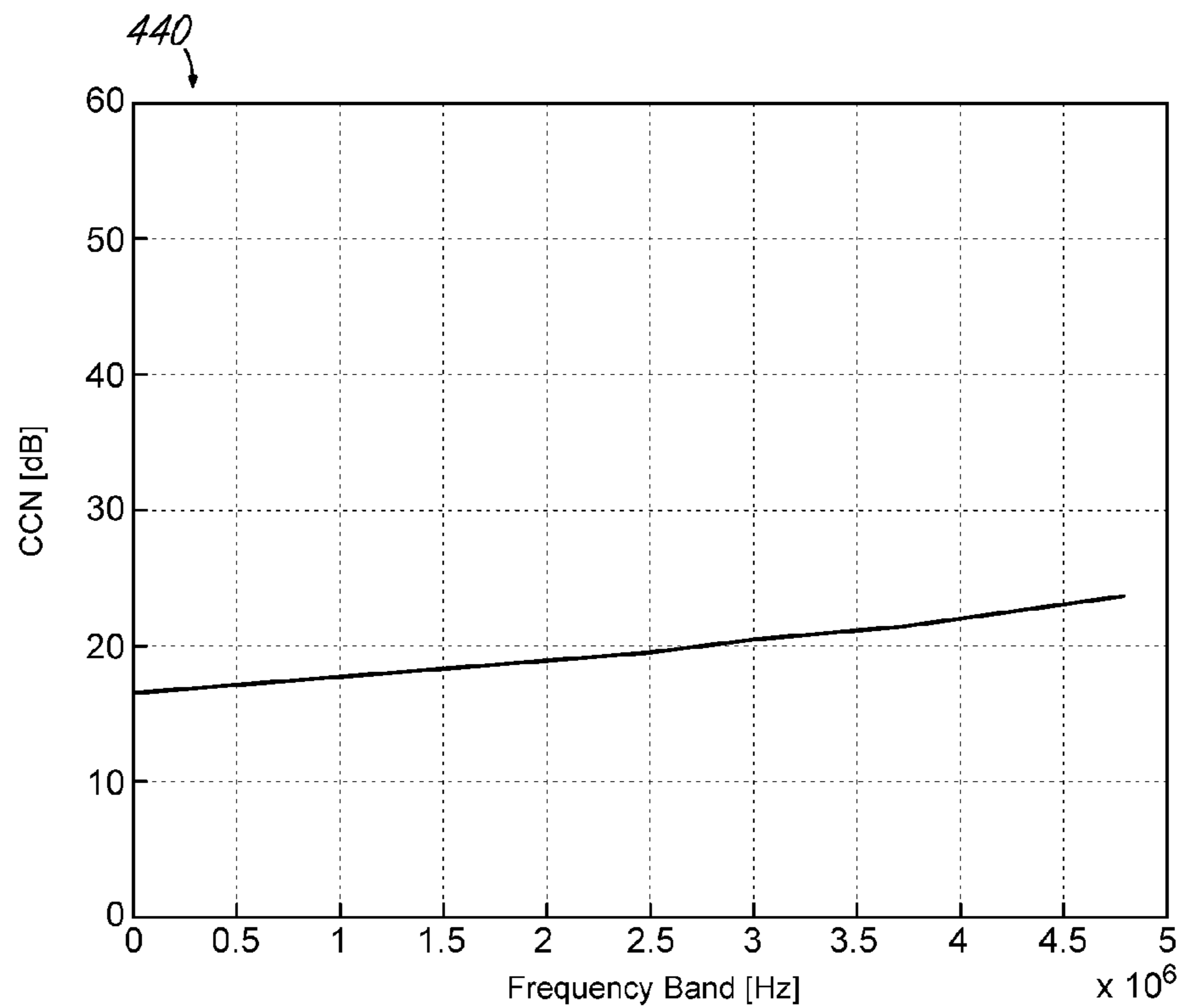
FIG.13 > 15 dB Imbalance
